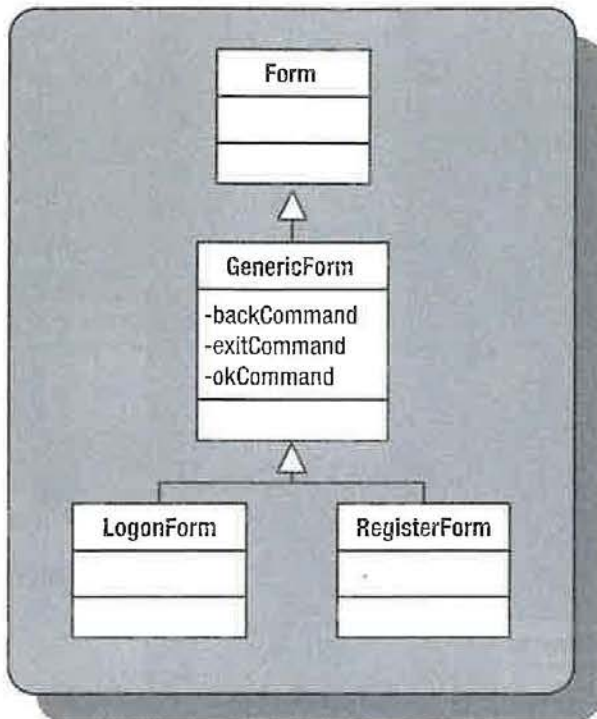
Figure 9-19. Bundling together common functionalities of a Form
