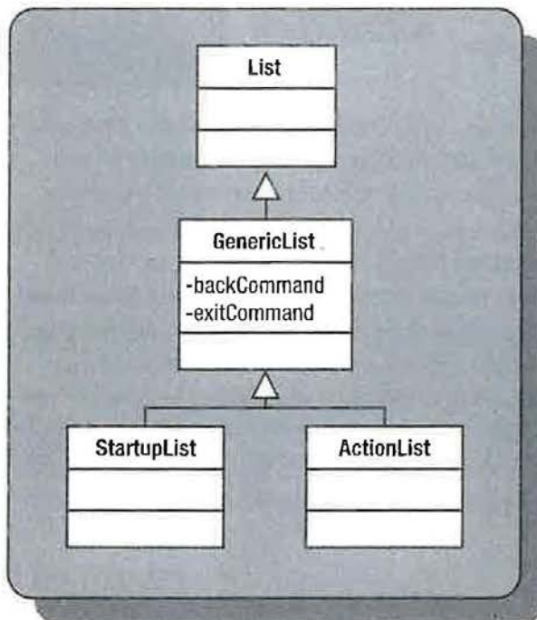
Figure 9-18. Bundling together common functionalities of a List
