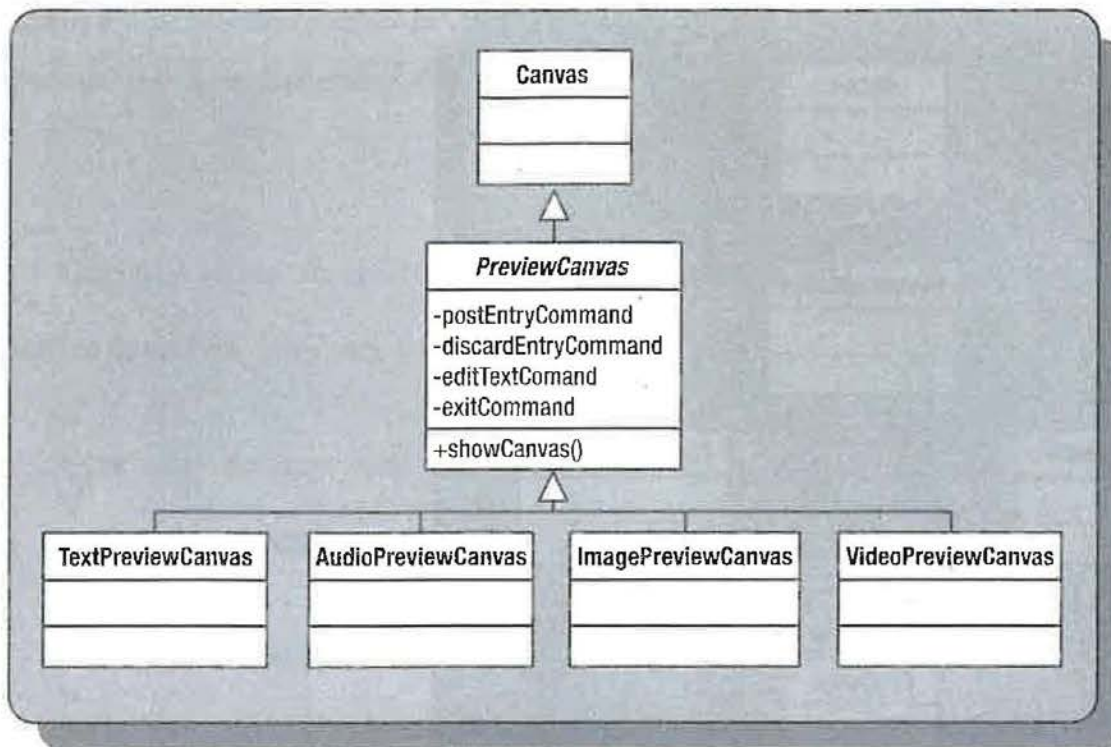
Figure 9-21. Defining the blog preview set of classes
