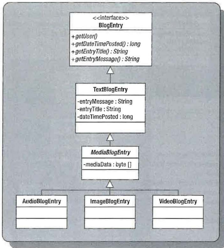
Figure 9-16. Model for the Device Blog MIDlet application
