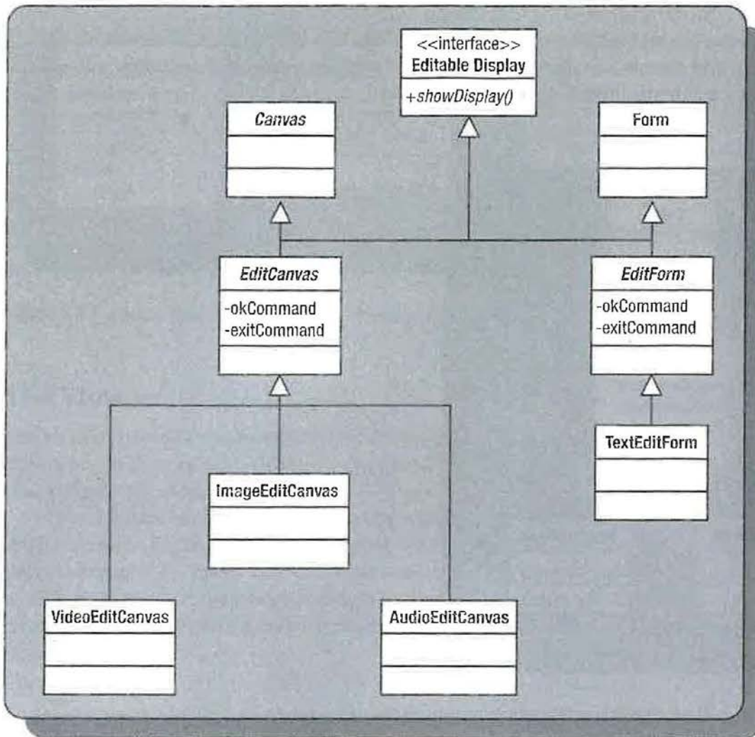
Figure 9-20. Defining the blog editing set of classes in the Device Blog MIDlet
