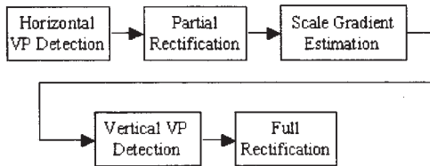
Figure 2: Algorithm description
