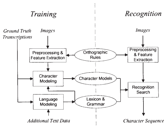
Figure 1: HMM OCR overview
