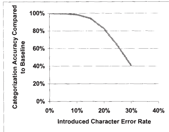
Figure 3. Reuters RCV1-V2 categorization accuracy compared to baseline versus introduced character error rate.
