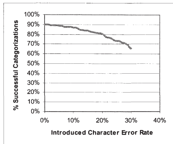
Figure 1. Reuters-21578 document categorization accuracy versus introduced character error rate.
