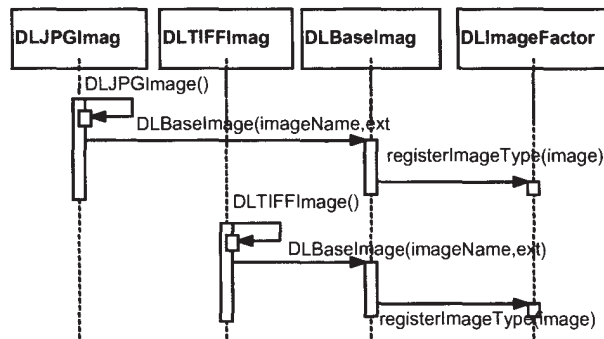
Figure 3: Image plug-in registration process
