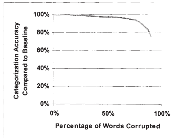
Figure 4. Reuters-21578 categorization accuracy compared to baseline versus the percentage of words corrupted.
