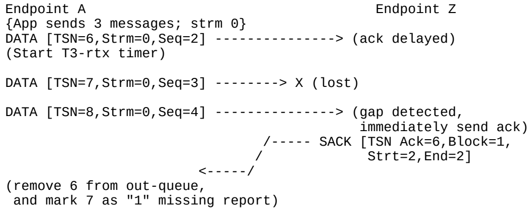
Figure 9 - Reporting a Gap using SACK
