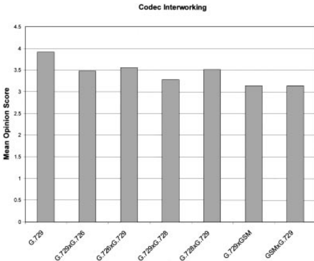
Fig. 4. Effects of transcoding.
