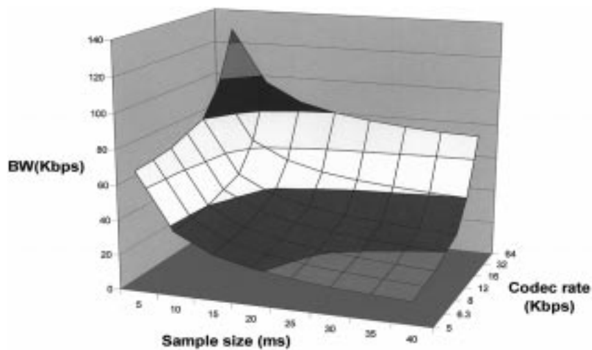
Fig. 5. The varying bands, from top to bottom, represent the following VoIP bandwidth requirements (40-byte headers): 120–140, 100–120, 80–100, 60–80, 40–60, 20–40, and 0–20.
