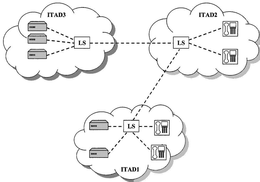
Fig. 18. TRIP architecture.
