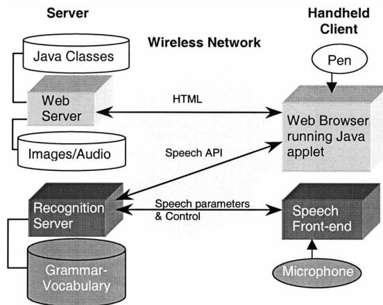
Figure 15. BBN's networked architecture for the Portable Voice Assistant, with speech recognition processing split up such that only feature extraction takes place on the handheld.
