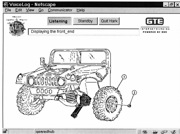
Figure 13. The BBN Portable Voice Assistant interface illustrating a diagram from the repair manual, with the system's display and spoken-language processing status confirmed at the top. Netscape Communicator browser window © 2000 Netscape Communications Corporation. Used with permission. Netscape Communications has not authorized, sponsored, endorsed, or approved this publication and is not responsible for its content.
