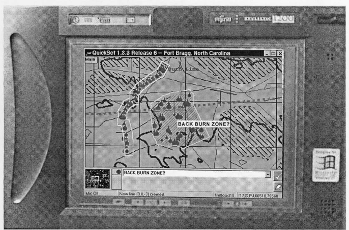
Figure 5. QuickSet system running on a wireless handheld PC, showing user-created entities on the map interface.
