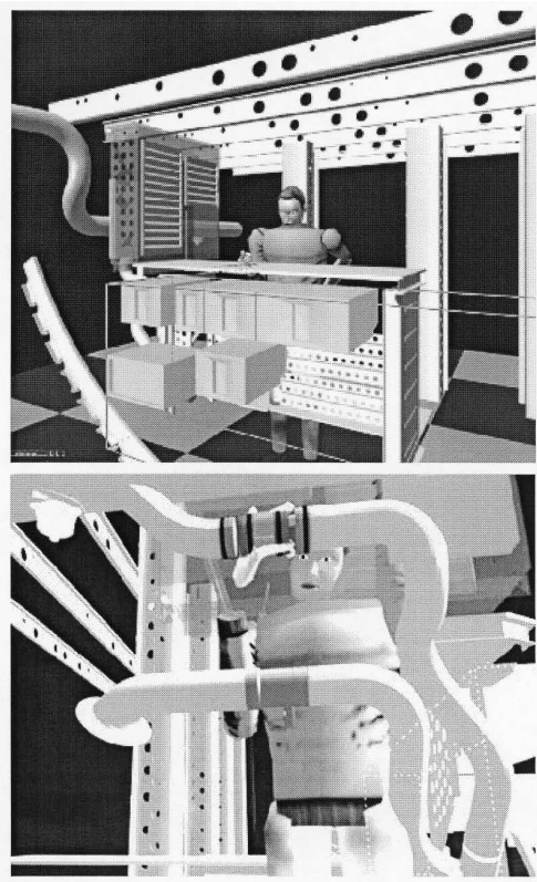
Figure 8. Boeing 777 aircraft's main equipment center.
