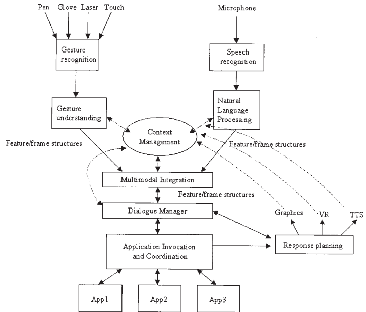
Figure 1. Typical information flow in a multimodal architecture.
