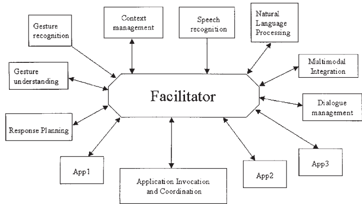
Figure 2. Facilitated multimodal architecture.
