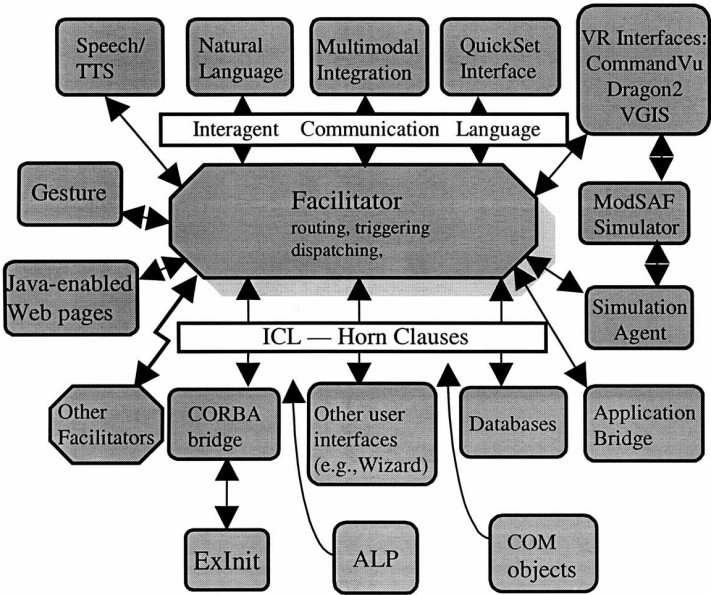
Figure 6. The OGI QuickSet system’s facilitated multiagent architecture.
