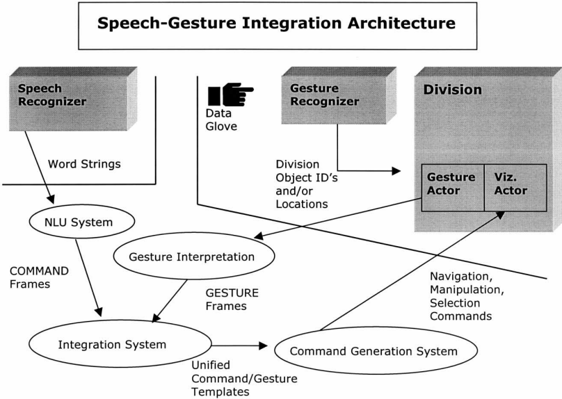
Figure 10. Boeing's integrated speech and gesture system architecture.
