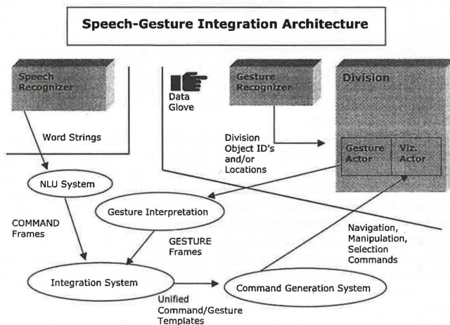
Figure 10. Boeing's integrated speech and gesture system architecture.
