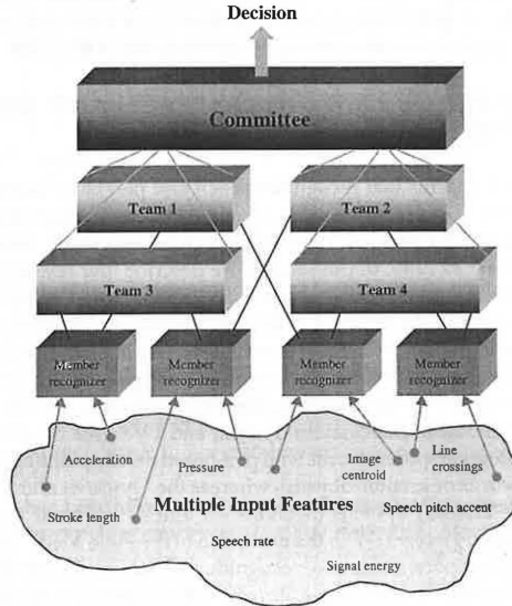
Figure 3. The three-tiered bottom-up Members-Teams-Committee architecture, composed of multiple members, multiple teams, and a decision-making committee.
