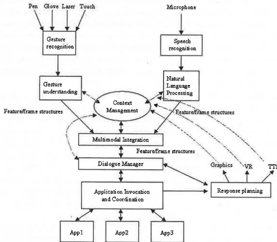
Figure 1. Typical information flow in a multimodal architecture.
