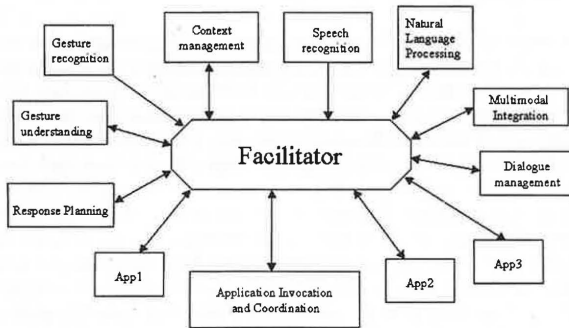
Figure 2. Facilitated multimodal architecture.
