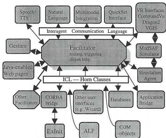
Figure 6. The OGI QuickSet system's facilitated multiagent architecture.
