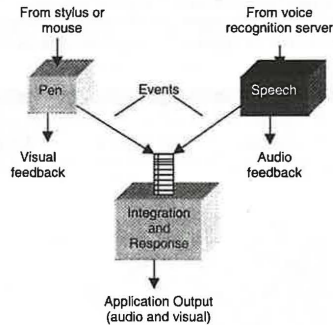
Figure 14. Data flow through the Portable Voice Assistant applet's three processing threads.
