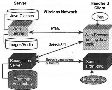
Figure 15. BBN's networked architecture for the Portable Voice Assistant, with speech recognition processing split up such that only feature extraction takes place on the handheld.
