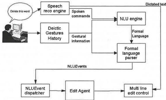
Figure 7. Architectural flow of signal and language processing in IBM's Human-Centric Word Processor system.
