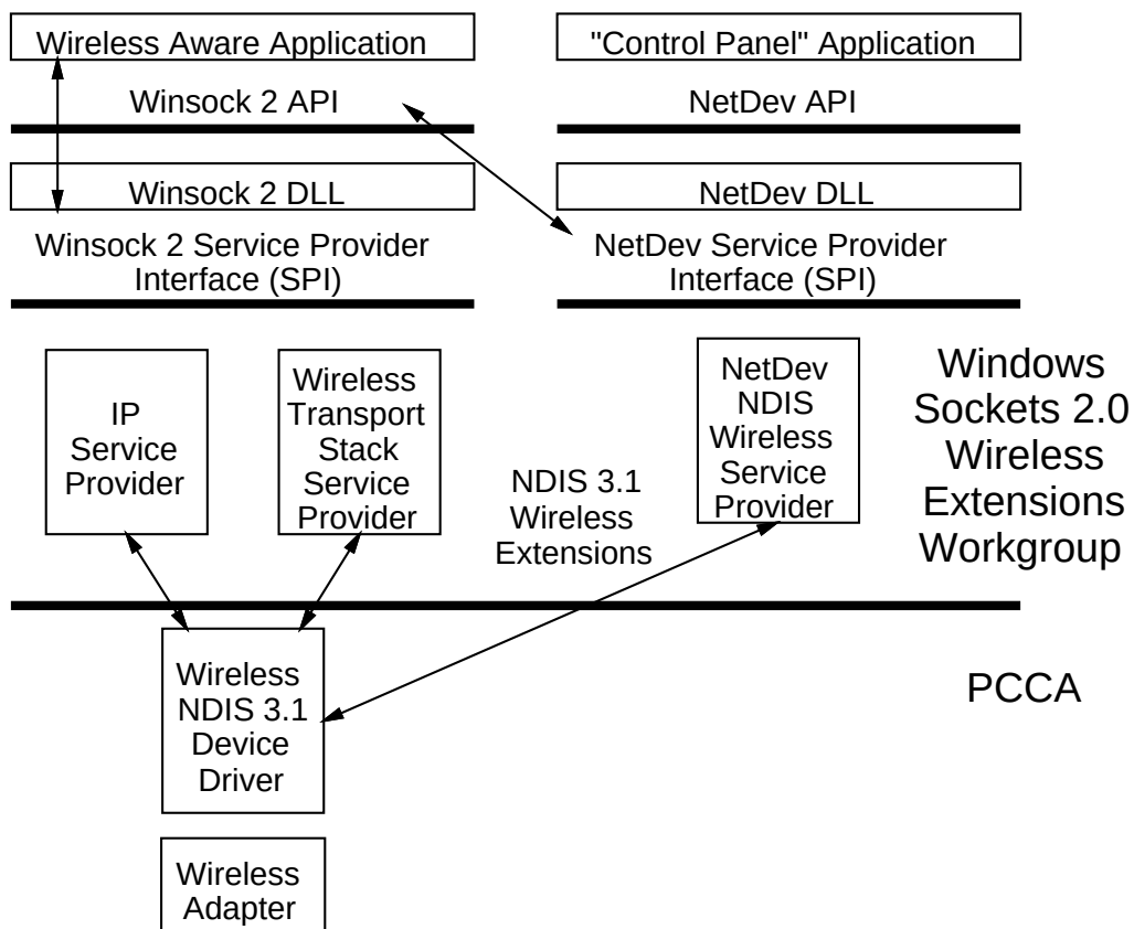
Figure 6: Structure for application and protocol stack awareness of wireless links.
