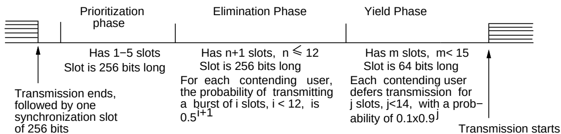
Figure 4: Channel access for HIPERLAN when the medium is sensed busy.
