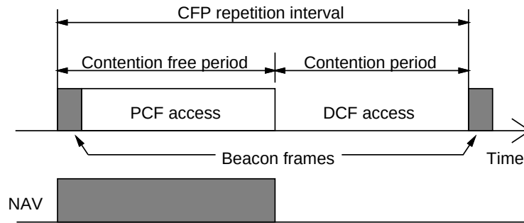
Figure 3: Alternation of contention free and contention periods.
