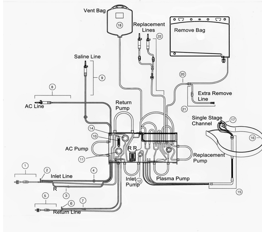
Figure 4-33. Therapeutic plasma exchange flow diagram for Spectra Optia. AC = anticoagulant, RR = return reservoir (Copyright, CaridianBCT, Inc, 2009. Used with permission.)
