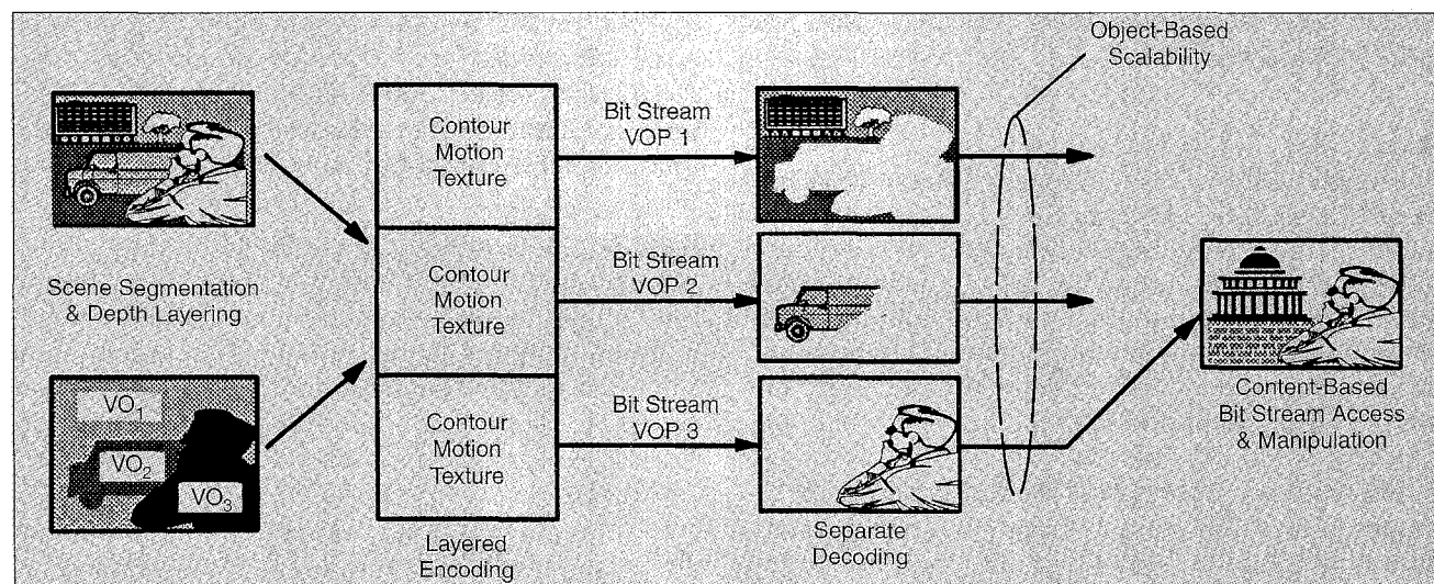
▲ 13. The "object-layered" coding approach taken by the MPEG-4 video-coding standard.
