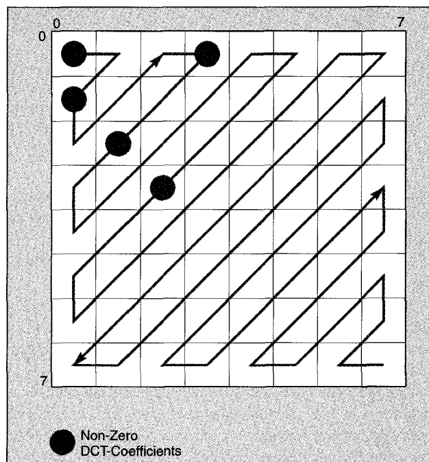
▲ 6. “Zig-zag” scanning of the quantized DCT coefficients in an 8 \times 8 block. Only the nonzero quantized DCT coefficients are encoded. The possible locations of nonzero DCT coefficients are indicated in the figure. The zig-zag scan attempts to trace the DCT coefficients according to their significance. With reference to Fig. 3, the lowest DCT-coefficient (0,0) contains most of the energy within the blocks and the energy is concentrated around the lower DCT coefficients.
