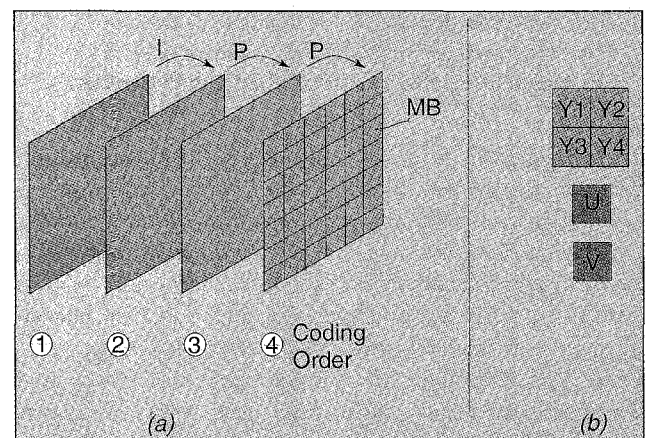
▲ 4. (a) Illustration of I-pictures (I) and P-pictures (P) in a video sequence. P-pictures are coded using motion-compensated prediction based on the nearest previous frame. Each frame is divided into disjoint "macroblocks." (b) With each macroblock, information related to four luminance blocks (Y1, Y2, Y3, Y4) and two chrominance blocks (U, V) is coded. Each block contains 8 \times 8 pels.
