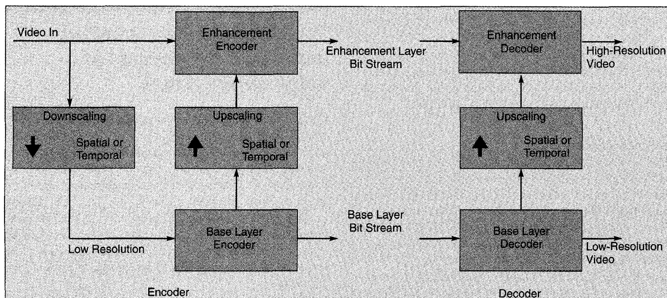
▲ 10. Scalable coding of video.
