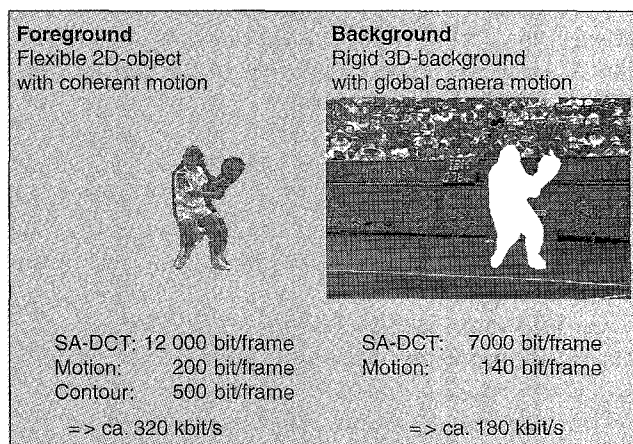
▲ 16. Foreground tennis player and separate sprite coded background.
