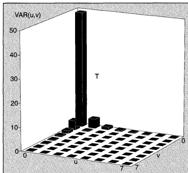
▲ 3. The figure depicts the variance distribution of DCT coefficients "typically" calculated as average over a large number of image blocks. The variance of the DCT coefficients was calculated based on the statistical model used in Fig. 1. u and v describe the horizontal and vertical image transform domain variables within the 8 \times 8 block. Most of the total variance is concentrated around the DC DCT-coefficient ( u=0, v=0 ).
