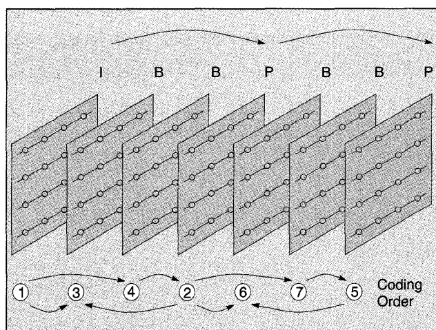
▲ 8. I-pictures (I), P-pictures (P), and B-pictures (B) used in an MPEG-1 video sequence. B-pictures can be coded using motion-compensated prediction based on the two nearest already-coded frames (either I-picture or P-picture). The arrangement of the picture coding types within the video sequence is flexible to suit the needs of diverse applications. The direction for prediction is indicated in the figure.
