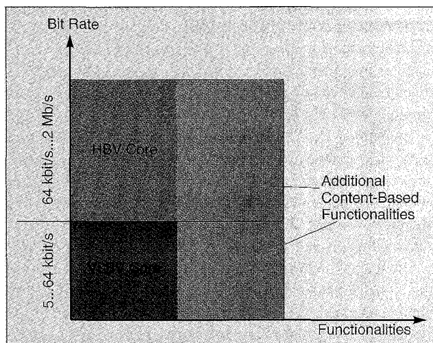
▲ 12. Structure of the MPEG-4 video-coding standard.
