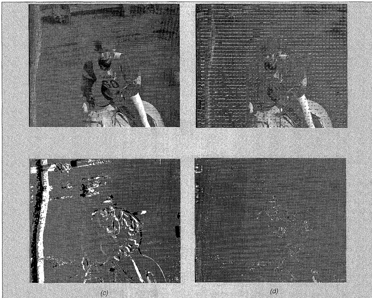
▲ 7. (a) Frame at time instance N to be coded. (b) Frame at instance N - 1 used for prediction of the content in frame N (note that the motion vectors depicted in the image are not part of the reconstructed image stored at the encoder and decoder). (c) Prediction error image obtained without using motion compensation—all motion vectors are assumed to be zero. (d) Prediction error image to be coded if motion-compensated prediction is employed.
