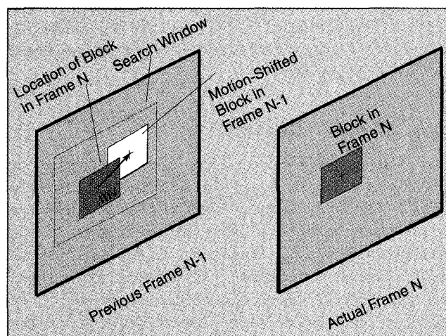
▲ 2. Block matching approach for motion compensation: One motion vector ( mv ) is estimated for each block in the actual frame, N , to be coded. The motion vector points to a reference block of the same size in a previously coded frame, N-1 . The motion-compensated prediction error is calculated by subtracting each pel in a block with its motion shifted counterpart in the reference block of the previous frame.
