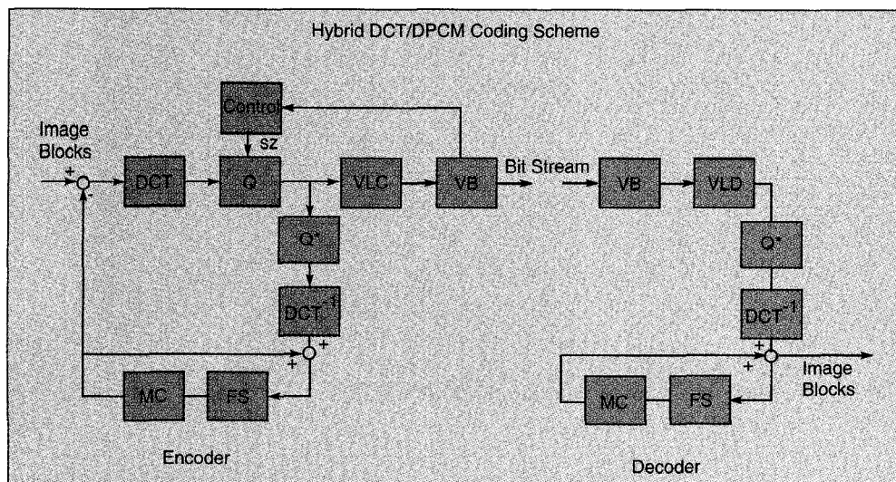
▲ 5. Block diagram of a basic hybrid DCT/DPCM encoder and decoder structure.
