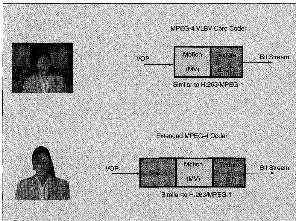
▲ 14. MPEG-4 VLBV core and the extended core coder.
