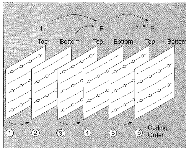
▲ 9. The concept of field pictures and an example of possible field prediction. The top fields and the bottom fields are coded separately. However, each bottom field is coded using motion-compensated interfield prediction based on the previously coded top field. The top fields are coded using motion-compensated interfield prediction based on either the previously coded top field or based on the previously coded bottom field. This concept can be extended to incorporate B-pictures.
