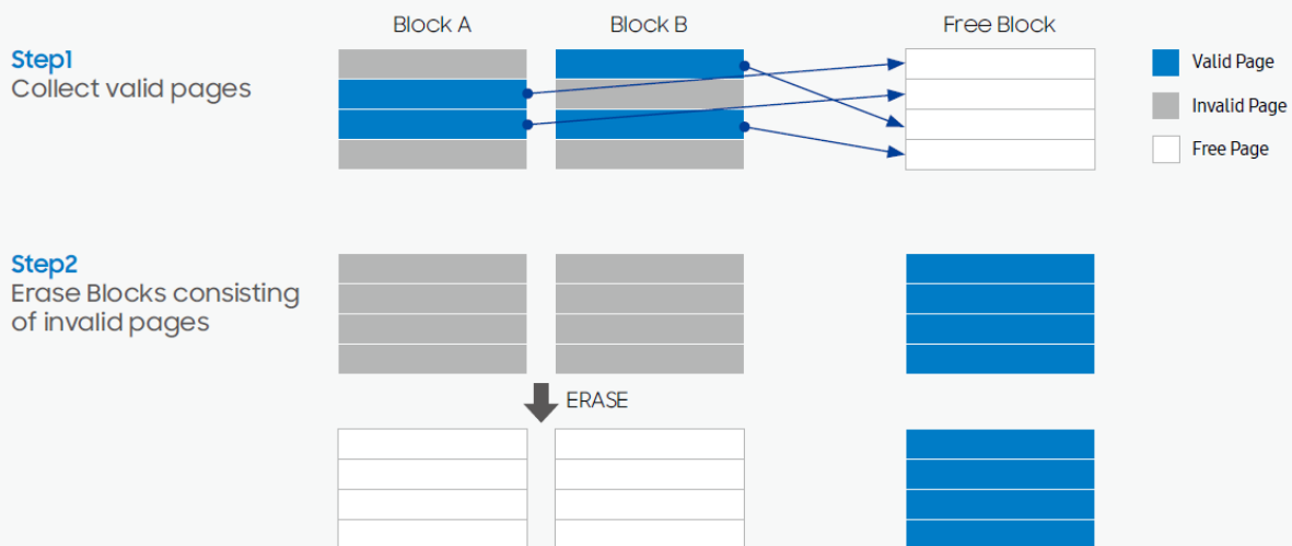
Figure 2: Garbage Collection
