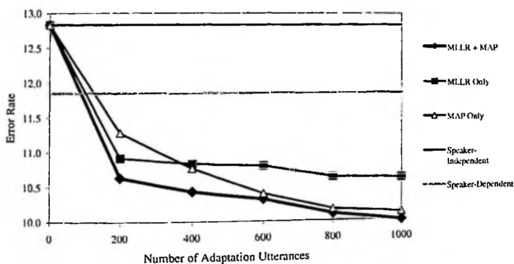
Figure 9.11 Comparison of Whisper with MLLR, MAP, and combined MLLR and MAP. The error rate is shown for a different amount of adaptation data. The speaker-dependent and speaker-independent models are also included. The speaker-dependent model was trained with 1000 sentences.
