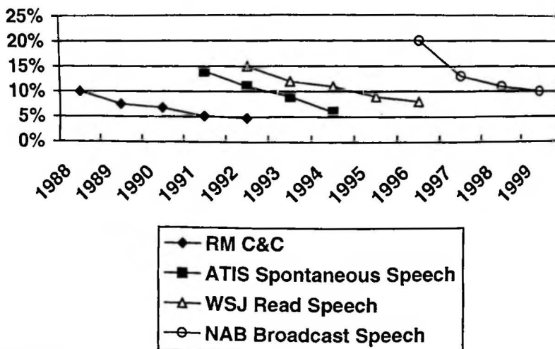
Figure 9.18 History of DARPA speech recognition word-error-rate benchmark evaluation results from 1988 to 1999. There are four major tasks: the Resource Management command and control task (RM C&C, 1000 words), the Air Travel Information System spontaneous speech understanding task (ATIS, 2000 words), the Wall Street Journal dictation task (WSJ, 20,000 words), and the Broadcast News Transcription Task (NAB, 60,000 words) [80-84].
