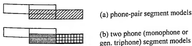
Figure 9.17 Overlapped evaluation using (a) a phone-pair segment model, or (b) back-off to two phone units when the phone-pair (e_{i-1}, e_i) segment model does not exist [47].
