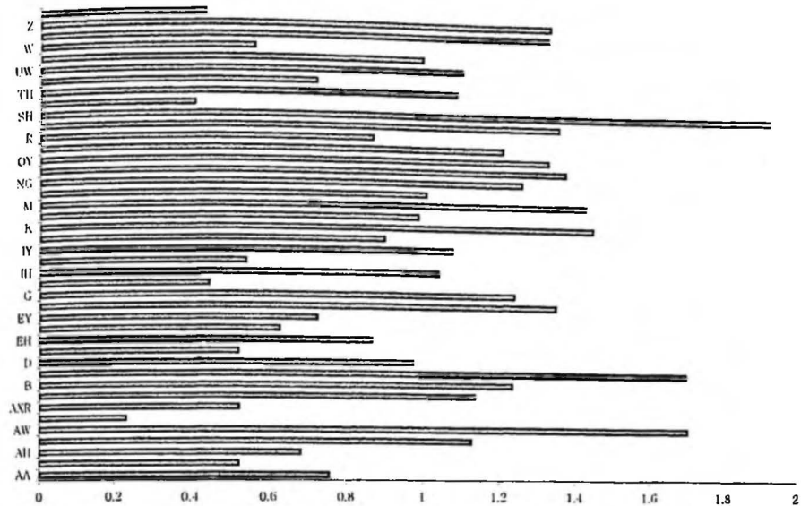
Figure 9.12 Transformation parameter a for each context-independent phone class. The weight of consonants is typically larger than that of vowels [63].
