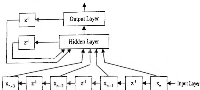
Figure 9.14 A recurrent network with contextual inputs, hidden vector feedback, and output vector feedback.
