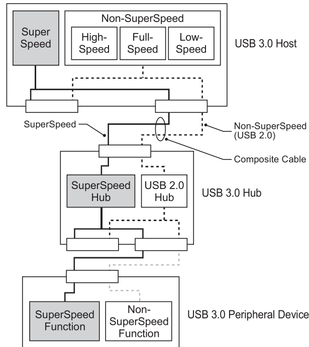
Figure 10-3. Simple USB 3.0 Topology
