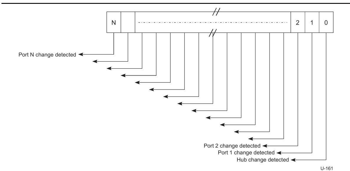
Figure 10-23. Hub and Port Status Change Bitmap
