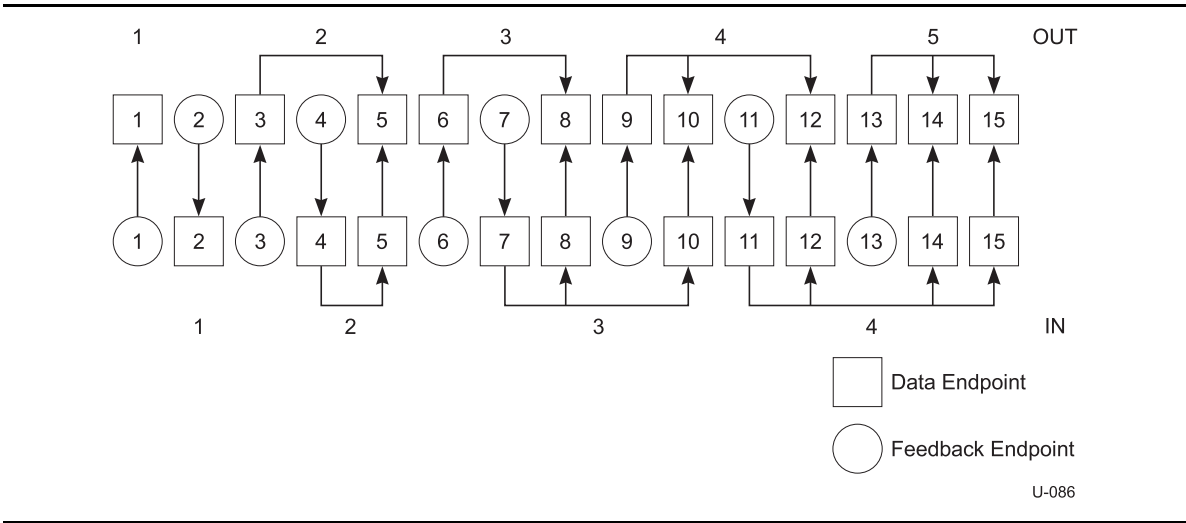
Figure 9-8. Example of Feedback Endpoint Relationships
