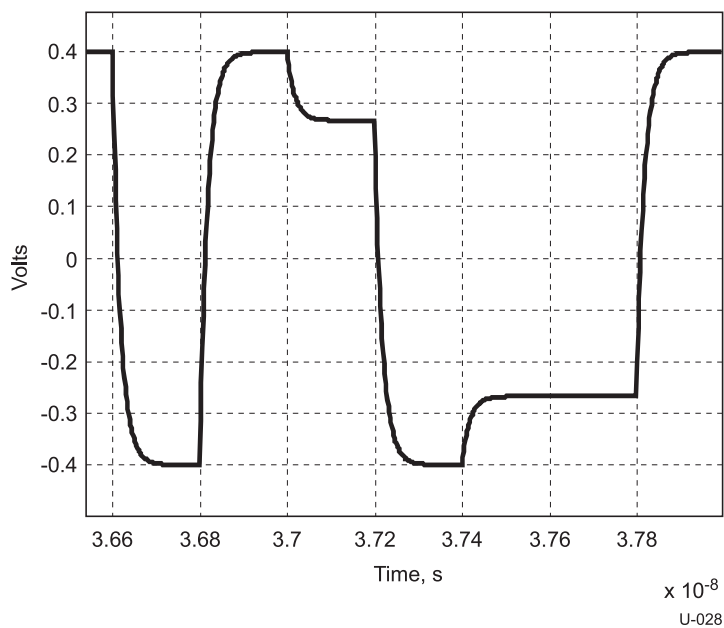
Figure 6-15. De-Emphasis Waveform
