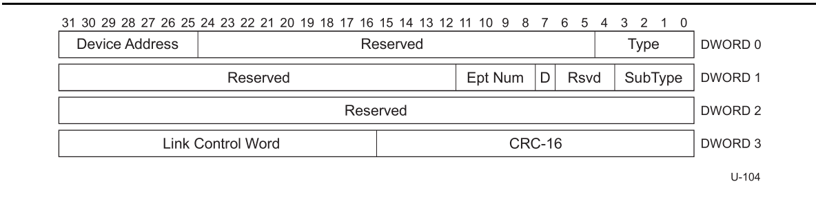
Figure 8-15. STALL Transaction Packet
