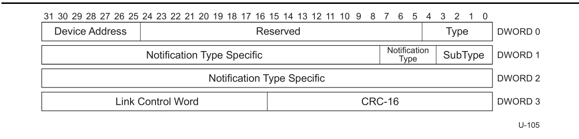
Figure 8-16. Device Notification Transaction Packet
