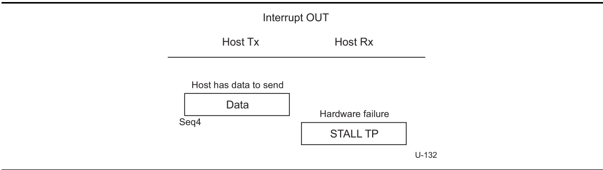
Figure 8-44. Endpoint Sends STALL TP
