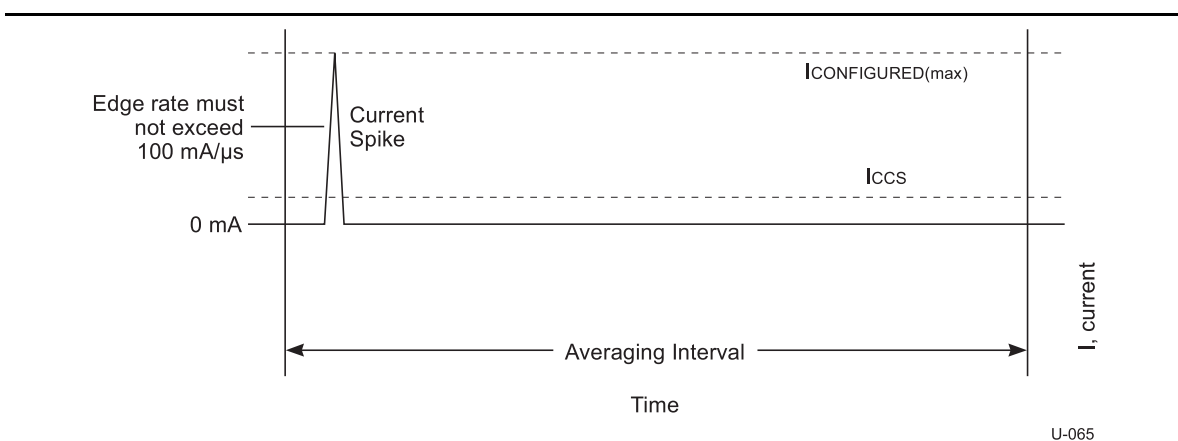
Figure 11-7. Typical Suspend Current Averaging Profile
