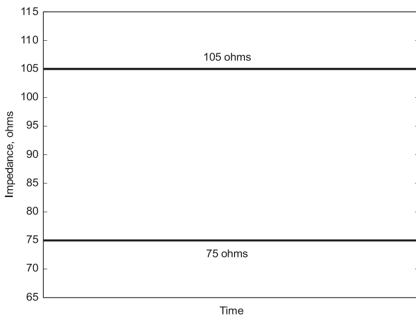
Figure 5-21. Impedance Limits of a Mated Connector
