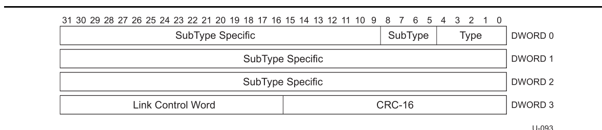
Figure 8-4. Link Management Packet Structure
