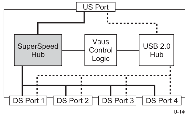
Figure 10-1. Hub Architecture
