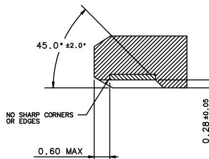
DETAIL Z
