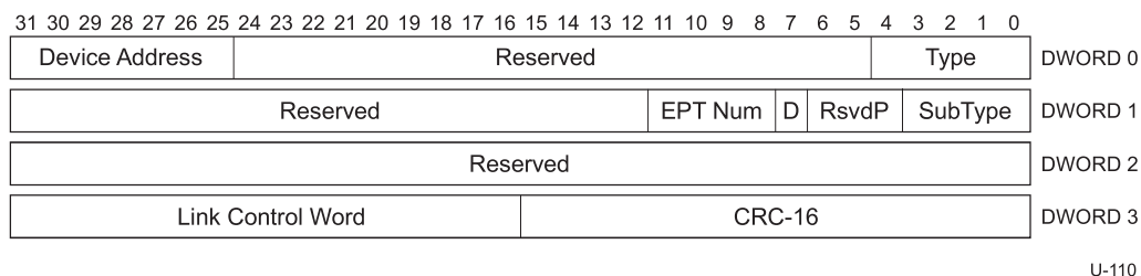
Figure 8-21. PING_RESPONSE Transaction Packet
