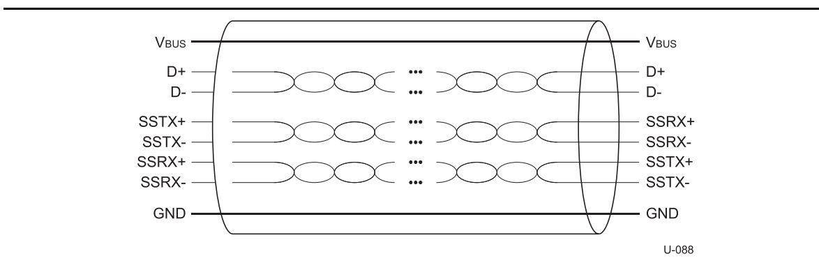
Figure 3-2. USB 3.0 Cable
