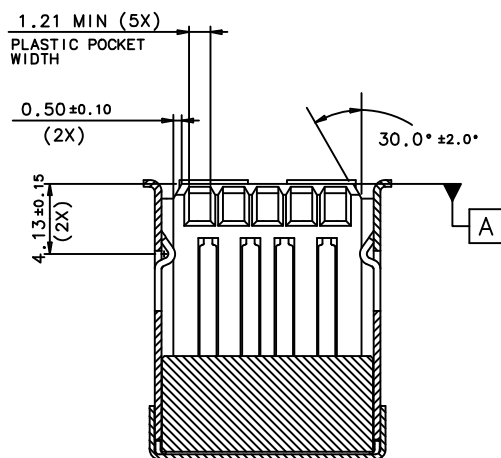
SECTION S-S
