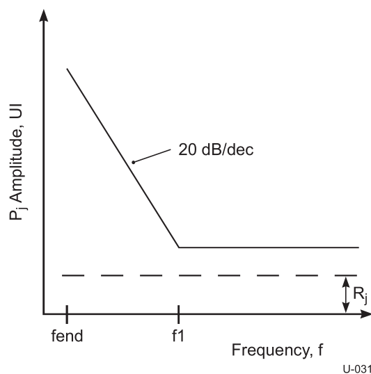
Figure 6-19. Jitter Tolerance Curve
