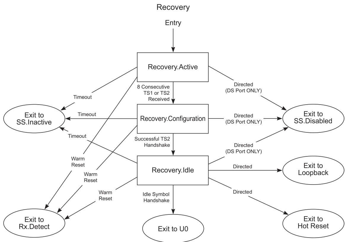
Figure 7-20. Recovery Substate Machine
