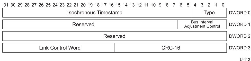
Figure 8-23. Isochronous Timestamp Packet
