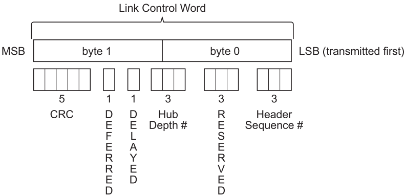
Figure 7-6. Link Control Word
