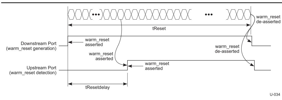
Figure 6-22. Example of Warm Reset Out of U3
