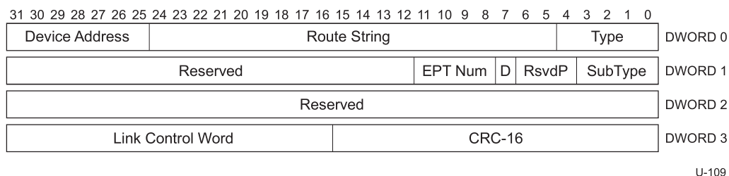
Figure 8-20. PING Transaction Packet
