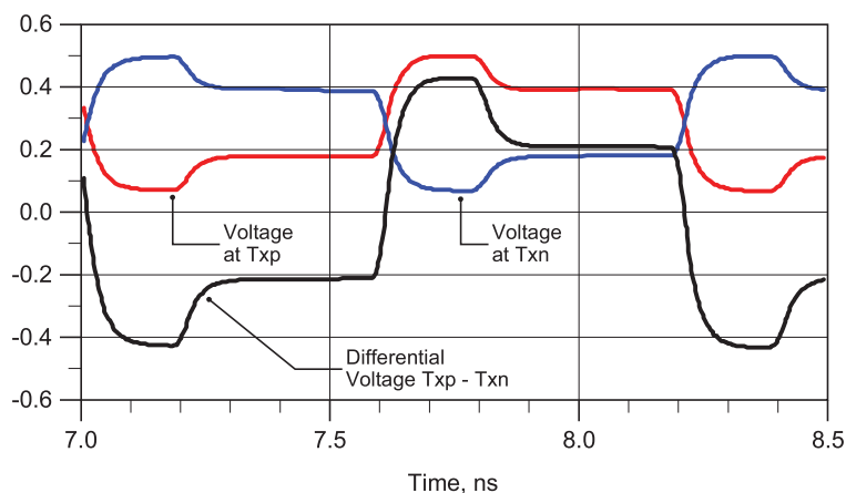
Figure 6-12. Single-ended and Differential Voltage Levels
