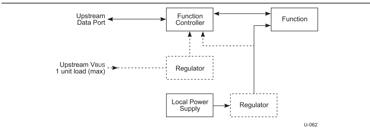
Figure 11-4. Self-powered Function
