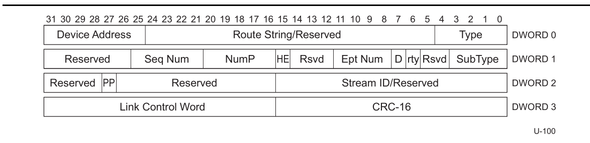
Figure 8-11. ACK Transaction Packet
