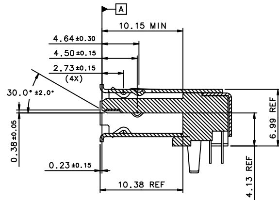
SECTION H-H
