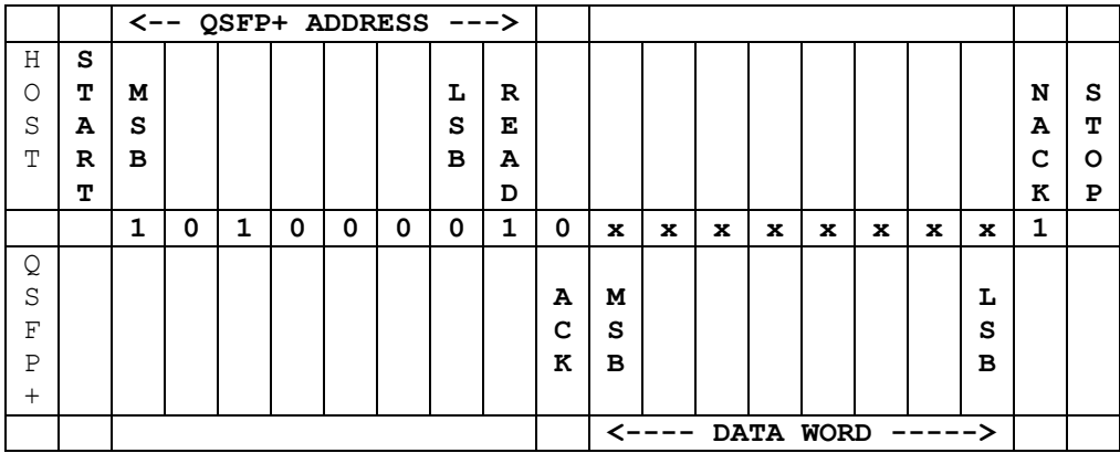
Figure 24 - QSFP+ Current Address Read Operation
