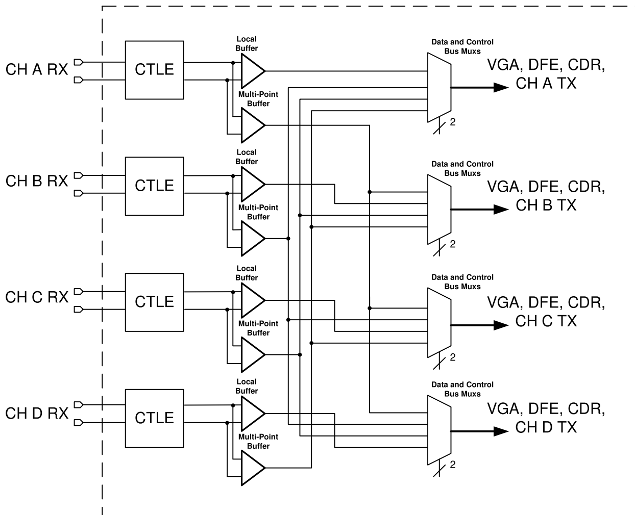
Figure 3. Cross Point Switch Diagram
