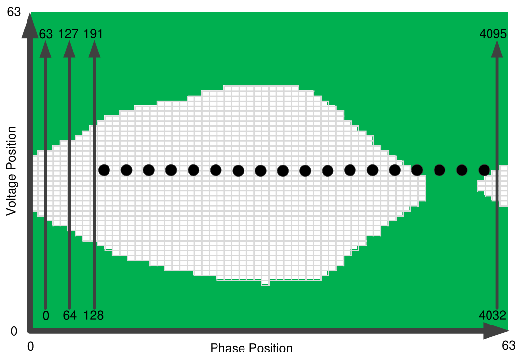
Figure 4. EOM Full Eye Capture Readout
