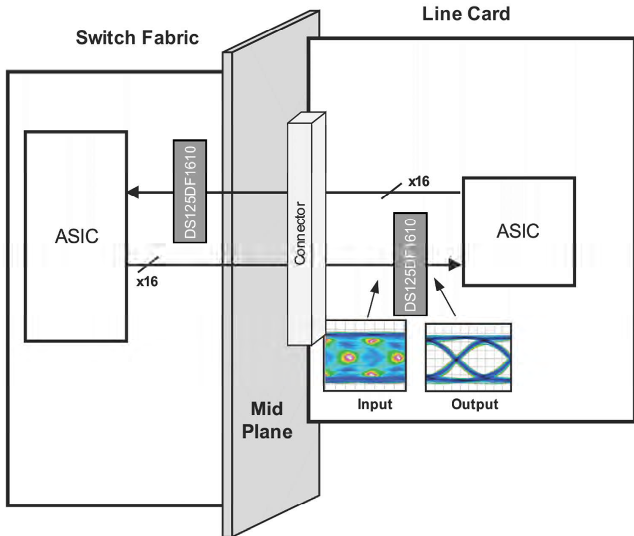
Figure 5. DS125DF1610 Example Application
