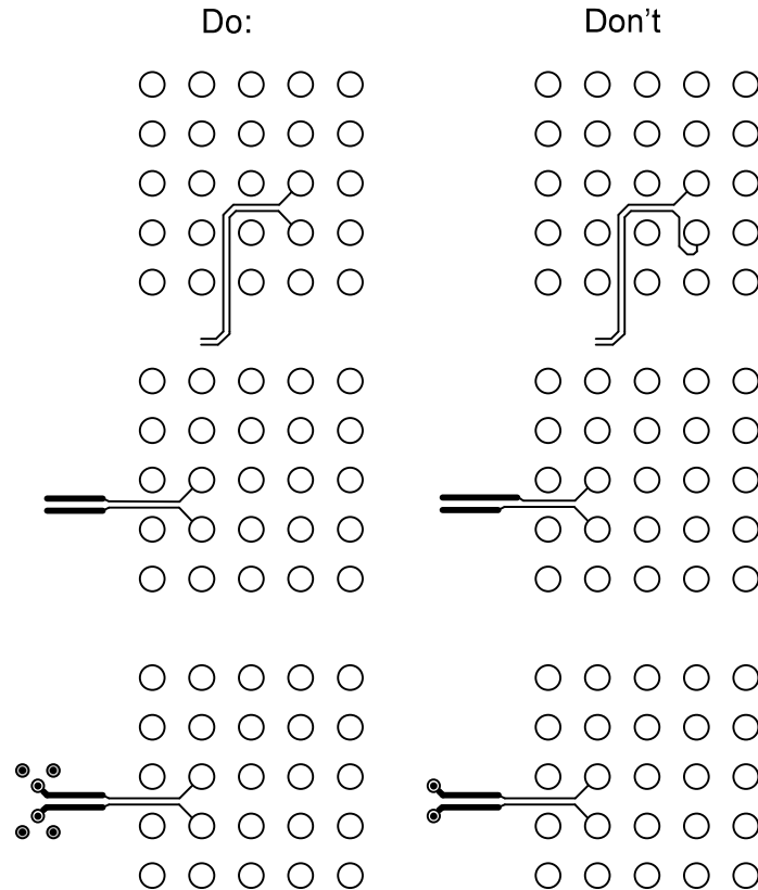
Figure 10. Layout Guidelines
