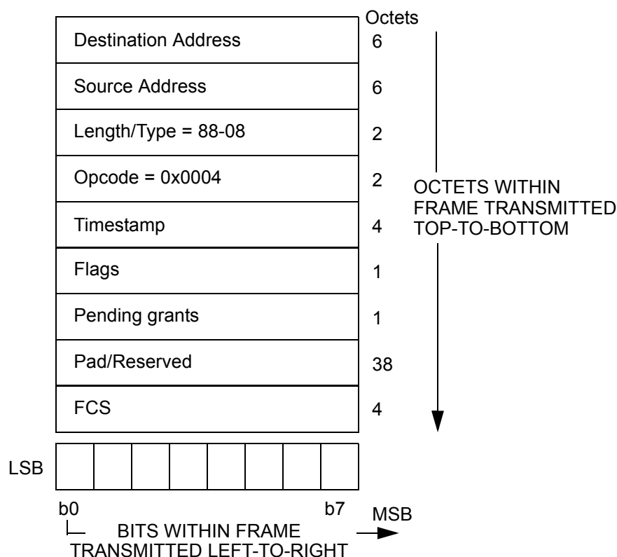
Figure 64–33—REGISTER_REQ MPCPDU
