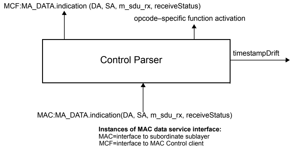
Figure 77–7—Control Parser service interfaces
