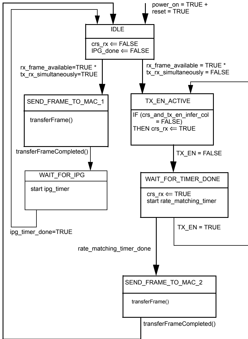
Figure 61-8—MAC-PHY rate matching receive state diagram
