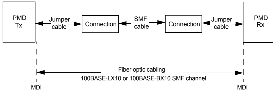
Figure 58–12—Fiber optic cabling model
