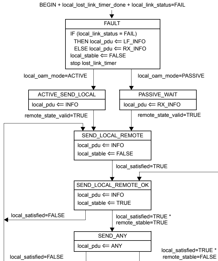
Figure 57–5—OAM Discovery state diagram
