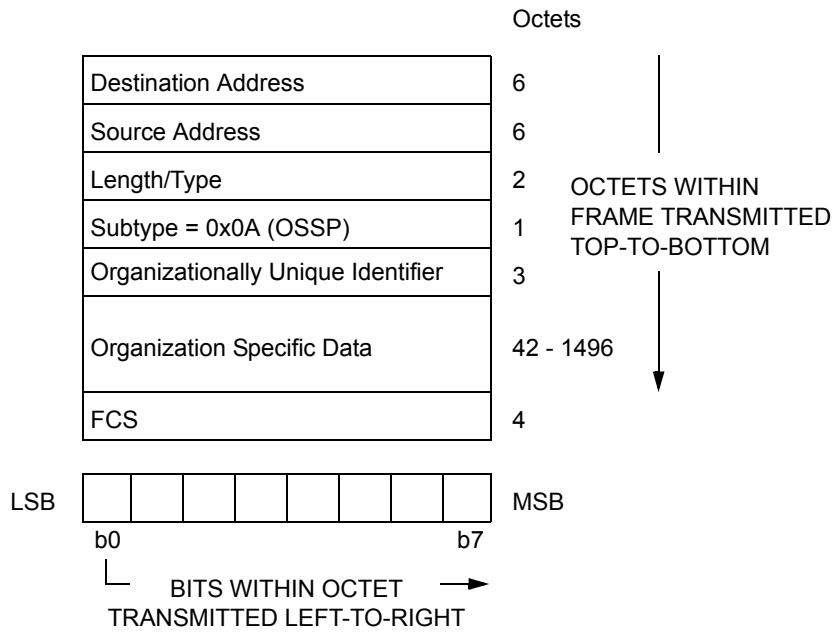
Figure 57B-1—OSSPDU structure
