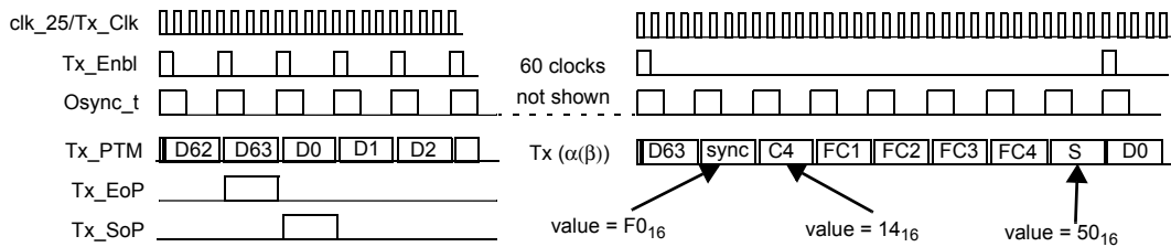
Figure 61–14—Example transmit timing
