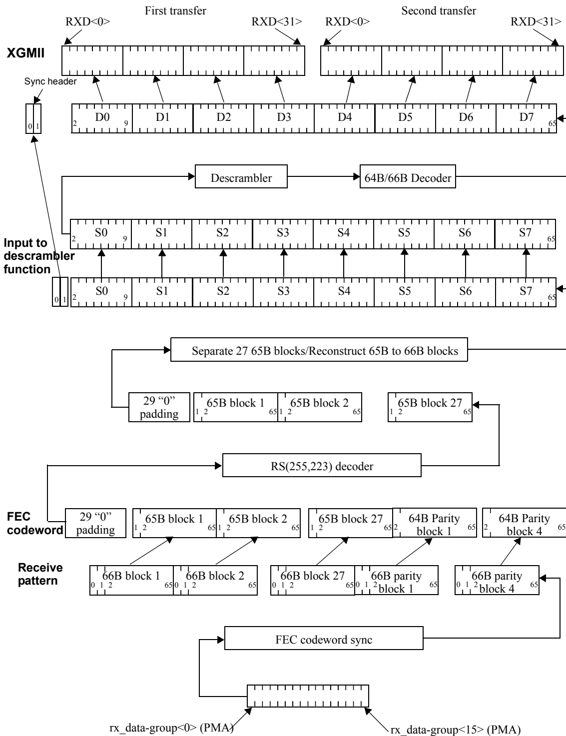
Figure 76–19—PCS Receive bit ordering
