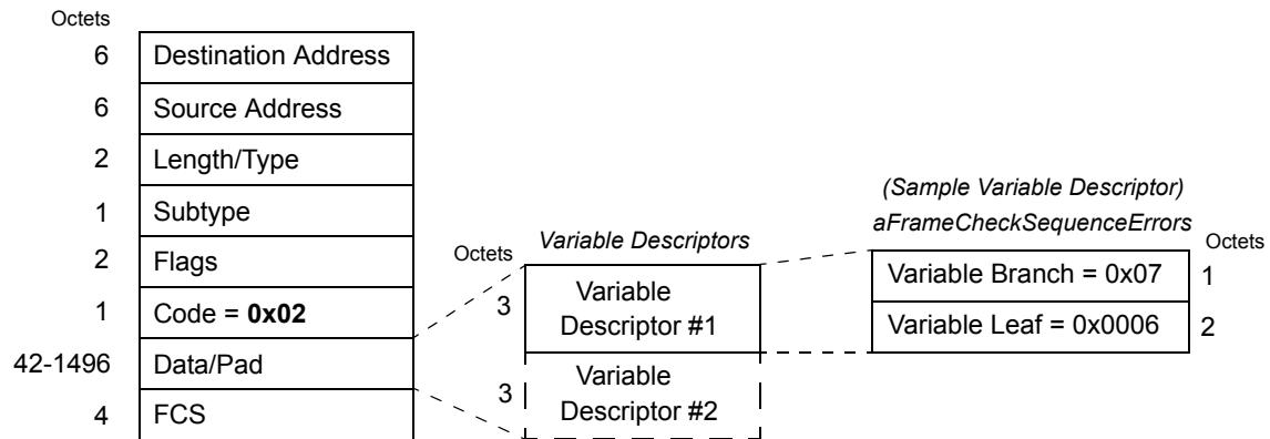
Figure 57–12—Variable Request OAMPDU frame structure
