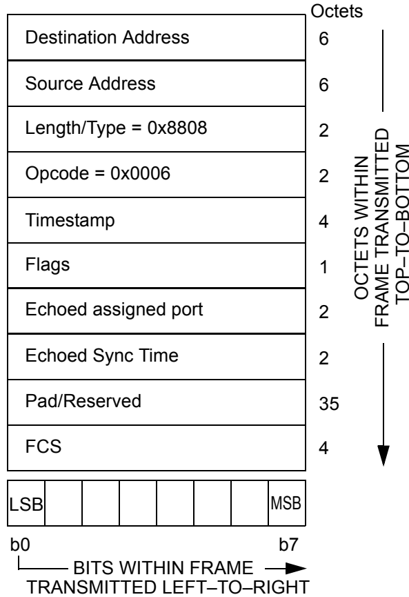
Figure 77–36—REGISTER_ACK MPCPDU
