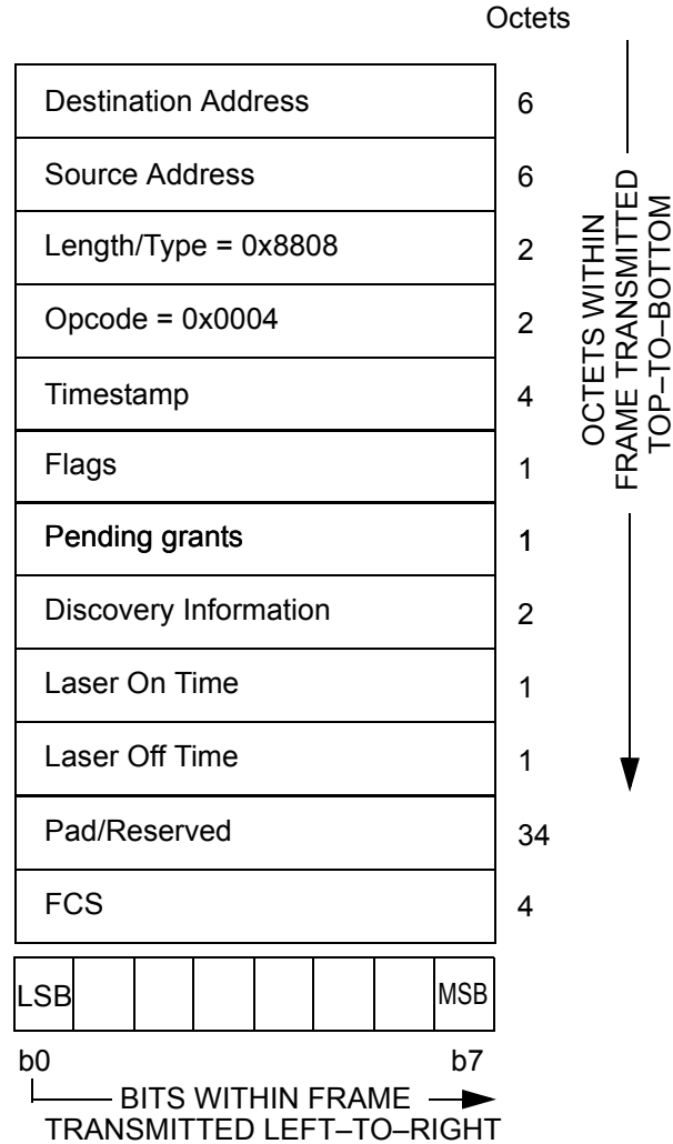
Figure 77–34—REGISTER_REQ MPCPDU
