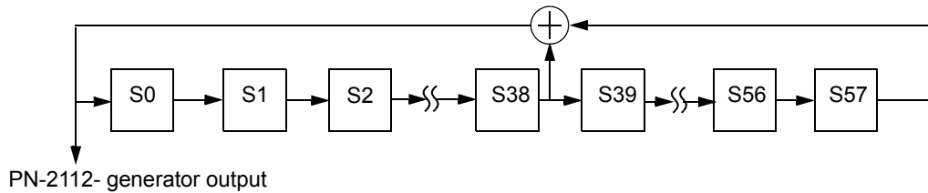
Figure 74–7—PN-2112 generator
