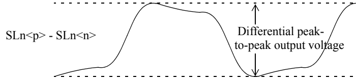
Figure 71-3—Transmitter differential peak-to-peak output voltage definition
