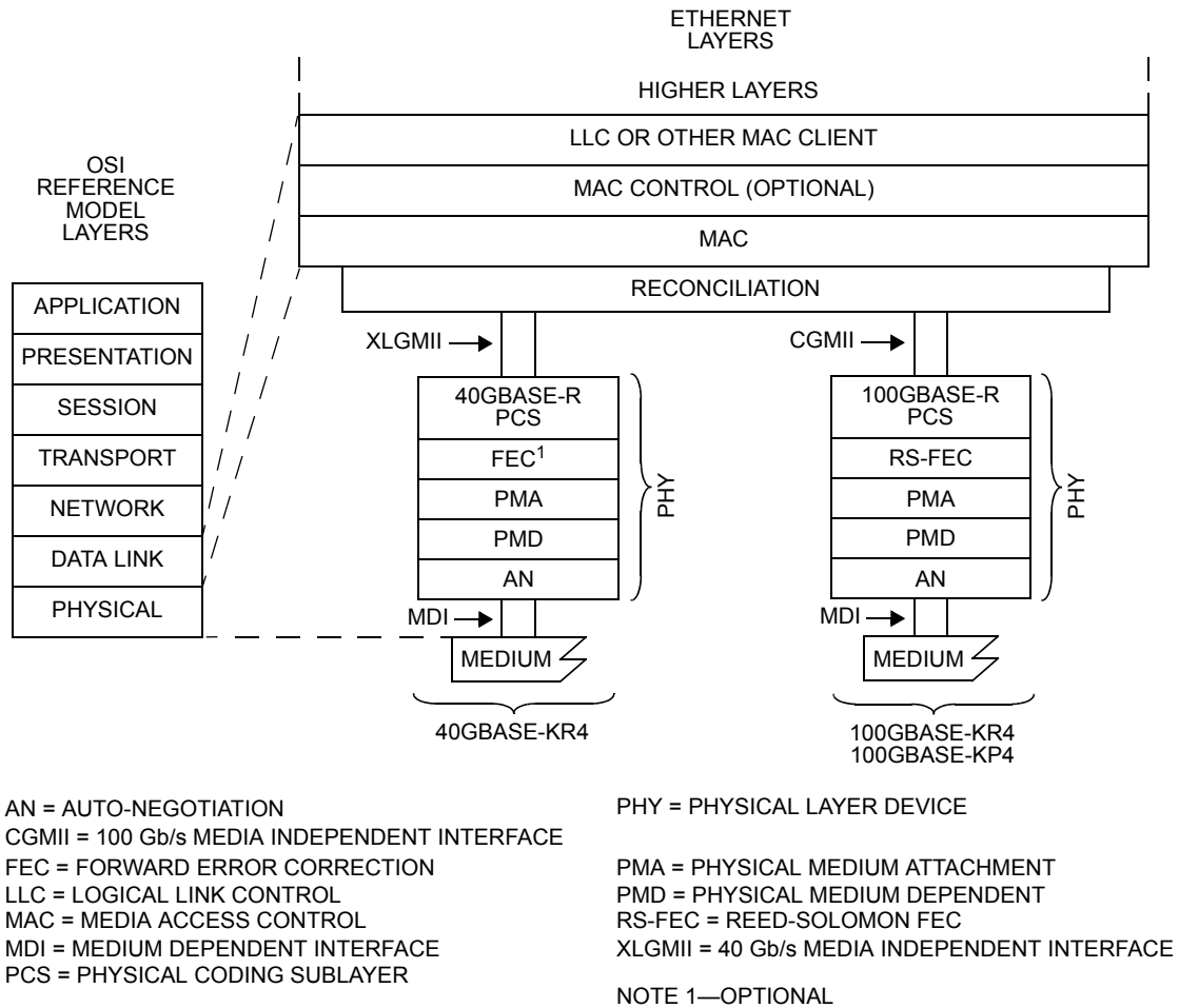
Figure 69-2—Architectural positioning of 40 Gb/s and 100 Gb/s Backplane Ethernet
