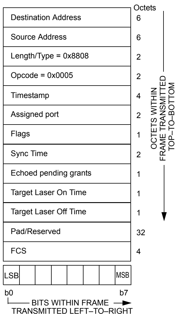
Figure 77–35—REGISTER MPCPDU
