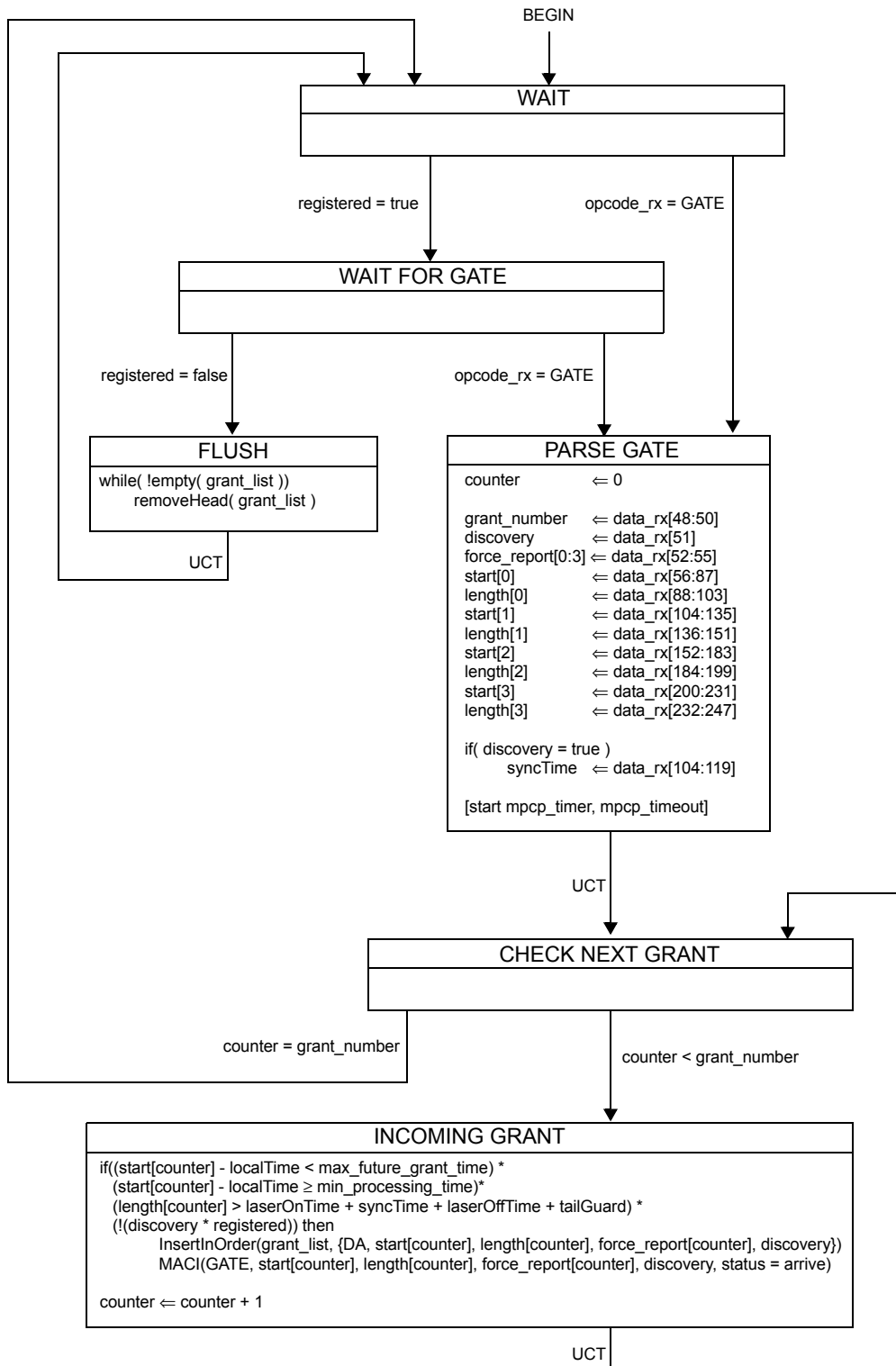
Figure 64-28—Gate Processing ONU Programming State Diagram
