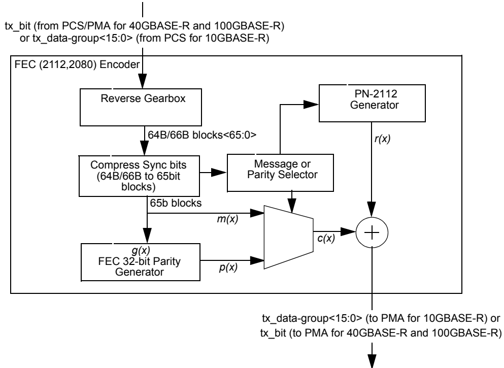
Figure 74-6—FEC (2112,2080) encoding
