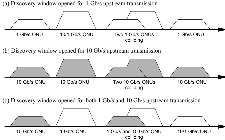
Figure 77-37—Combinations of REGISTER_REQ MPCPDUs during discovery window for 10G-EPON and 1G-EPON coexisting in the same PON
