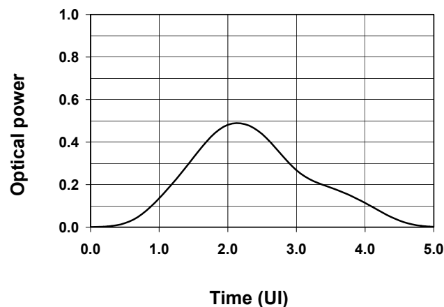
Figure 68–12—Comprehensive stressed receiver test pulse signals (i.e., signals corresponding to an isolated ONE bit)
