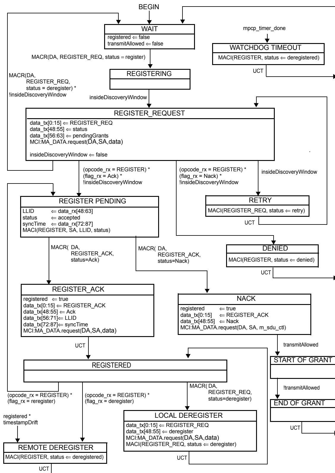
Figure 64-22—Discovery Processing ONU Registration State Diagram
