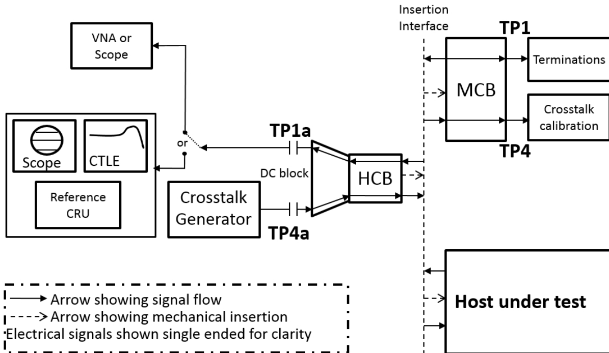
Figure 13-7. Host output test setup
