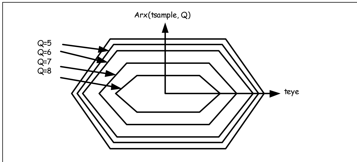
Figure 2-23. Statistical Eye
