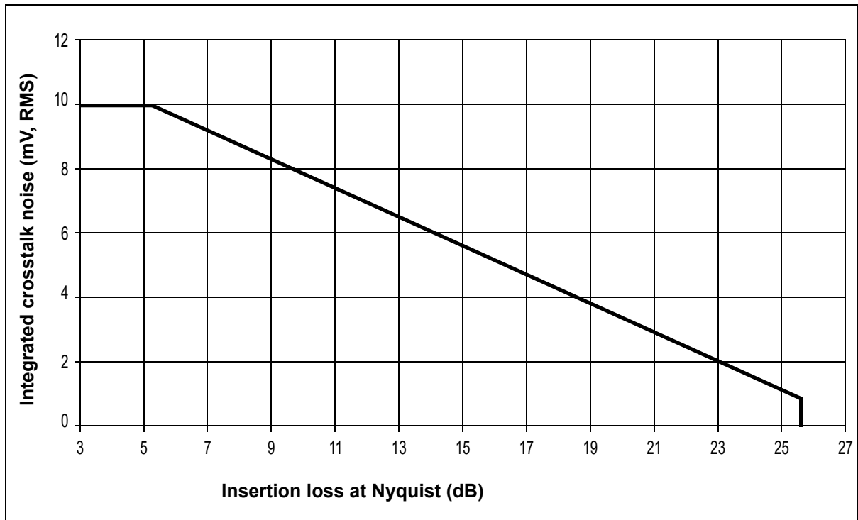
Figure 11-3. Illustration integrated crosstalk noise limits
