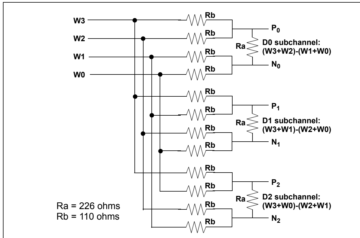
Figure 22-15. ENRZ to Differential Test Conversion Network
