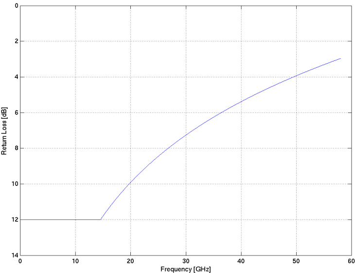
Figure 18-3. CEI-56G-USR-NRZ normative channel return loss at 58.0 Gsym/s
