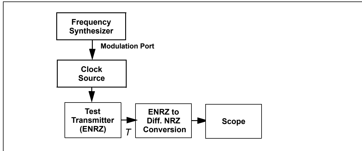
Figure 22-15. ENRZ to Differential Test Conversion Network
