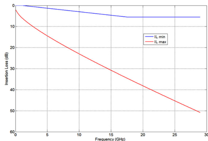
Figure 21-2. Channel Insertion Loss Limit for 29.0 Gsym/s
