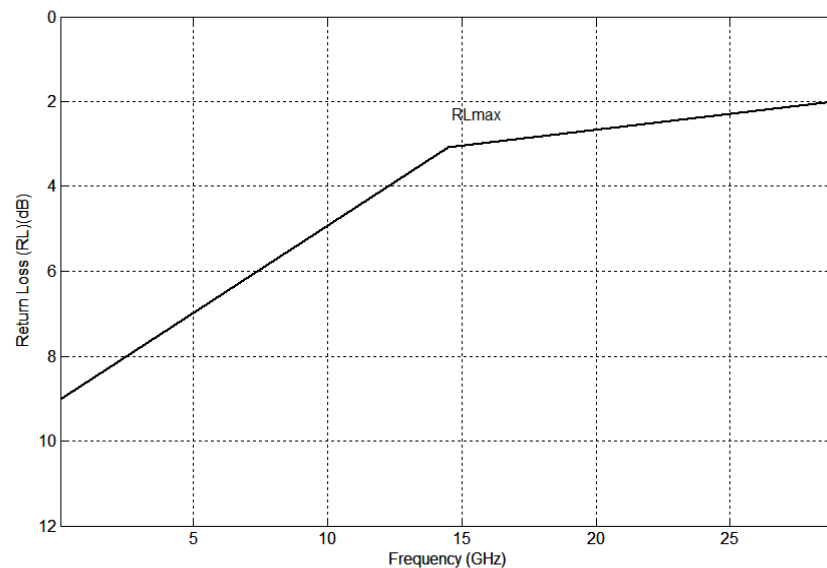
Figure 21-5. Transmitter common mode return loss limit for 29.0 Gsym/s.
