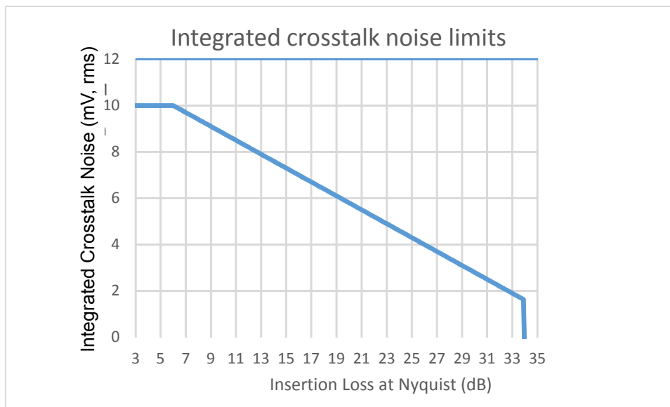
Figure 22-7. Illustration of integrated crosstalk noise limits
