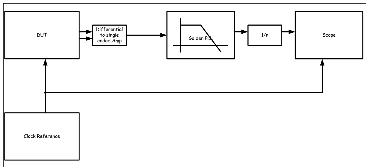
17 Figure 2-30. Transmit Wander Lab Setup
