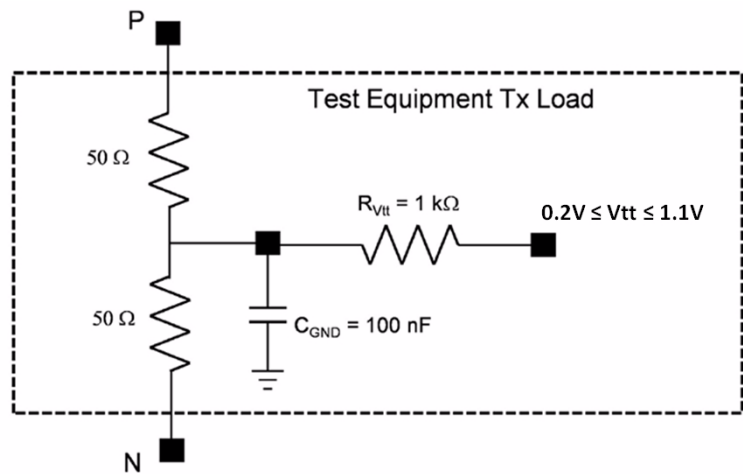
Figure 18-4. Transmitter Amplitude Test Load
