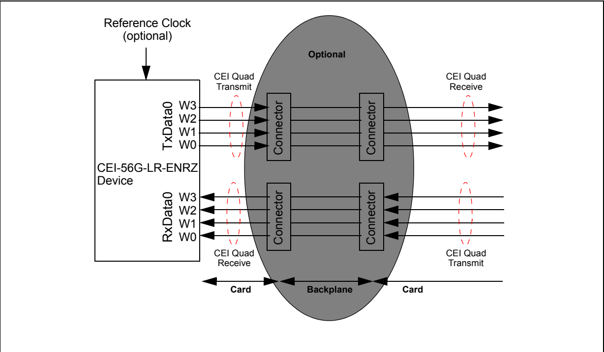
Figure 22-3. Signal Diagram
