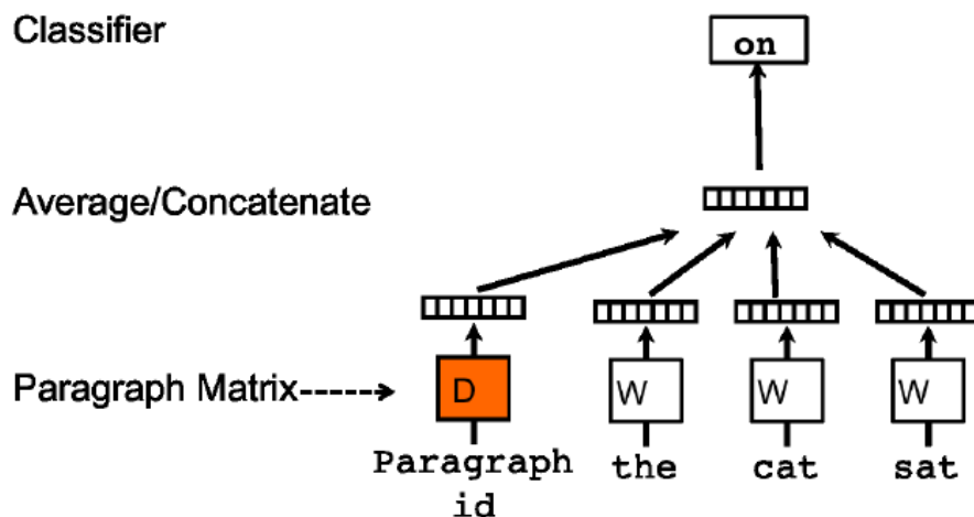
Figure 3.4: Doc2vec Pv-dm Framework for Learning Vectors. Context of Three Words, and Paragraph Vectors Is Used to Predict the next Word.[Le and Mikolov (2014)]
