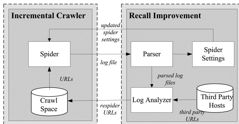
FIG. 4. Spidering process.
