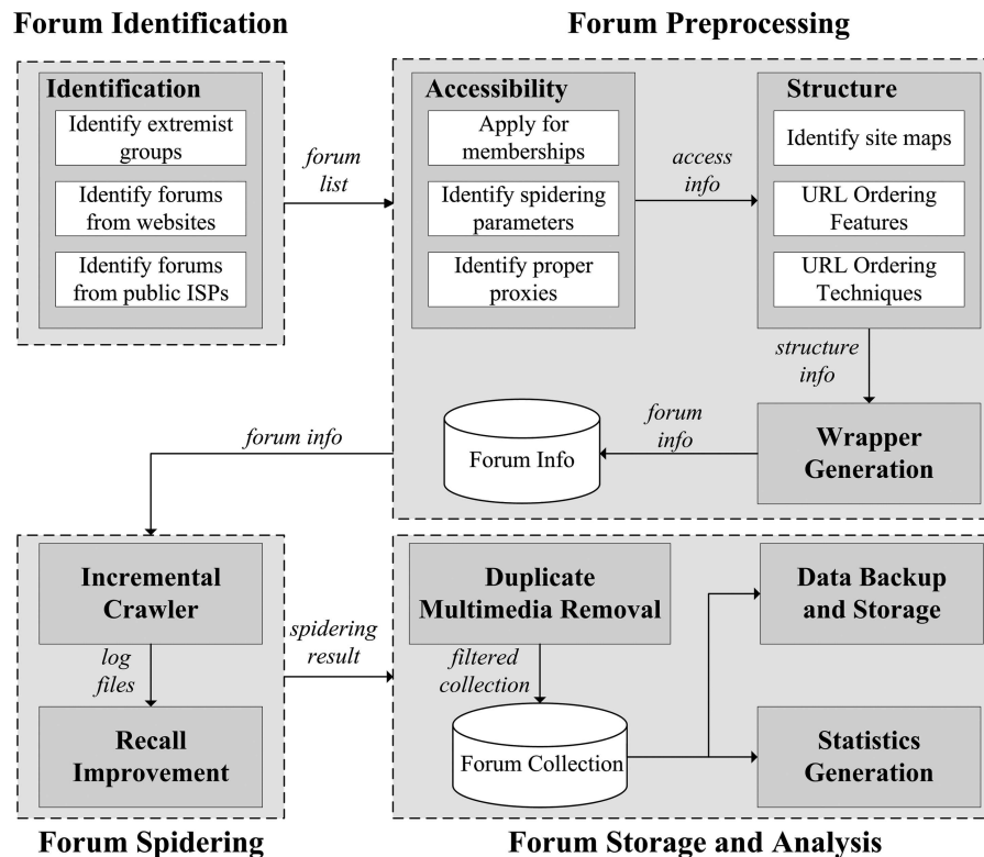
FIG. 1. Dark Web forum crawling system design.
