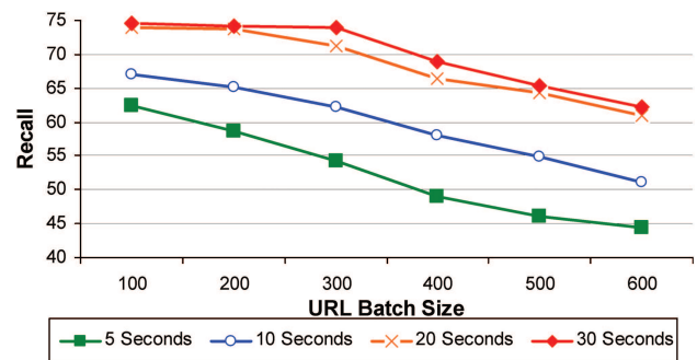
FIG. 9. Recall results for different settings of batch size and timeout interval.
