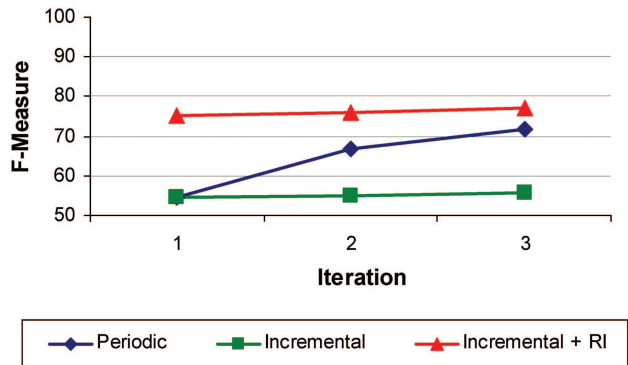
FIG. 11. Results by iteration for various collection-update procedures.
