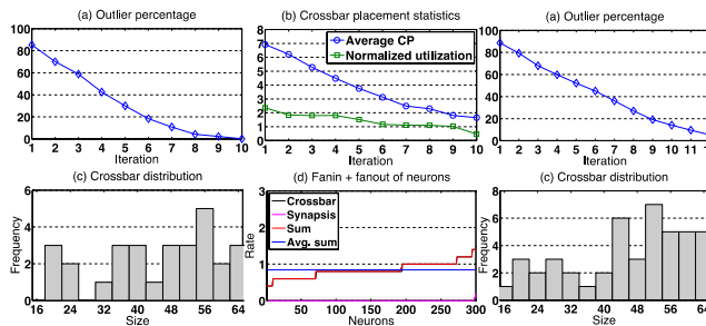
Figure 7. ISC Exp. Result of Testbench 1.
