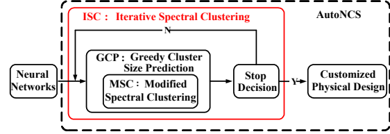
Figure 2. Overview of AutoNCS.
