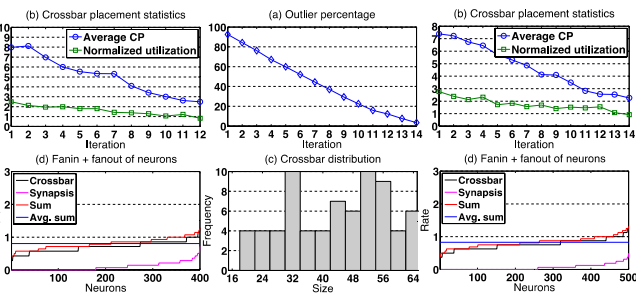
Figure 8. ISC Exp. Result of Testbench 2.
