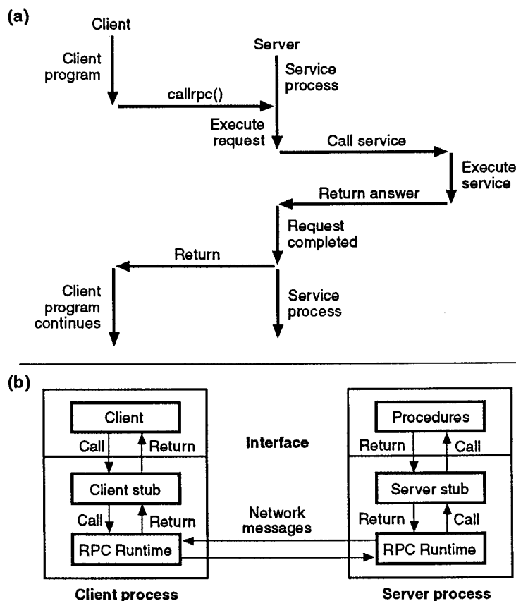
Figure 6. Apollo vs Sun RPC Source: Byte, 1989 [12]
