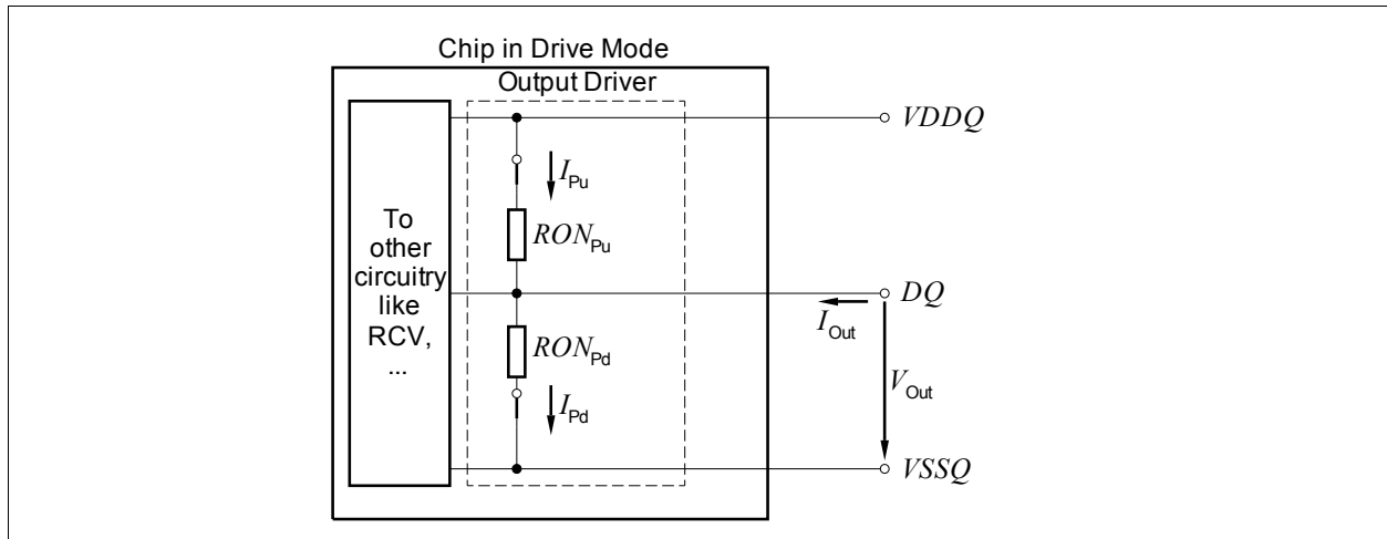
Figure 100 — Output Driver: Definition of Voltages and Currents
