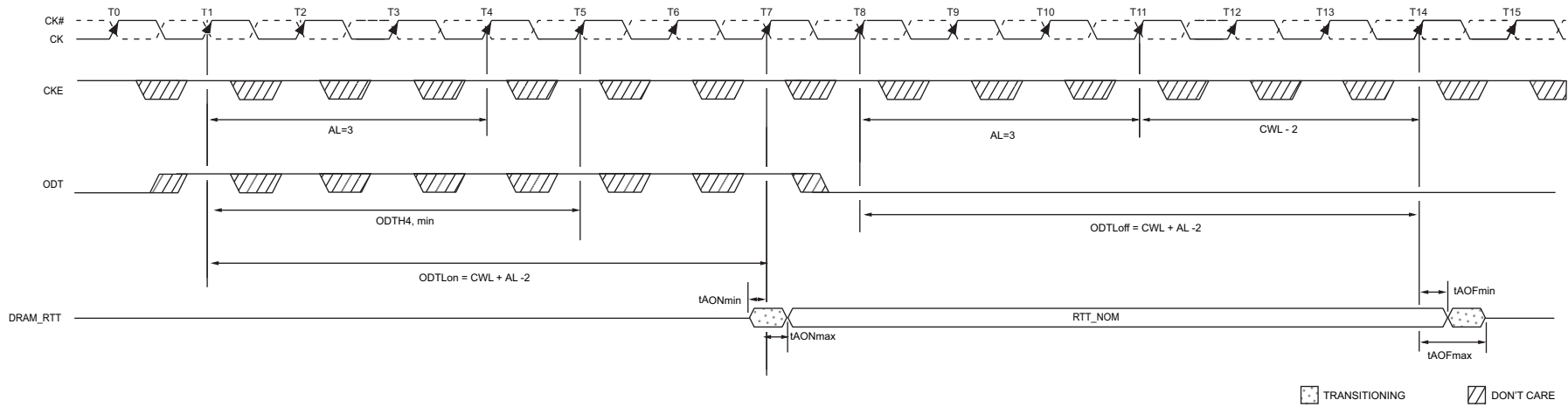
Figure 77 — Synchronous ODT Timing Example for AL = 3 ; CWL = 5 ; ODTLon = AL + CWL - 2 = 6.0 ; ODTLoft = AL + CWL - 2 = 6
