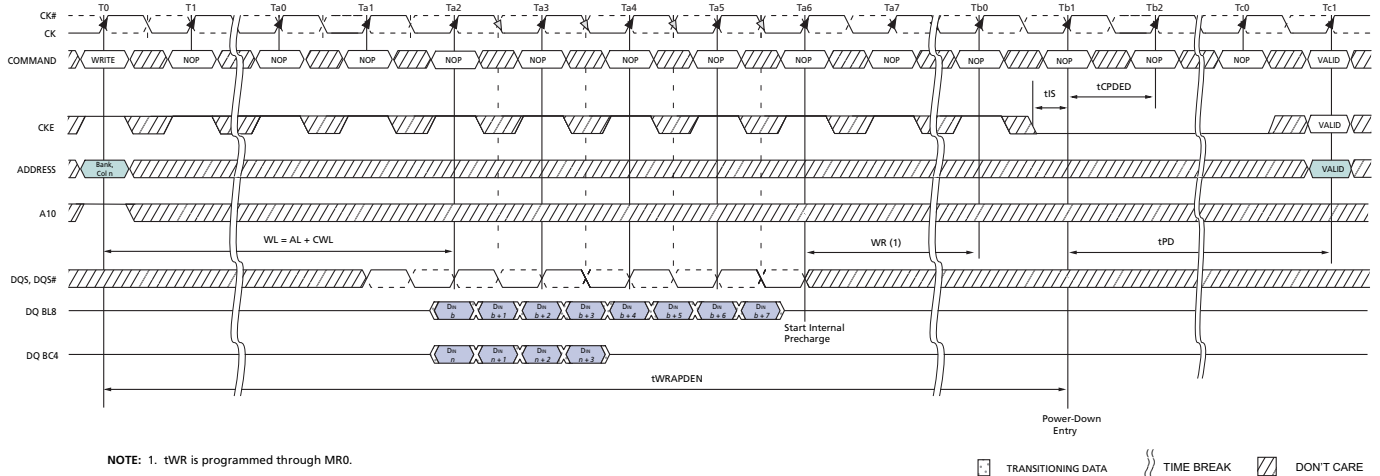
Figure 64 — Power-Down Entry after Write with Auto Precharge
