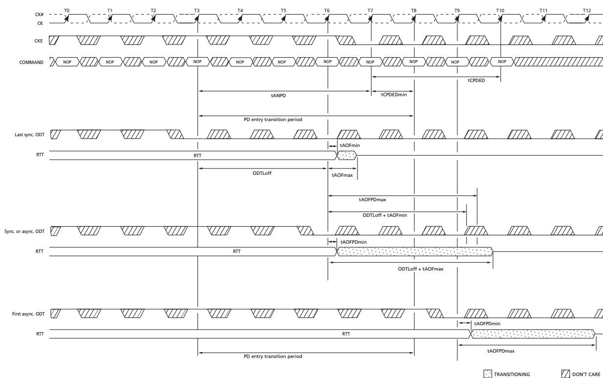
Figure 86 — Synchronous to asynchronous transition during Precharge Power Down (with DLL frozen) entry (AL = 0; CWL = 5; t_{ANPD} = WL - 1 = 4 )
