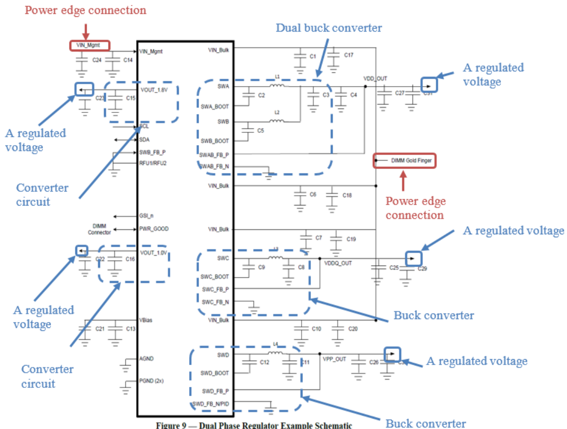
Figure 9 — Dual Phase Regulator Example Schematic
