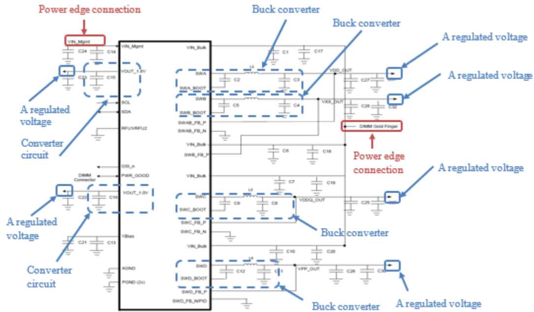
Figure 10 — Single Phase Regulator Example Schematic
