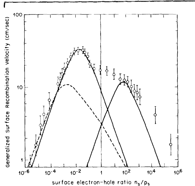
FIG. 2. Generalized surface recombination velocity S_{\text{gen}} as a function of n_s/p_s at a thermally grown Si-SiO 2 interface. The injection level was such that n_b = 3 \times 10^{16}/\text{cm}^3 and p_b = 5.5 \times 10^{16}/\text{cm}^3 . The two solid curves are Lorentzian functions from Eq. (4) representing interface states of two different cross-section ratios \sigma_n/\sigma_p . The dashed line is a model based on DLTS measurements (Ref. 13).
