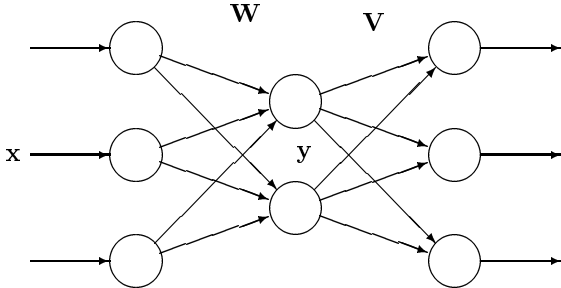
Fig. 5. Auto-encoder network with N = 3 and M = 2 .
