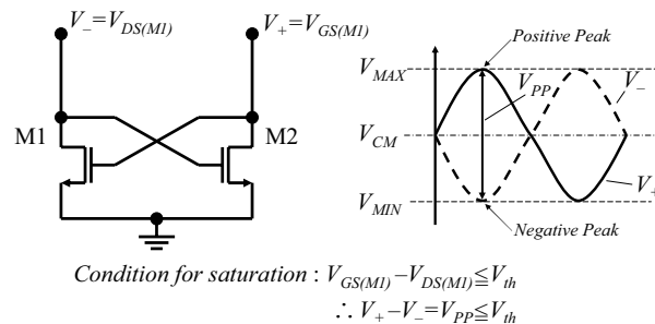
Fig. 2. VCO swing of cross-coupled NMOS
