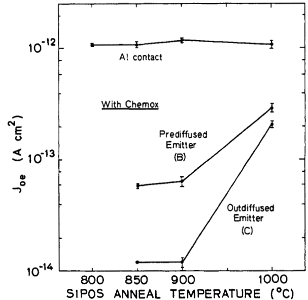
Fig. 6: emitter saturation current vs. anneal temperature for SIPOS contacts with a chemically grown interfacial oxide. The \gamma = 0 SIPOS layer is 3300 angstroms thick.
