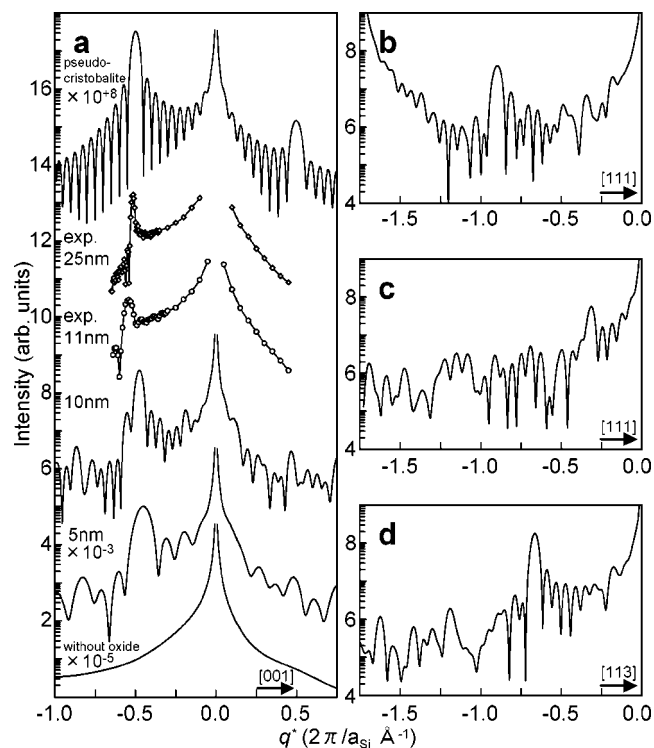
FIG. 2. X-ray diffraction intensities calculated for the SiO 2 /Si models (Fig. 1). Data are plotted on a log scale as a function of q^* , where q^* is the distance along the CTR from the 111 Bragg point in silicon reciprocal lattice unit. (a) Scans of the 10-nm and 5-nm SiO 2 models on Si(001) along [001] where q^*=0 corresponds to 1,1,1, coupled with the data for the bare silicon substrate and the 10 nm pseudocrystal/Si(001) model. Experimental spectra for 11-nm, 25-nm thick oxides (from Ref. 8) are also shown. (b) and (c) Scans of the 10-nm SiO 2 model on Si(111) along [111] ( q^*=0 to 1,1,1 for b and to 1,1,−1 for c) (d) Scan of the 10-nm SiO 2 model on Si(113) along [113] ( q^*=0 to 1,1,1).
