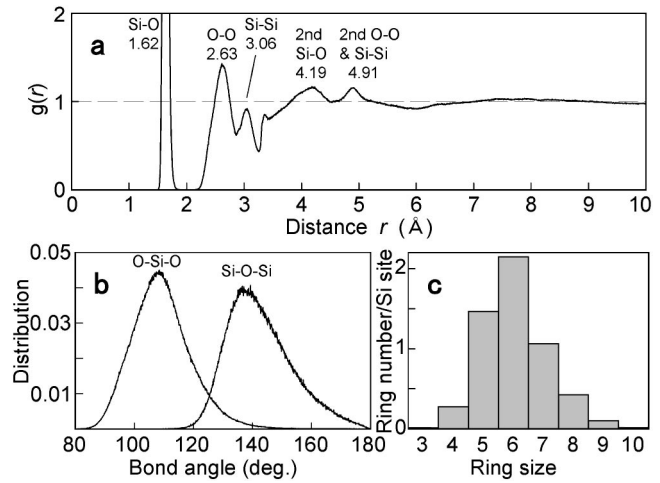
FIG. 5. Analyses of the SiO 2 /Si(001) model at 300 K. (a) Pair-correlation function. (b) Bond angle distributions. (c) Ring statistics according to the shortest path analysis. 26
