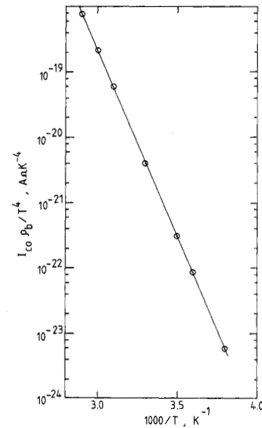
Fig. 6. Graph of \ln I_{C0}/T^4 versus inverse temperature for the RCA and HF devices.
