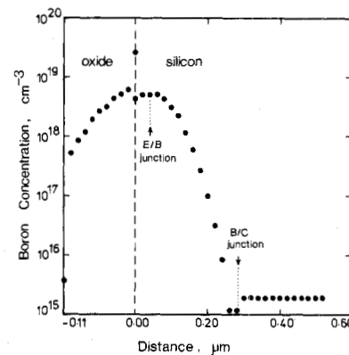
Fig. 7. Theoretical boron profile obtained from the SUPREM process simulation program.
