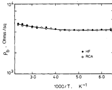
Fig. 5. Temperature dependence of the resistance under the emitter for the RCA and HF devices.
