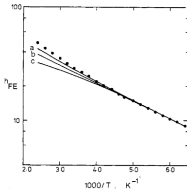
Fig. 8. Fit obtained between the transport theory (15) and the experimental results (HF device 1) for AT^{0.75} \gg 1 (curve a), AT^{0.75} \ll 1 (curve c), and for an intermediate case, (curve b).
