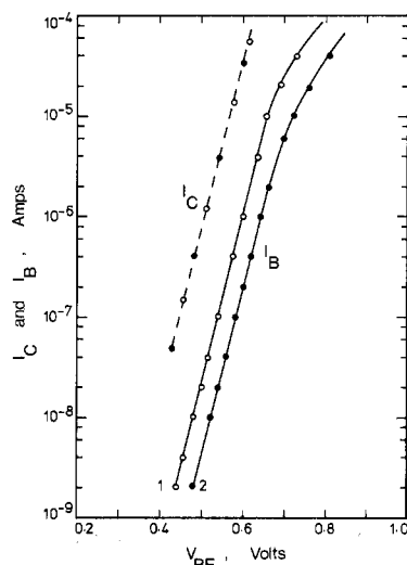
Fig. 3. Collector and base current as a function of base/emitter voltage for a device given an HF etch (device 1), and a comparable device given an RCA clean (device 2).
