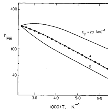
Fig. 9. Fit obtained between the modified tunneling theory (8) and the experimental results (RCA device 2) for three values of the parameter C_h .
