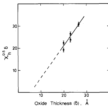
Fig. 10. Graph, taken from the literature [37], showing the relationship between the effective barrier height for holes and the interfacial oxide thickness.
