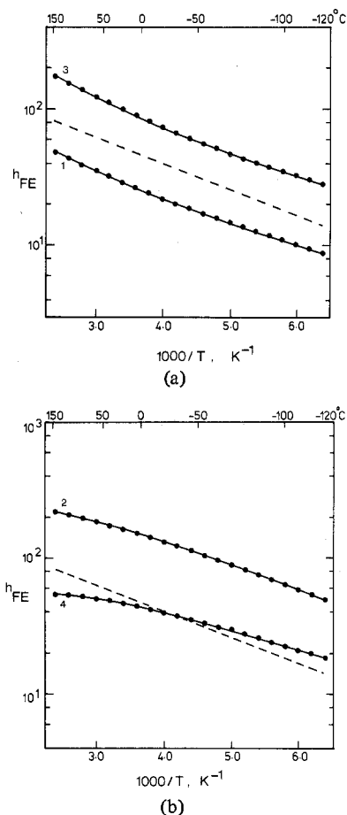
Fig. 4. Temperature dependence of the current gain for (a) two HF devices (transistors 1 and 3) and a conventional transistor (dashed line) and (b) two RCA devices (transistors 2 and 4) and a conventional transistor (dashed line).
