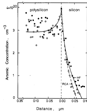
Fig. 2. Arsenic profiles, obtained from Rutherford backscattering experiments, for samples given an HF etch and an RCA clean.
