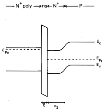
Fig. 1. Band diagram for a polysilicon-emitter bipolar transistor with a thin interfacial oxide layer.
