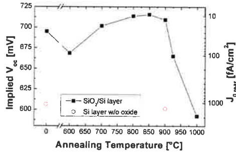
Figure 1: The diagram depicts the implied V_{oc} of TOPCon's interface passivation as a function of the plateau temperature T_{\text{anneal}} of the furnace anneal. The samples without tunnel oxide (red circles) clearly underline the importance of the tunnel oxide layer for surface passivation. Additionally, the right y-axis depicts the corresponding J_{0, \text{rear}} values calculated according to Eq. 3.
