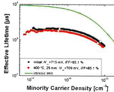
Figure 2: Measured injection dependent effective minority carrier lifetime for a sample symmetrically passivated by the TOPCon structure after thermal treatment at 800 °C and subsequent hotplate annealing at 400 °C for 25 min, respectively. The figure also depicts the open-circuit (1 sun, open diamonds) and MPP conditions (open circles) as well as the intrinsic limit of the absorber calculated according to [19].
