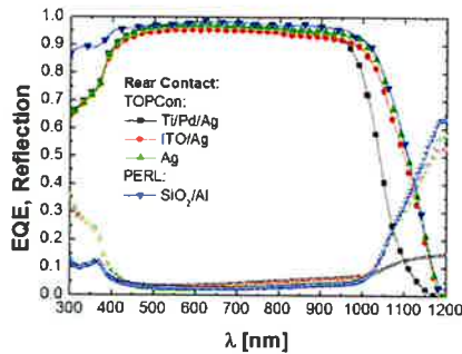
Figure 4: External quantum efficiency (lines and closed symbols) as well as the reflection (open symbols) of solar cells with different rear metallization schemes are plotted over wavelength. Titanium is a very lossy metal and offers very weak reflection above 1000 nm. On the contrary, the stack of ITO/Ag reflects almost as much light as the Ag single layer. The best light management is obtained with our PERL cell (open symbols) [26] featuring a 100 nm \text{SiO}_2/\text{Al} mirror. Note, the cell's reflection in the wavelength range below 400 nm and between 600 and 1000 nm is slightly lower due to the use of inverted pyramids and a double antireflection coating.
