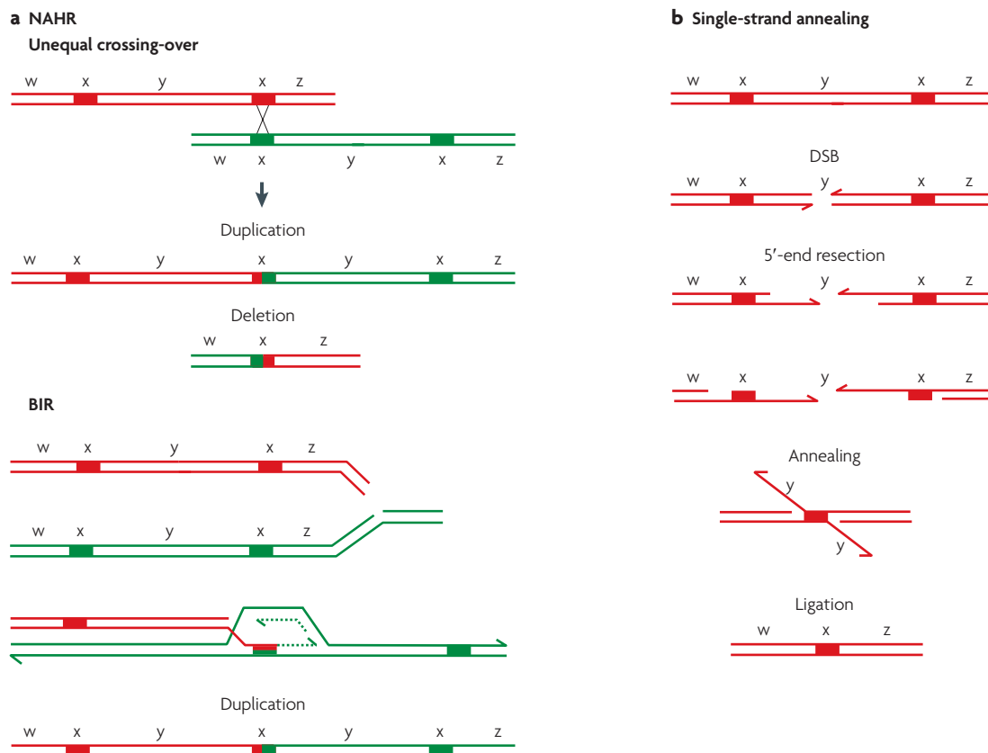
Figure 3 | Change in copy number by homologous recombination. Each line represents a single DNA strand, polarity is indicated by half arrows on 3' ends, and specific sequences are identified by letters w–z. a | Non-allelic homologous recombination (NAHR) will occur by unequal crossing over if a recombination repair event uses a direct repeat (x) as homology (upper panel). In this situation, a crossover outcome leads to products that are reciprocally duplicated and deleted for the sequence between the repeats (y). These might segregate from each other at the next cell division, thus changing the copy number in both daughter cells. NAHR can also occur by BIR when the broken molecule uses ectopic homology to restart the replication fork (lower panel). BIR will form duplications and deletions in separate events. b | Single-strand annealing. When 5'-end resection on either side of a double-stranded break (DSB) does not lead to invasion of homologous sequence, resection continues. If this resection reveals complementary single-stranded sequence (x) shown by the filled regions, these can anneal. Removal of flaps, gap filling and ligation complete repair of the DSB with deletion of the sequence between the repeats (y) and of one of the repeats.
