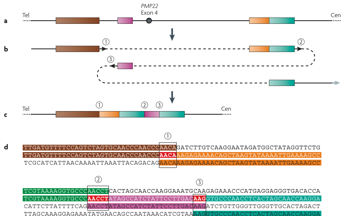
Figure 1 | Complex structural variation. An example of a complex genomic rearrangement in humans, with microhomology junctions that caused the deletion of ~9 kb, including exon 4 of the gene for peripheral myelin protein 22 ( PMP22 ) 18 . a | A map of part of PMP22 , before the microhomology junctions are formed. The coloured boxes represent blocks of sequence. b | A hypothetical series of three template switches that would achieve the rearrangements, indicated by the black arrows and numbers; the grey arrow signifies resumption of replication on the original template. The template switches also could have occurred in the opposite order. Numbers correspond to the junctions detailed in part d . c | The rearranged chromosomal region, in which a deletion of exon 4 has joined the brown sequence to the orange and green sequence, followed by an inversion of part of the deleted segment (pink sequence) and a direct duplication of the green sequence. d | The nucleotide sequences of the coloured segments in the same colours as in part a . The boxes outline interacting microhomology sequences. In the upper panel, the top line is parental sequence, the second line is the sequence of the rearranged chromosome and the bottom line is the parental interacting sequence from the other side of the deletion. The junction between the brown sequence and the orange and green sequence shows a 4-bp microhomology (red). The lower panel shows the sequences that interacted to make junctions 2 and 3. The second line has the new sequence joining green to inverted pink sequence (third line) with a 5-bp microhomology (red), and the fourth line show the sequence that interacted in inverted orientation to make junction 3 (pink sequence to green sequence) with a 3-bp microhomology (red). The orange and green fragment is 98 bp and the pink fragment is 28 bp, including the microhomology sequences at both ends. Cen, centromere; tel, telomere. Figure is reproduced from Nature Genetics REF. 18 © (2009) Macmillan Publishers Ltd. All rights reserved.
