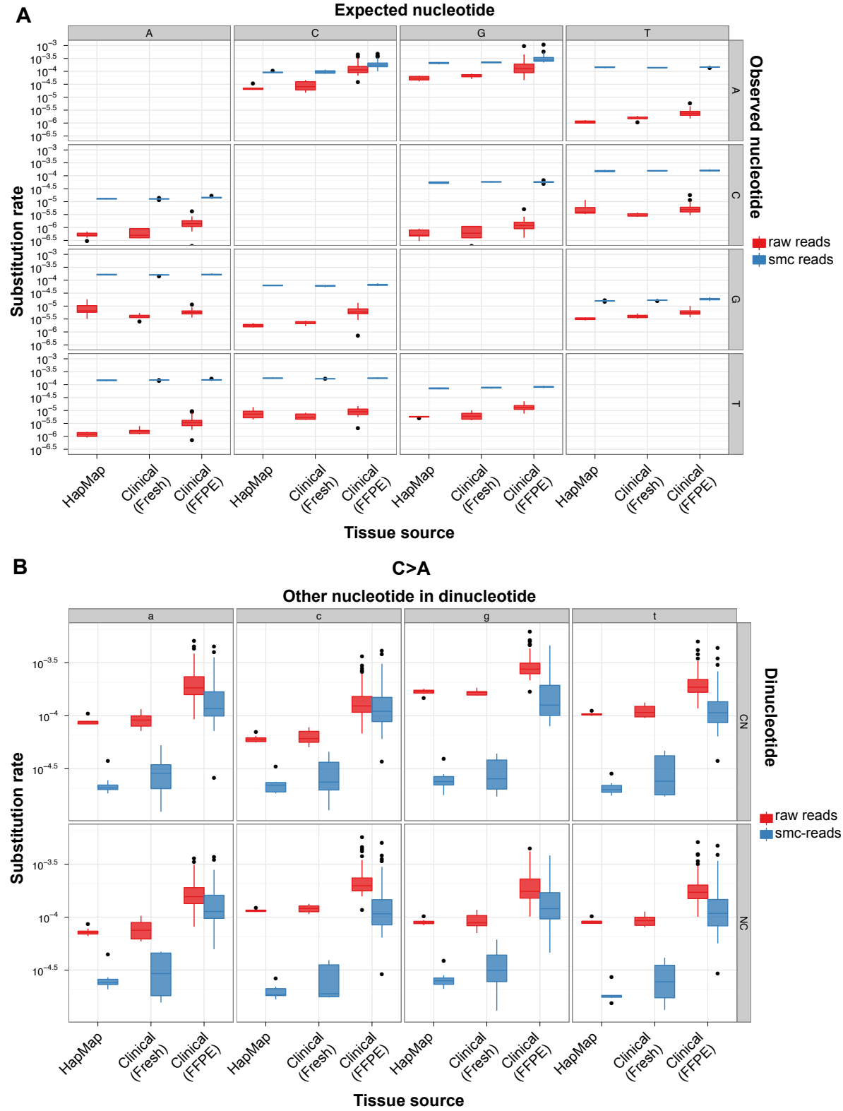
Supplemental Fig. S5. Substitution rate distributions as a function of expected and observed gap-fill nucleotide.
