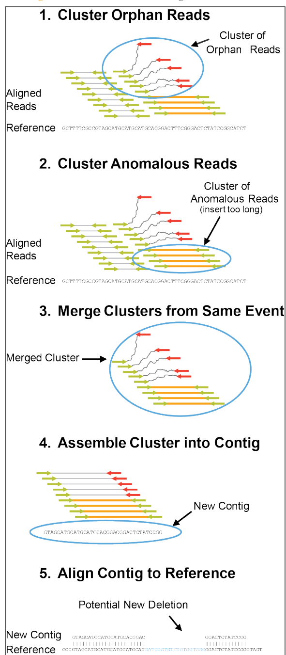
Figure 25 assembleIndels Algorithm
