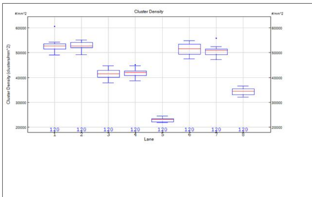
Figure 6 Cluster Density
