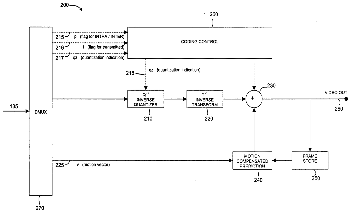
Fig. 2 (PRIOR ART)
