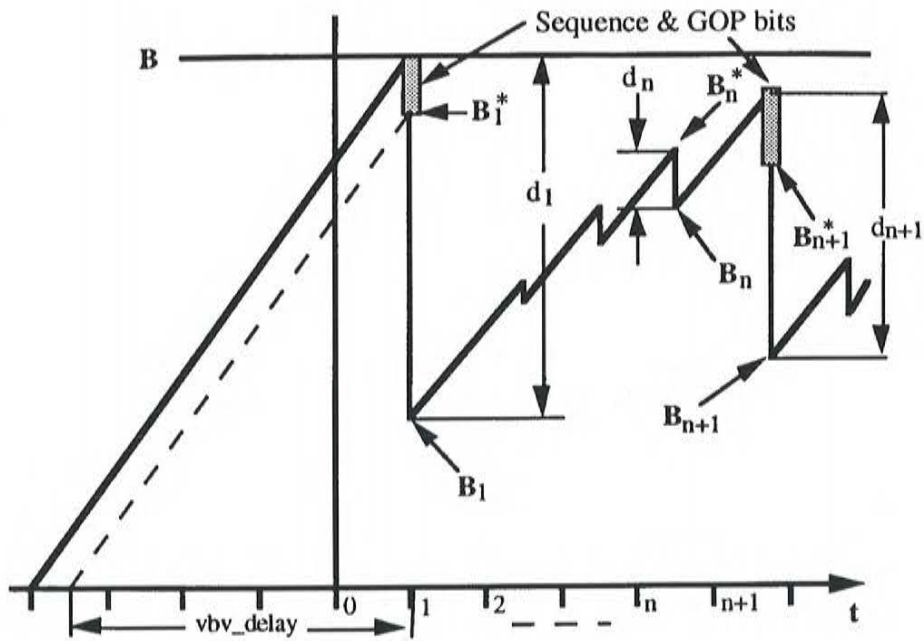
Figure C.1 -- VBV buffer occupancy
