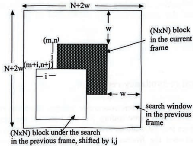
Figure 3.6 The current and previous frames in a search window
