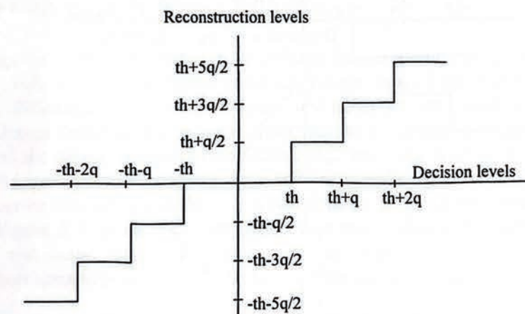
Figure 3.3 Quantisation characteristics
