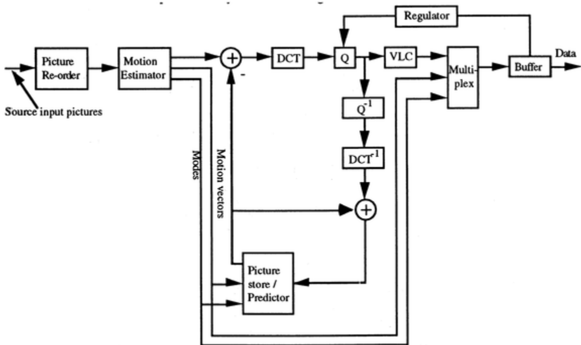
MPEG-1, Fig. 2 (Simplified video encoder block diagram).
