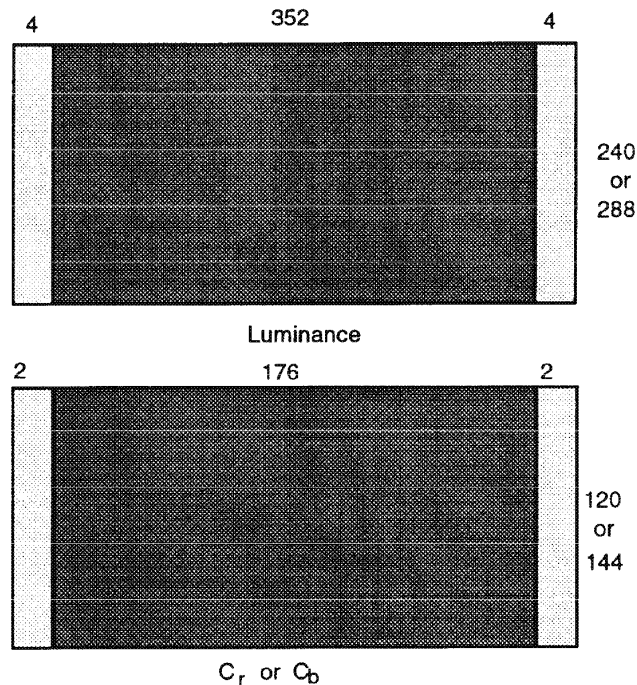
Figure D.13 -- Source input with significant pel area shaded dark
