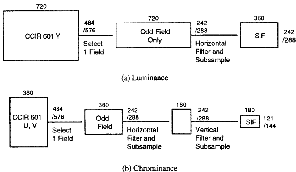
Figure D.12 -- Conversion from CCIR 601 into SIF
