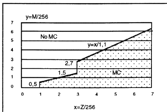
Figure D.33 -- Characteristic MC/No MC
