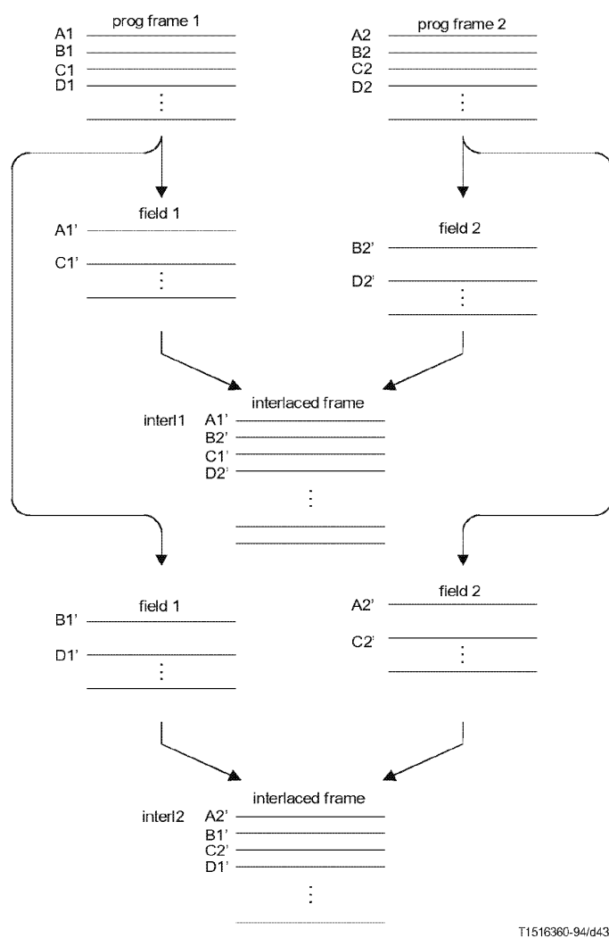
Figure D.3 – Progressive to two interlace conversion
