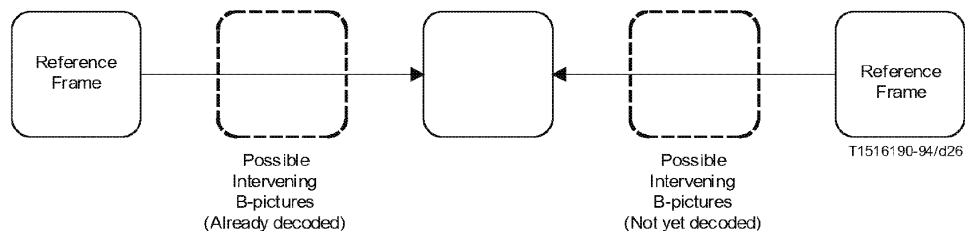
Figure 7-11 – Frame-prediction for B-pictures
