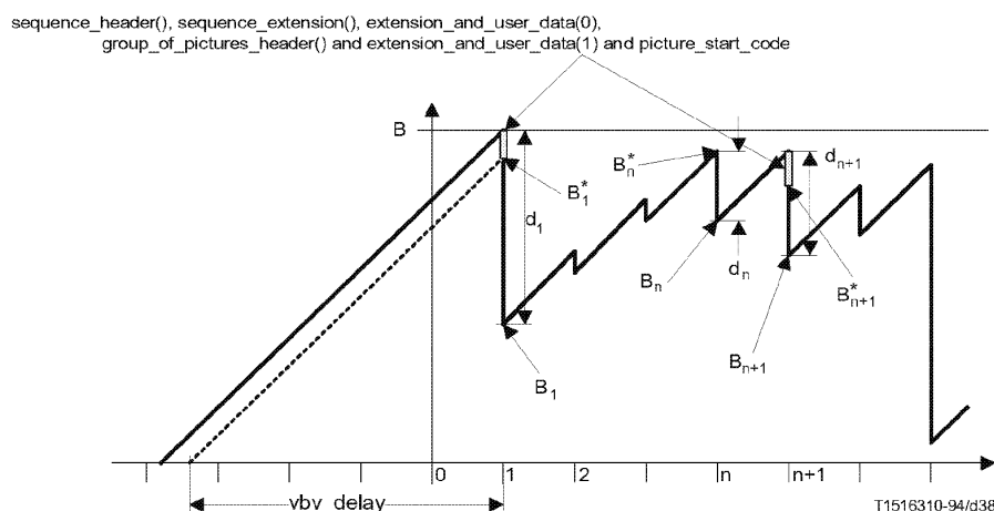
Figure C.1 – VBV Buffer Occupancy – Constant bit-rate operation
