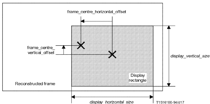
Figure 6-16 – Frame centre offset parameters
