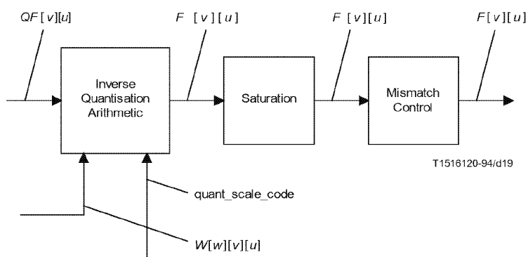
Figure 7-4 – Inverse quantisation process
