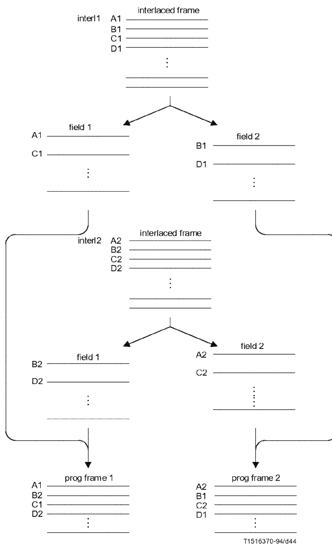
Figure D.4 – Two interlace to progressive conversion
