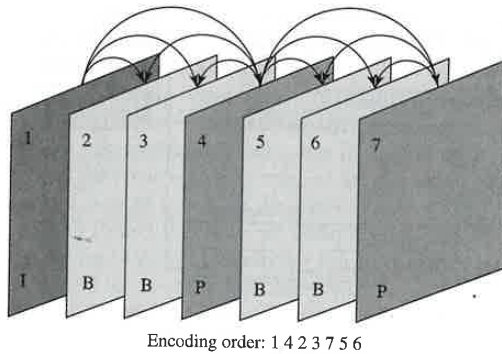
Figure 9.12 Video coding using both uni- and bidirectional temporal prediction. The arrows indicate the reference frames used for predicting a coded frame. Frames labeled I, P, and B are coded without prediction, with unidirectional prediction, and with bidirectional prediction, respectively.
