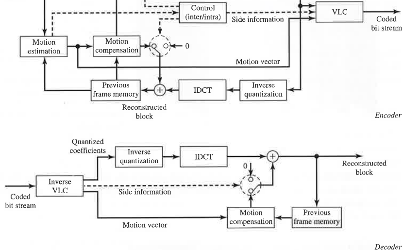
Figure 9.13 Encoding and decoding process for a block in a typical block-based hybrid coding system.
