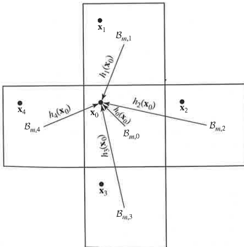
Figure 9.14 An example of overlapped block motion compensation, using four neighboring blocks.
