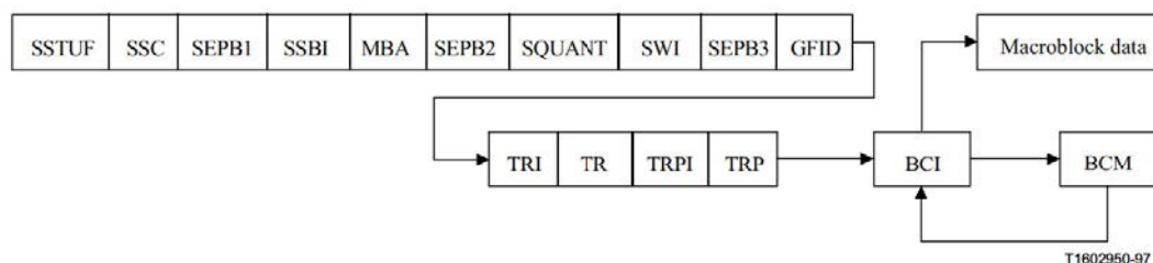
Figure N.3/H.263 – Structure of slice layer for NEWPRED
