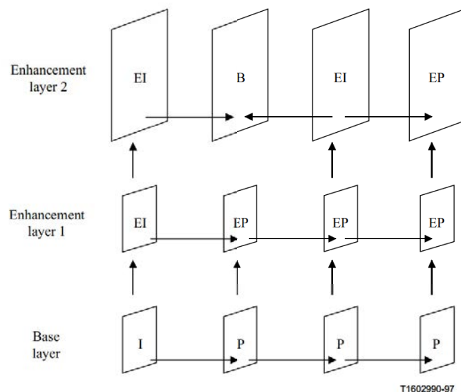
Figure O.4/H.263 – Illustration of multilayer scalability
