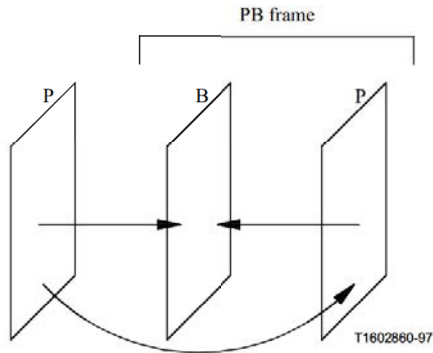
Figure G.1/H.263 – Prediction in PB-frames mode
