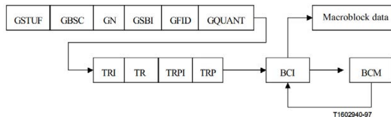
Figure N.2/H.263 – Structure of GOB layer for NEWPRED
