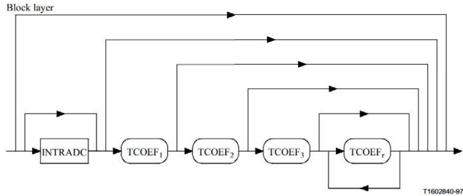
Figure E.1/H.263 – Structure of SAC Block layer
