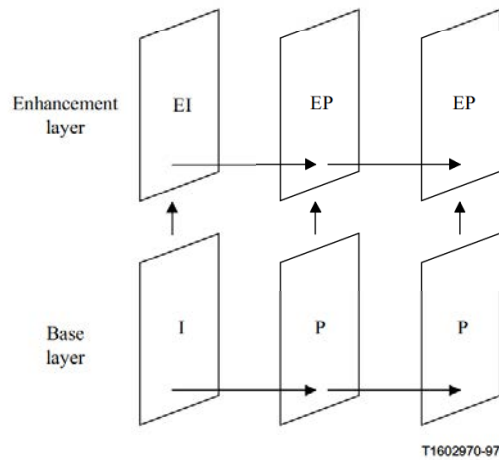
Figure O.2/H.263 – Illustration of SNR scalability
