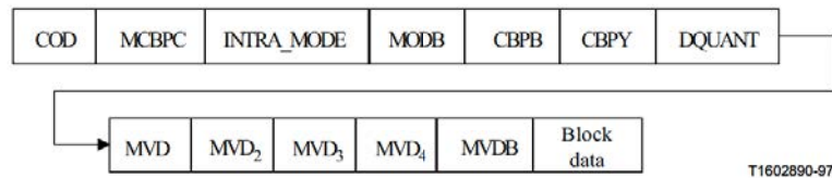
Figure I.1/H.263 – Structure of macroblock layer
