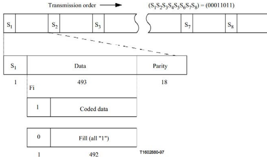
Figure H.1/H.263 – Error correcting frame
