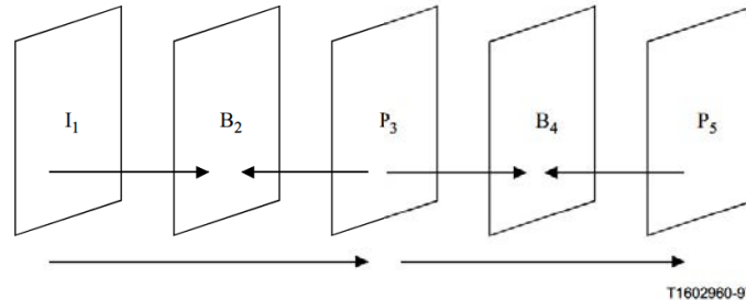
Figure O.1/H.263 – Illustration of B-picture prediction dependencies
