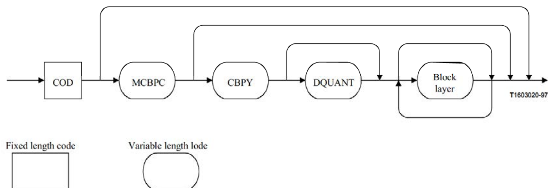
Figure O.7/H.263 – Macroblock syntax for EI-pictures
