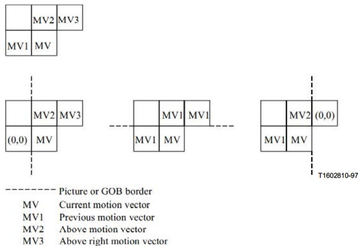
Figure 12/H.263 – Motion vector prediction
