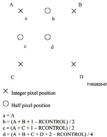
Figure 13/H.263 – Half-pixel prediction by bilinear interpolation
