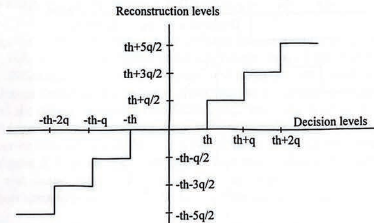
Figure 3.3 Quantisation characteristics
