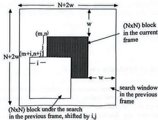
Figure 3.6 The current and previous frames in a search window
