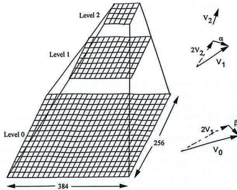
Figure 3.8 A three-level image pyramid
