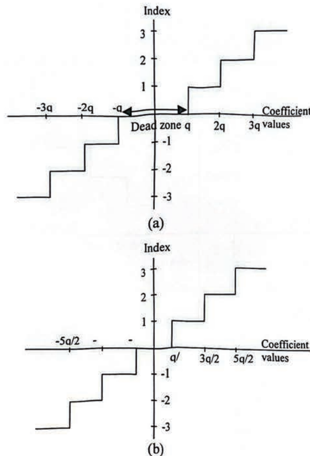
Figure 3.4 Uniform quantisers (a) with and (b) without dead zone
