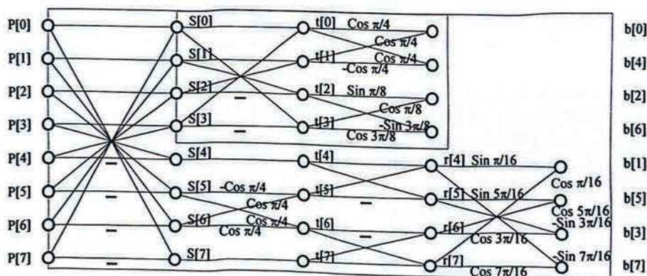
Figure 3.2 A fast DCT flow chart
