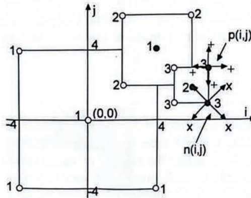
Figure 3.7. An example of the CSA search for w=8 pixels/frame
