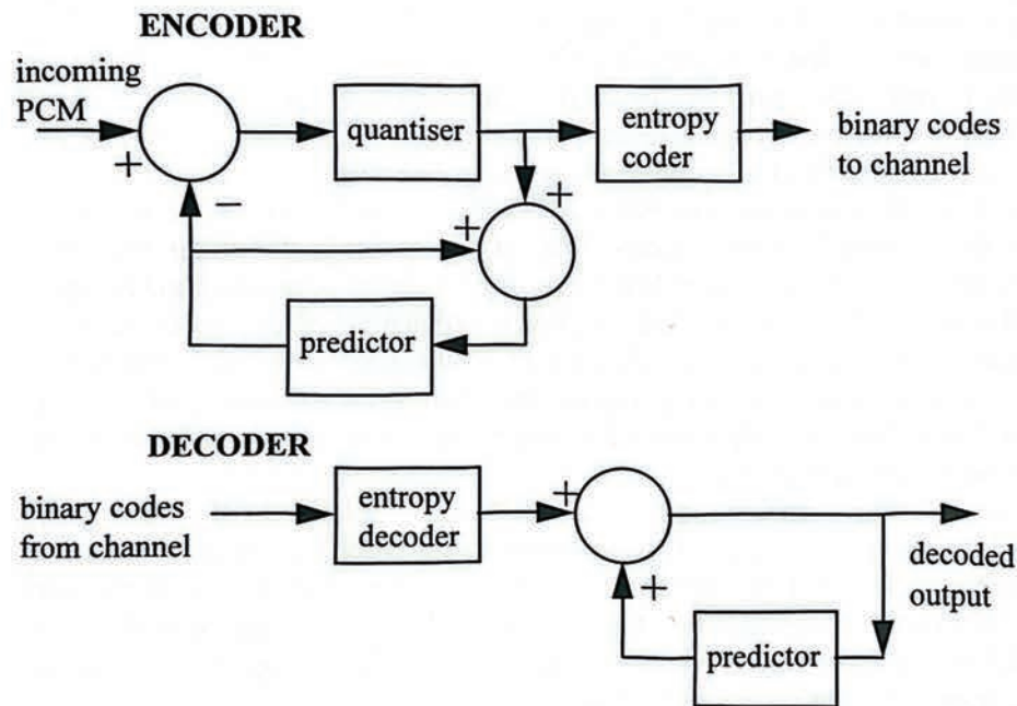
Figure 3.1 Block diagram of a DPCM codec
