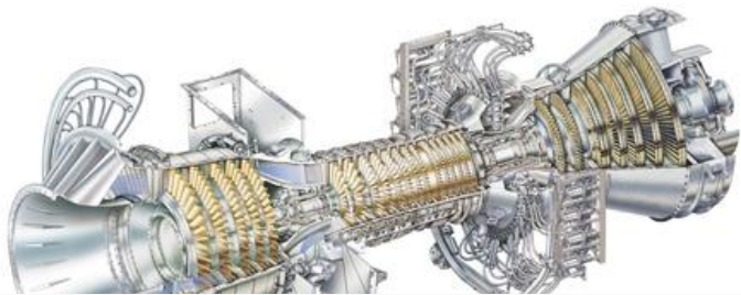
LMS100-PA Aero derivative Gas Turbine Package (106 MW)
