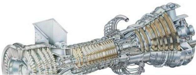
LM6000-PH DLE Aero-derivative Gas Turbine Package (48-53 MW)
