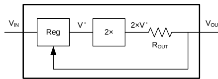
Figure 11. LM2750 Output Resistance Model
