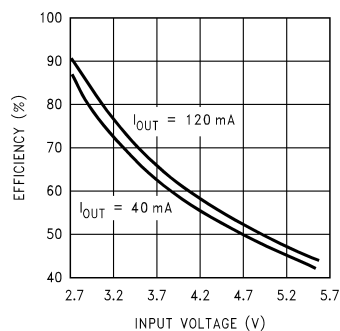
Figure 14. Power Efficiency
