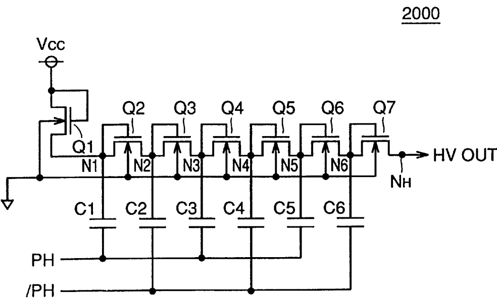
FIG.19 PRIOR ART
