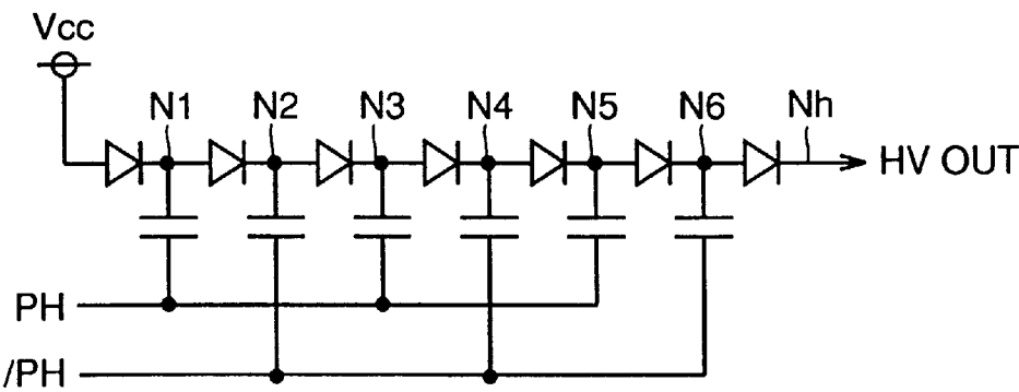
FIG.21 PRIOR ART
