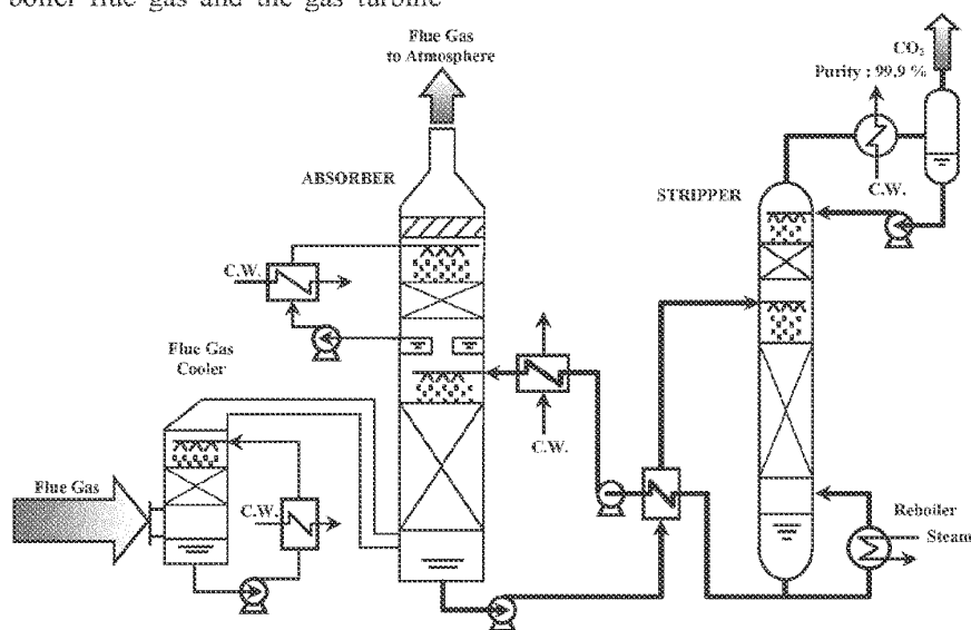
Figure 3. Flue Gas CO 2 Recovery System
