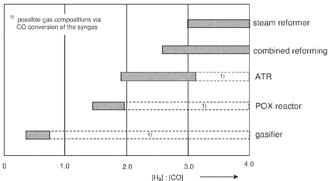
Fig. 1: Composition ranges provided by syngas generators
