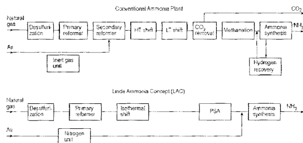
Figure 114. Comparison of Linde LAC process with a conventional process
