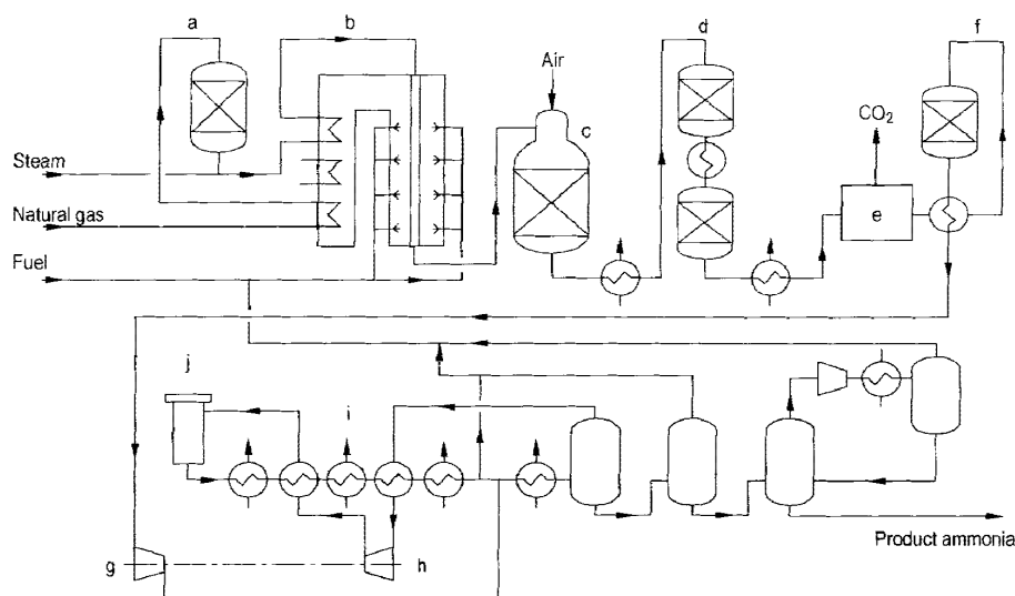
Figure 108. Haldor Topsøe's low energy process
