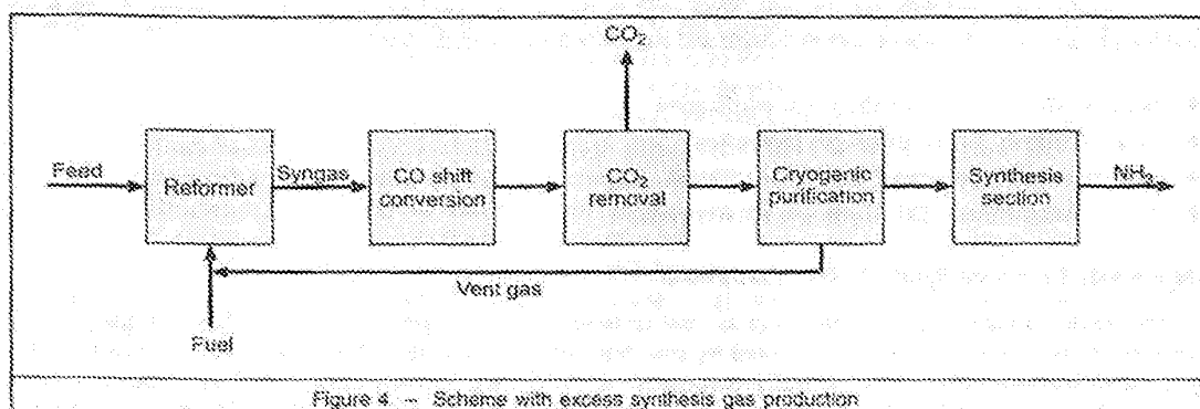
Figure 4 -- Scheme with excess synthesis gas production
