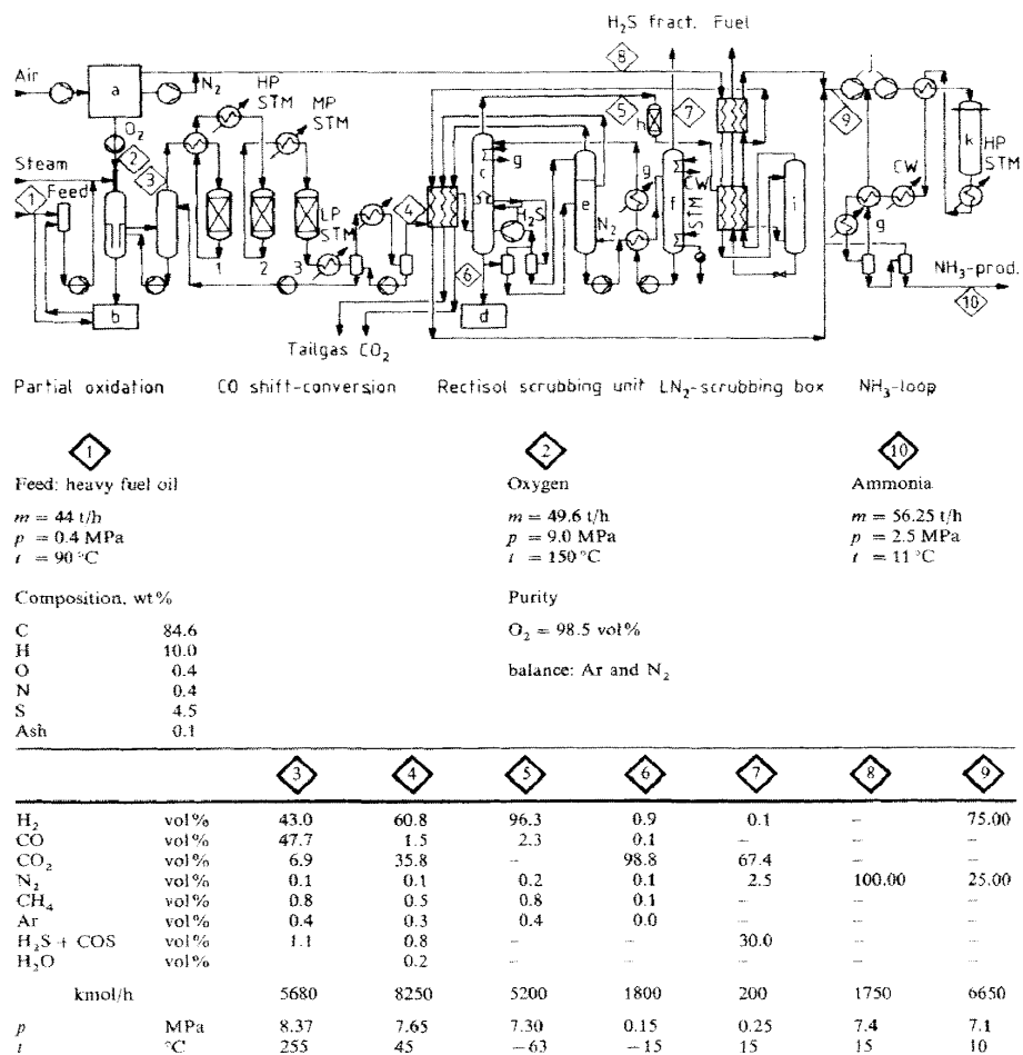
Figure 116. Ammonia production based on heavy fuel oil (Linde flow scheme with Texaco gasification) a) Air separation unit; b) Soot extraction; c) CO 2 absorption; d) Methanol/H 2 O distillation; e) Stripper; f) Hot regenerator; g) Refrigerant; h) Dryer; i) Liquid N 2 scrubber; j) Syngas compressor; k) NH 3 reactor Material Balance
