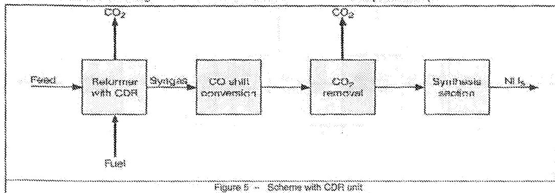
Figure 5 -- Scheme with CDR unit
