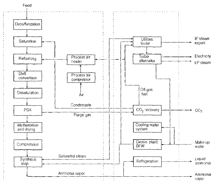
Figure 112. Arrangement of core units and utility section
