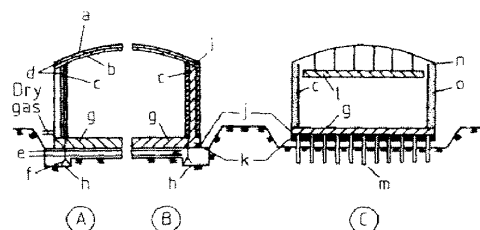
Figure 119. Arrangements of refrigerated ammonia tanks
