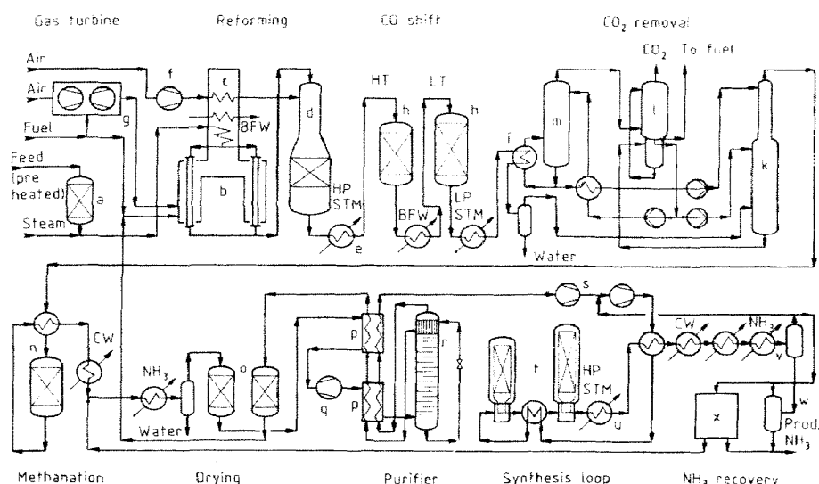
Figure 109. The Braun purifier ammonia process
