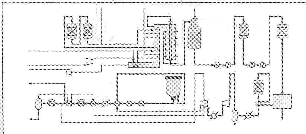
Figure 1 – Process flow diagram for Topsøe ammonia plant
