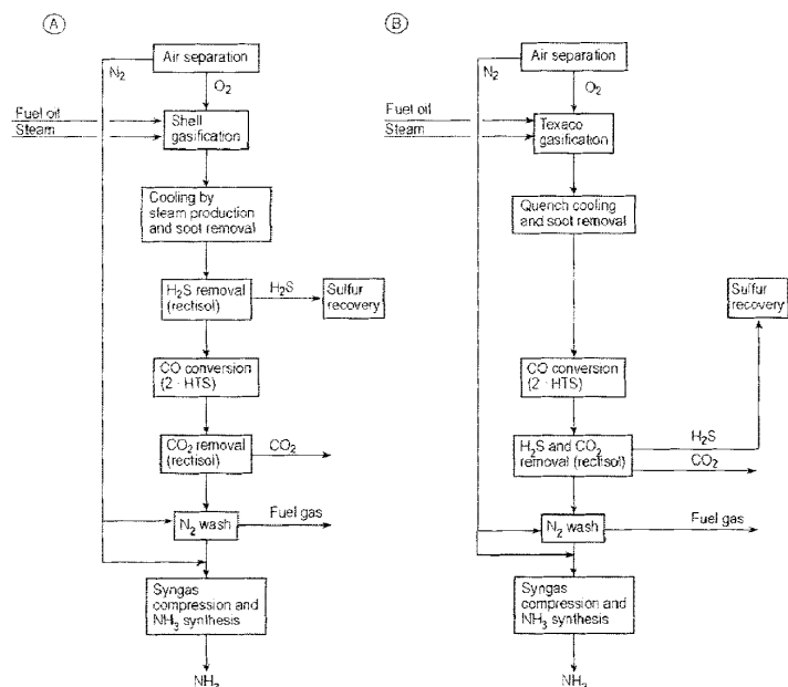
Figure 115. Flow diagrams of ammonia production from fuel oil or heavy residues by the Shell (A) and the Texaco (B) process (standard configuration)
