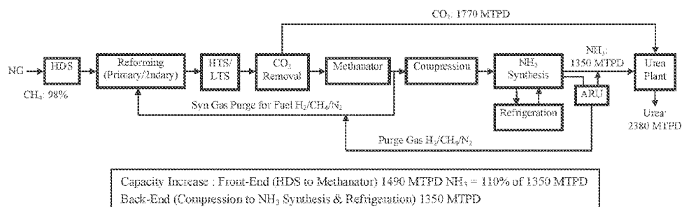
Figure 4. Larger Front-End Capacity Case
