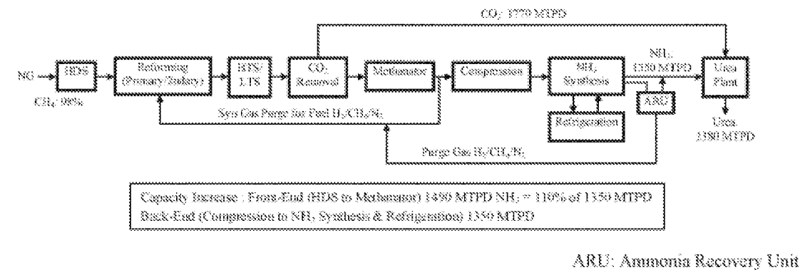
Figure 4. Larger Front-End Capacity Case
