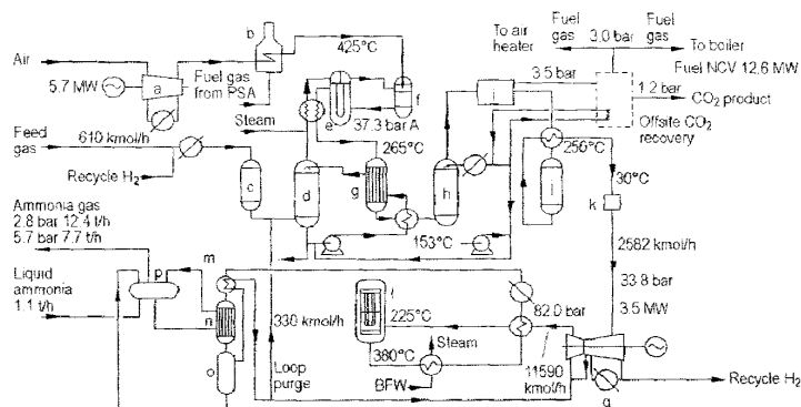
Figure 111. ICI LCA process (core unit)
