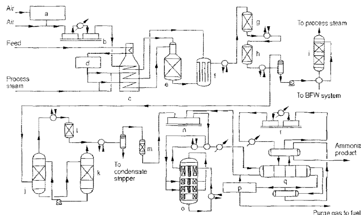
Figure 113. Kellogg's Ammonia 2000 process (integrated KRES/KAAP process) a) Air separation unit; b) Air compressor; c) Process heater; d) Sulfur removal; e) Autothermal reformer; f) Reforming exchanger; g) HTS; h) LTS; i) Condensate stripper; j) CO 2 absorber; k) CO 2 stripper; l) Methanator; m) Dryer; n) Synthesis gas compressor; o) KAAP ammonia converter; p) Purge gas recovery unit; q) Refrigeration exchanger; r) Refrigeration compressor
