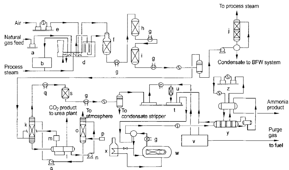
Figure 107. M. W. Kellogg's low energy process
