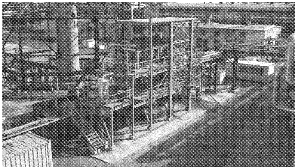
Fig. 6: View of the ATR test facility ready for startup
