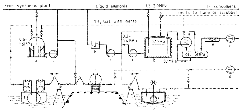
Figure 118. Ammonia terminal with loading and unloading facilities
