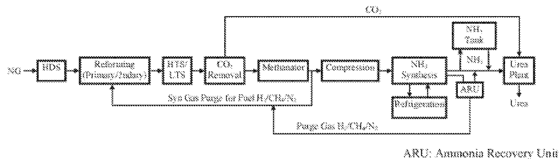
Figure 1. Conventional Ammonia Plant
