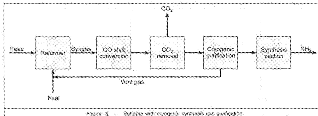
Figure 3 -- Scheme with cryogenic synthesis gas purification
