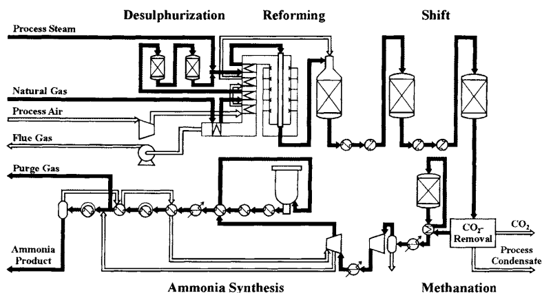
Figure 51 Complete ammonia plant [108]
