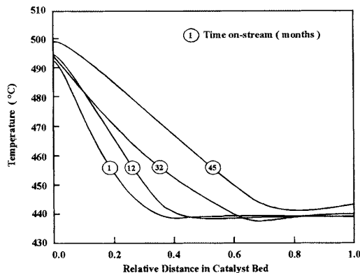
Figure 10 Temperature profile of an adiabatic prereformer with natural gas feed in a 1600 MTPD ammonia plant [22]. \text{H}_2\text{O}/\text{C}=2.8 P=35 bars. The movement of the temperature profile with time is due to catalyst poisoning by sulphur (see Section 2.3.5.2).
