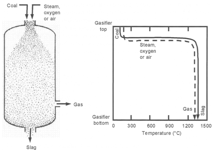
Figure 73 Entrained flow gasifier and typical temperature profile [174].
