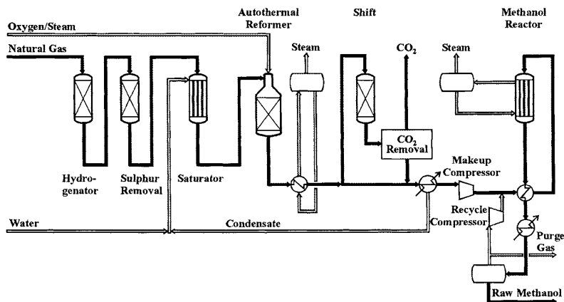
Figure 48 Methanol production by ATR and \text{CO}_2 removal [104].
