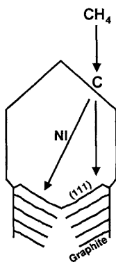
Figure 40 Schematic illustration of the process by which carbon whiskers are formed at the nickel particle during steam reforming.
