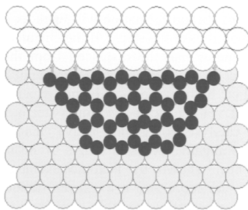
Figure 45 Illustration of a graphene island nucleated from a step on a Ni(111) surface.
