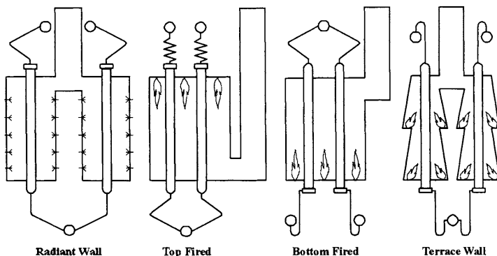
Figure 15 Tube and burner arrangements [4]
