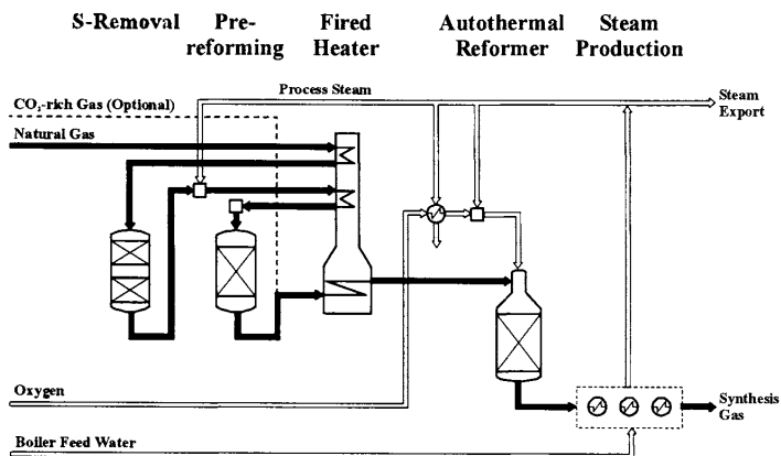
Figure 12 Typical layout of the syngas generation unit with adiabatic prereformer in a GTL plant [26].
