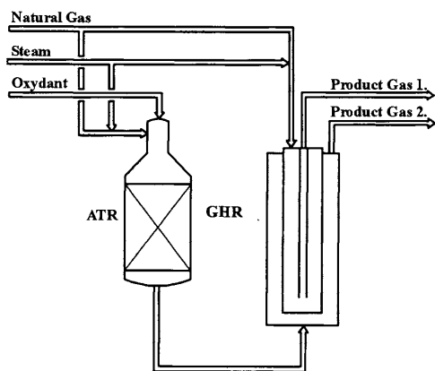
Figure 34 Autothermal reformer (ATR) and Gas Heated Reformer ('Two-in, two-out', GHR) in parallel arrangement
