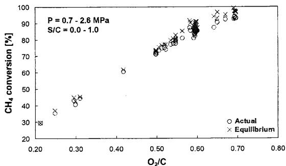
Figure 63 Methane conversion in CPO pilot plant experiments with air as oxidant [167]
