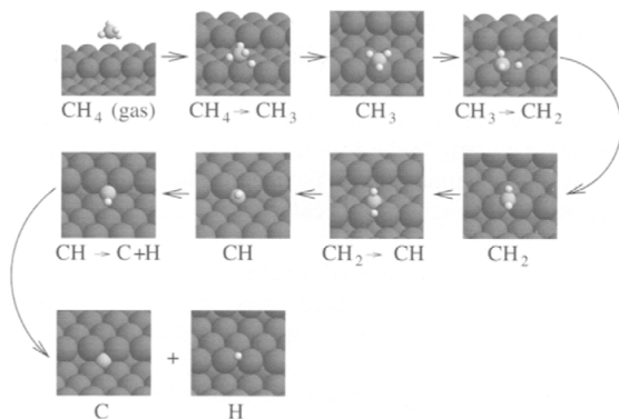
Figure 43 Calculated structures of intermediates and transition states for all elementary processes in the methane activation reactions on the step sites of a Ni(211) surface [89].
