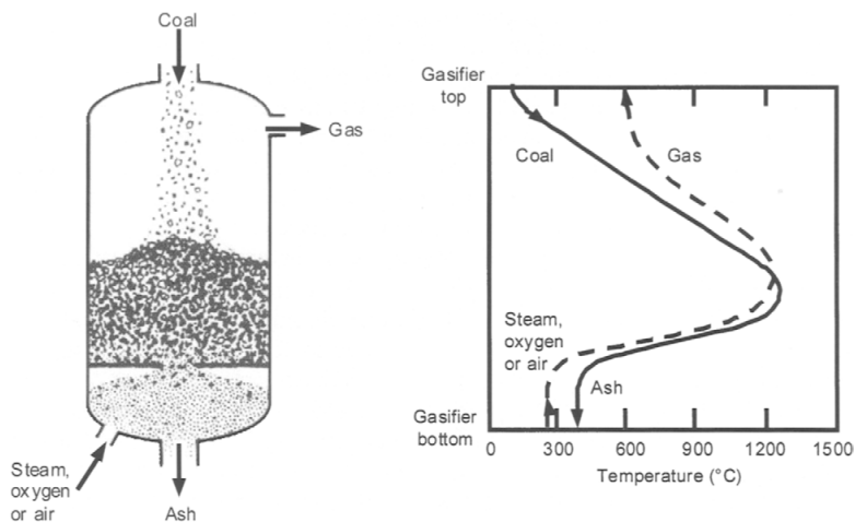
Figure 67 Lurgi dry bottom gasifier and typical temperature profile [174]
