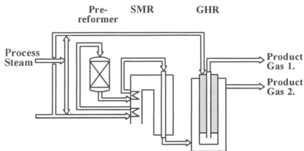
Figure 33 Tubular reformer (SMR) and Gas Heated Reformer ('Two-in, two-out', GHR) in parallel arrangement
