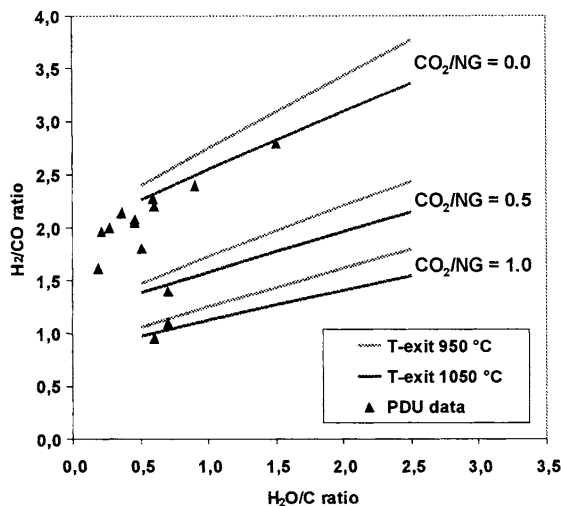
Figure 60 Syngas equilibrium; experimental data from soot-free ATR-operation [155]
