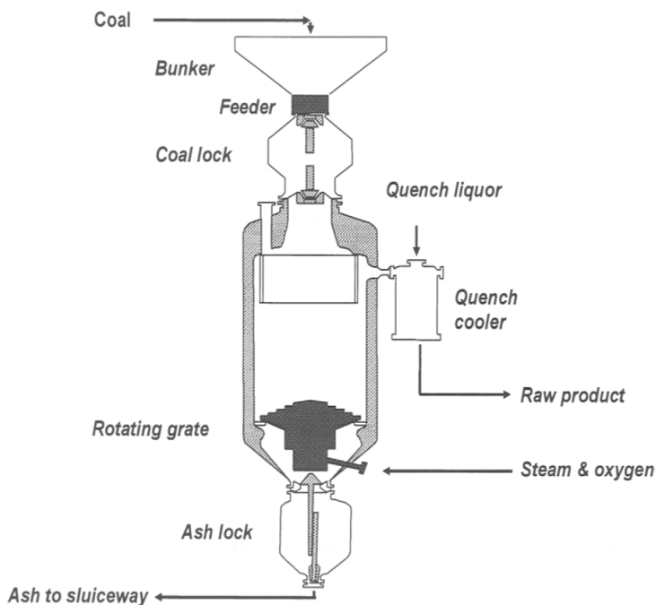
Figure 66 Sasol-Lurgi fixed bed dry bottom gasifier [191]
