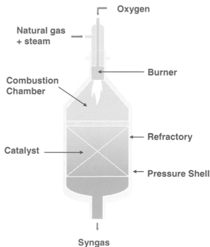
Figure 55 Illustration of an ATR reactor [taken from 132].
