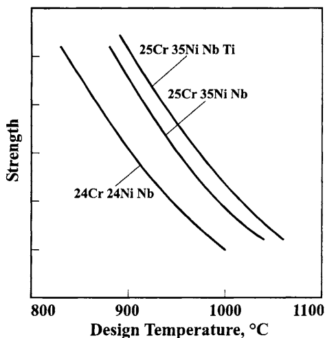
Figure 20 Creep rupture strength for different reformer tube materials [44]
