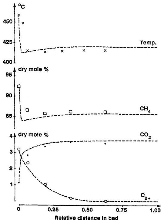
Figure 14 Temperature and conversion profiles for prereforming of natural gas, H_2O/C ratio = 0.40, P = 8 bar. Measured data: x - temperature; □ - CH_4 concentration; • - CO_2 concentration; o - C_{2+} concentration. Calculated profiles are shown as dashed lines. [22].
