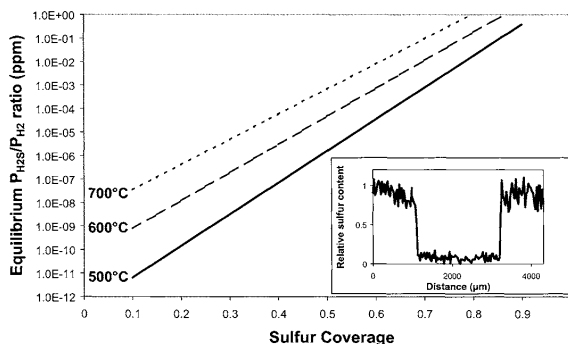
Figure 38 Equilibrium P_{\text{H}_2\text{S}}/P_{\text{H}_2} ratio as a function of the sulphur coverage. The inserted figure gives the sulphur profile in a strongly sulphur poisoned catalyst pellet
