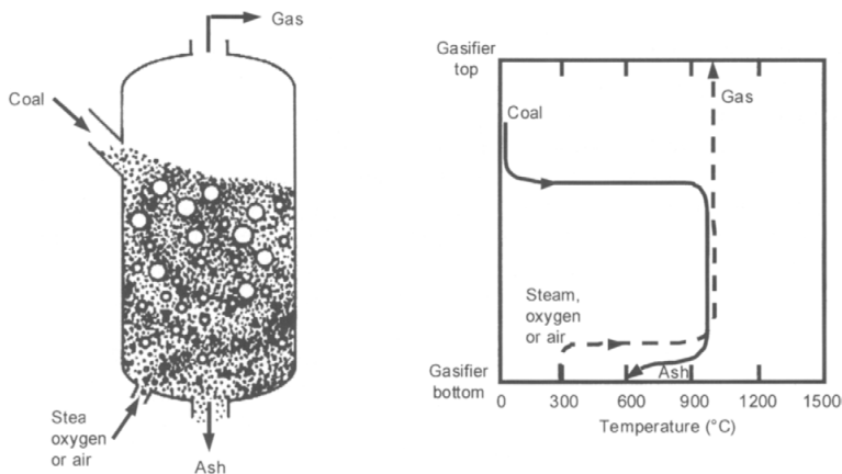
Figure 69 Fluidized bed gasifier and typical temperature profile [174].
