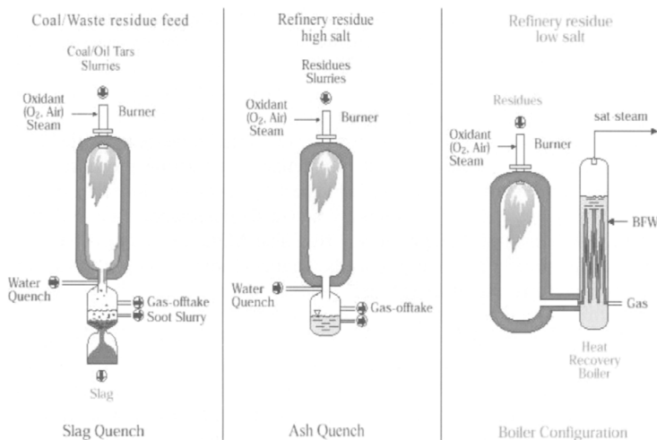
Figure 77 Different modes of operation for a MPG [211]
