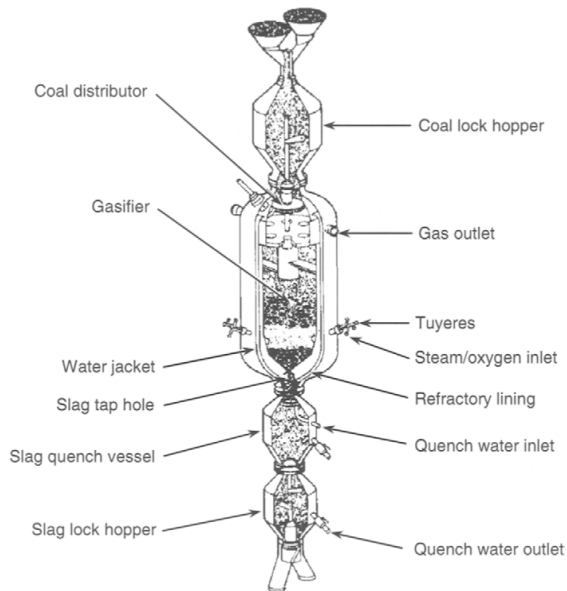
Figure 68 BGL gasifier [174, see also 177]
