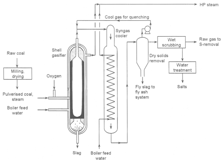
Figure 76 Shell gasifier [218, 219]
