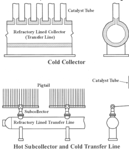
Figure 19 Typical designs of gas outlet systems [4]
