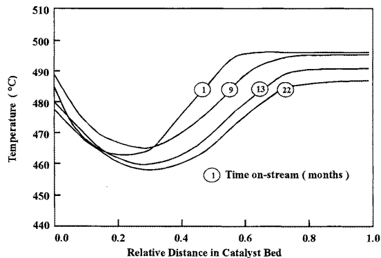
Figure 9 Temperature profile of an adiabatic prereformer with naphtha feed [22]. H_2O/C=3.5 . P=26 bars. The movement of the temperature profile with time is due to catalyst poisoning by sulphur (see Section 2.3.5.2).
