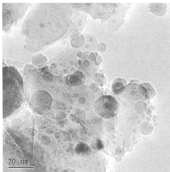
Figure 37 Nickel supported on a \text{MgAl}_2\text{O}_4 spinel carrier. Recorded at 550°C and 7 mbar of hydrogen using the insitu electron microscope at Haldor Topsøe A/S.
