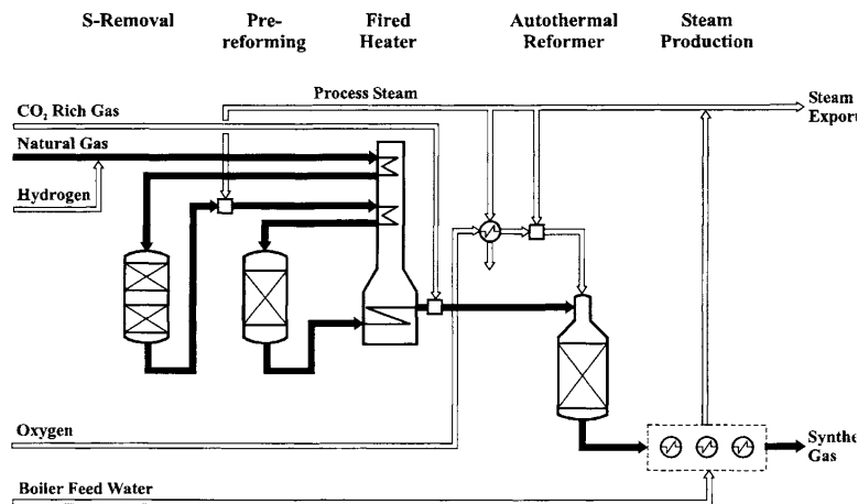
Figure 50 Typical process flow diagram for synthesis gas production for GTL
