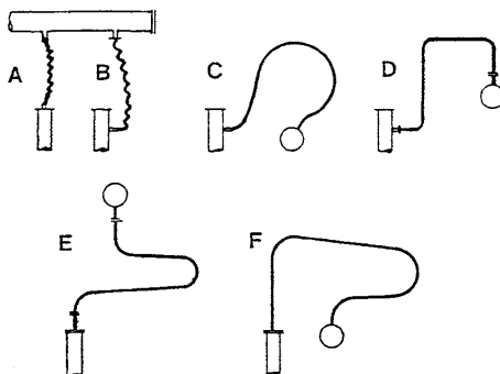
Figure 18 Typical design of gas inlet systems
