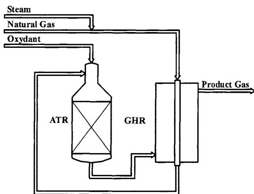
Figure 31 'Two-step reforming with GHR': Autothermal reformer (ATR) and Gas Heated Reformer (GHR) in series arrangement.
