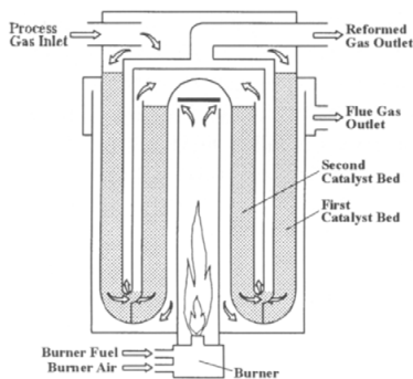
Figure 28 Topsøe Heat Exchange Reformer (HER) [57]
