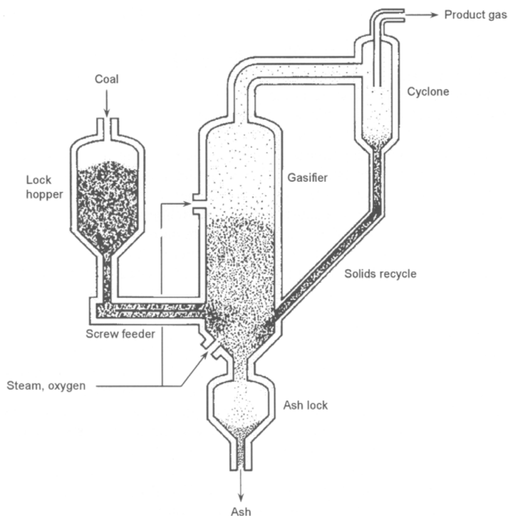
Figure 71 HTW gasifier [174, see also 177]
