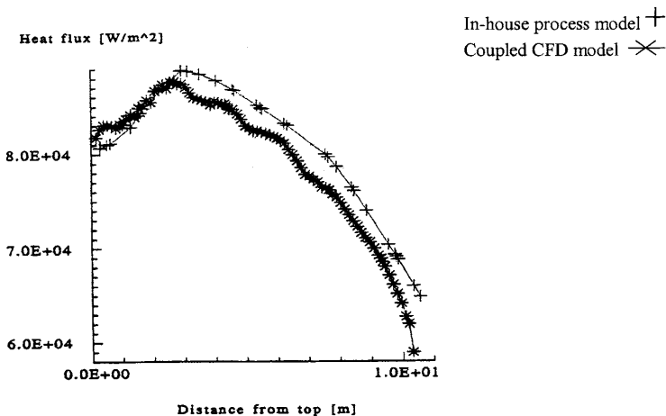
Figure 26 Heat flux calculated by CFD and by in-house process model [56]
