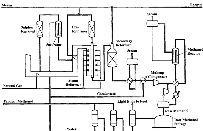
Figure 52 Methanol production by two-step reforming [104].
