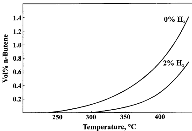
Figure 2 Equilibrium concentration of butene in n-butane at 30 bar g
