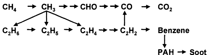
Figure 53 Simplified reaction path for C_1 and C_2 chemistry CH_4 combustion [118].
