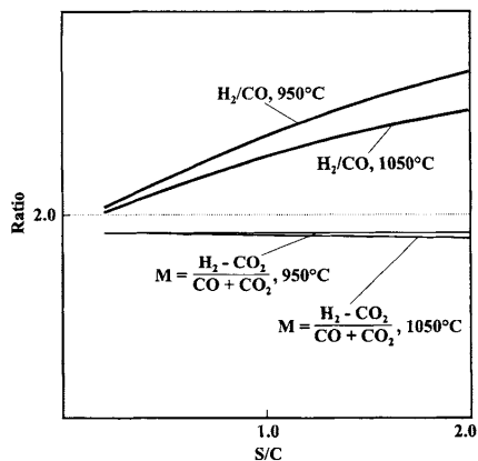
Figure 47 M and H 2 /CO in raw gas from ATR
