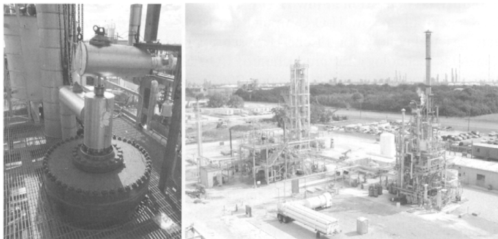
Figure 58 ATR Process Demonstration Unit, Houston, Texas [132]
