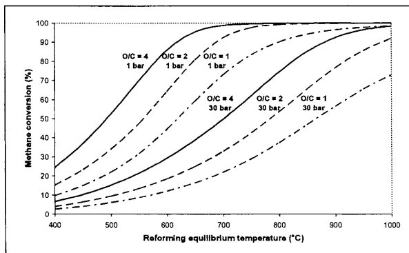
Figure 8 Steam reforming and methane conversion (O/C: ratio of steam to methane in the feed gas).
