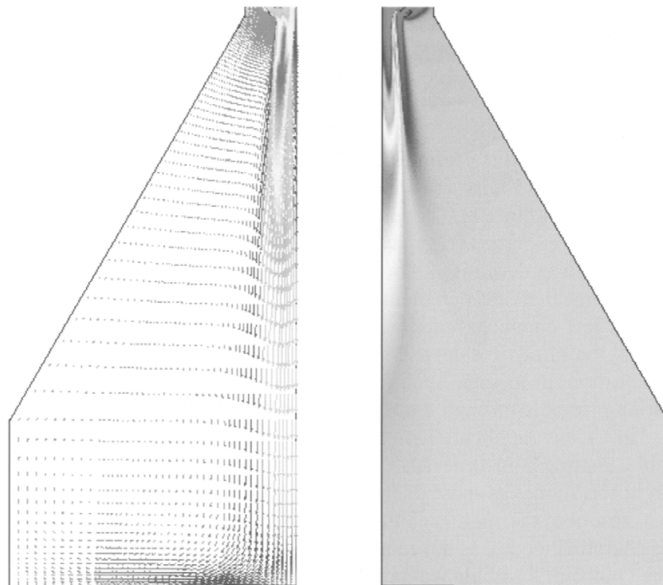
Figure 56 Example of CFD modelling results for the combustion chamber in an ATR reactor. The left part show velocity vectors and the right part show temperatures. [134]
