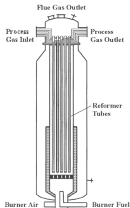
Figure 29 Topsøe Convection Reformer (HPCR) [59]
