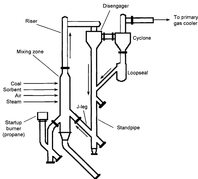
Figure 72 Transport reactor [191]
