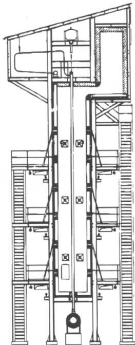
Figure 16 Cross section of side fired reformer
