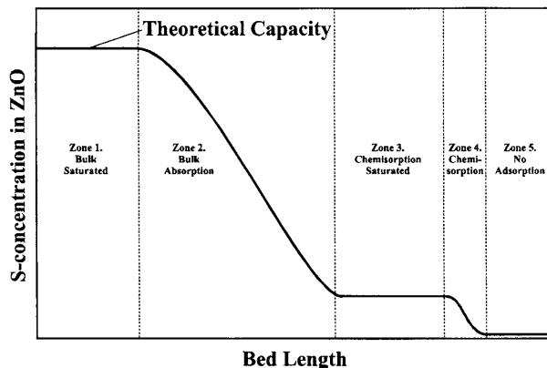
Figure 7 Ideal sulphur profile in a zinc oxide bed
