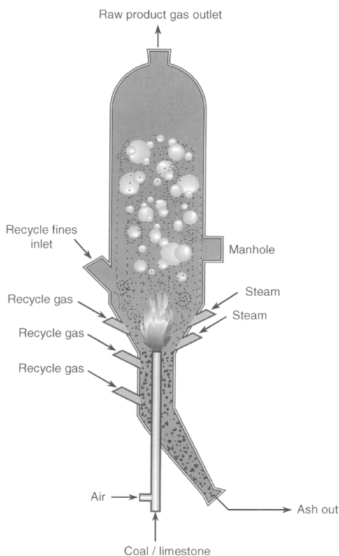
Figure 70 KRW gasifier [192]
