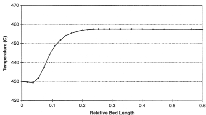
Figure 13 Temperature profile in adiabatic prereformer during pilot plant operation. H_2O/C = 0.4 [26].
