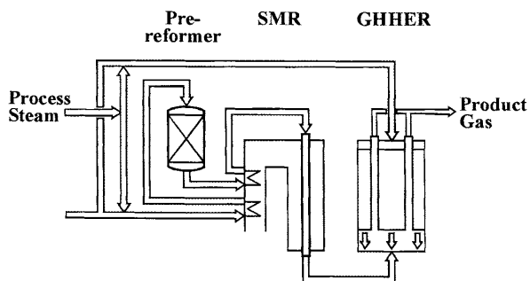
Figure 35 Tubular Reformer (SMR) and Gas Heated Reformer ('two-in, one-out', GHHER) in parallel arrangement
