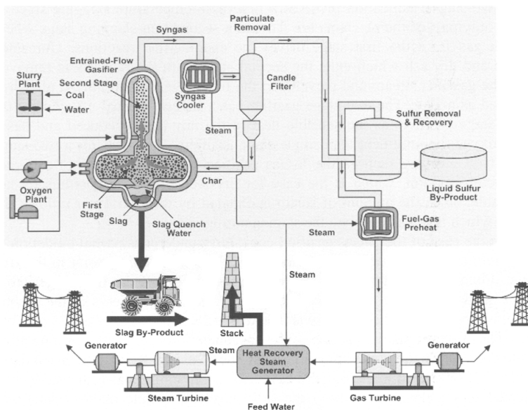
Figure 78 Wabash River Coal Gasification Repowering plant [215]
