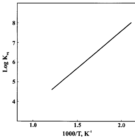
Figure 4 Equilibrium constant for reaction (11)
