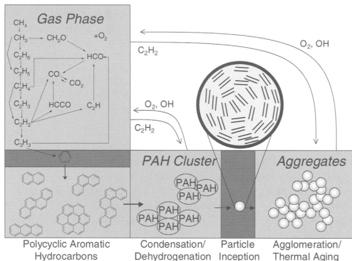
Figure 54 Schematic representation of reaction steps involved in the soot formation in methane combustion, taken from [128].
