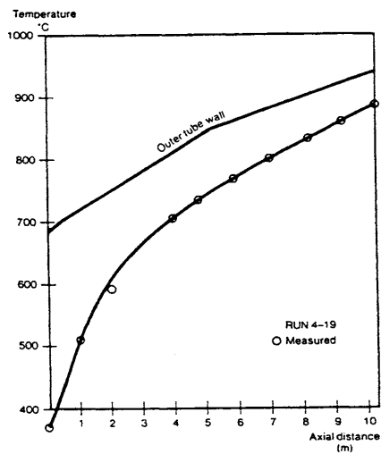
Figure 22 Measured and calculated axial temperature profiles from run in PDU [51]
