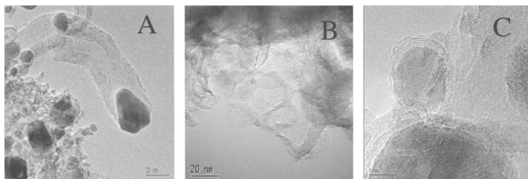
Figure 39 Electron microscopy pictures of whisker carbon (a), pyrolytic carbon on a ceramic carrier b), and encapsulating carbon (c). C_nH_m : Higher hydrocarbons (hydrocarbons with two or more carbon atoms)
