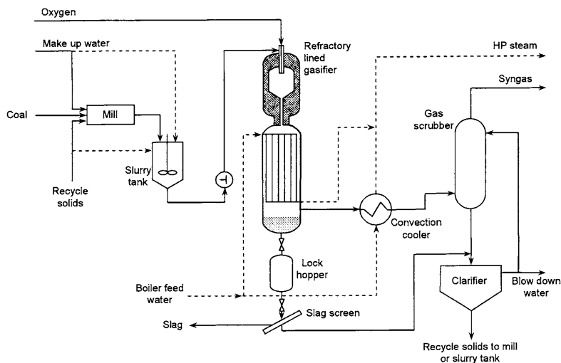
Figure 75 Texaco gasifier with radiant cooling [1].
