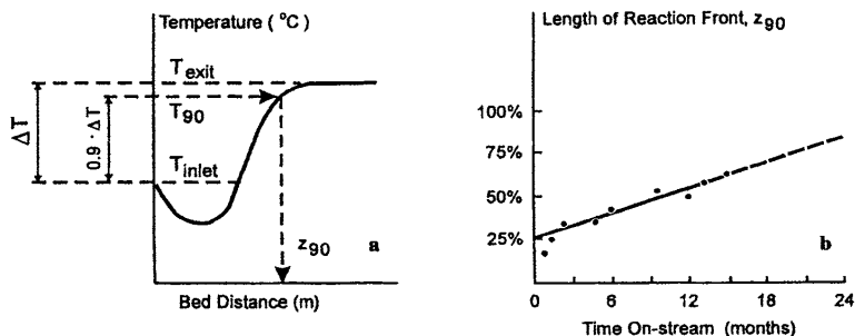
Figure 11 Graphical deactivation plot for performance prediction [25].
