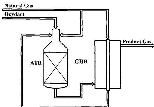
Figure 32 'Combined Reforming with GHR': Autothermal reformer (ATR) and Gas Heated Reformer (GHR) in series arrangement with partial by-pass of feed over the GHR.
