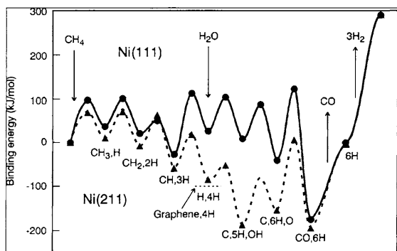
Figure 44 Calculated energies along the reaction path for steam reforming on the Ni(111) and Ni(211) surfaces. The corresponding structures are shown in Figs. 42 and 43. All energies are given relative to a situation in which all reactants are in the gas phase far from the clean surface [89].
