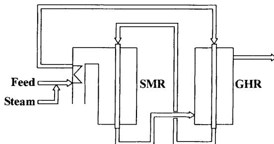
Figure 30 'Gas Heated Prereforming': Fired tubular reforming (SMR) and Gas Heated Reformer (GHR) in series arrangement
