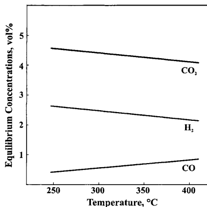
Figure 6 Equilibrium concentrations of CO , CO_2 , and H_2 ; 3% H_2 and 5% CO_2 in the feed
