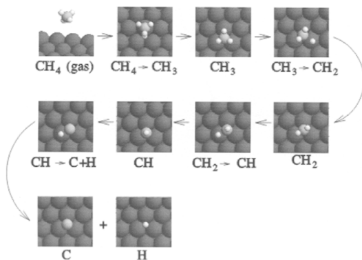
Figure 42 Calculated structures of intermediates and transition states for all elementary processes in the transformation of methane into adsorbed carbon and hydrogen on a Ni(111) surface [89].
