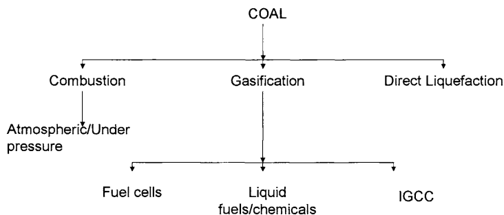
Figure 65 Different options for coal conversion and power generation. [175]
