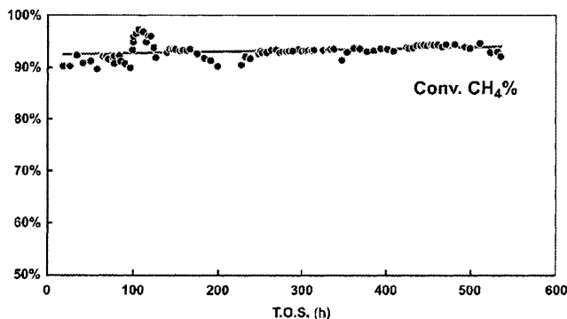
Figure 62 CPO with methane feed and oxygen as oxidant [161]. P=1.5 Mpa. H_2O/CH_4=0.26 ; CO_2/CH_4=0.11 ; O_2/CH_4=0.56
