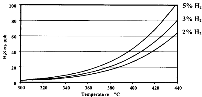
Figure 5 Equilibrium \text{H}_2\text{S} , 5% \text{CO}_2 in natural gas
