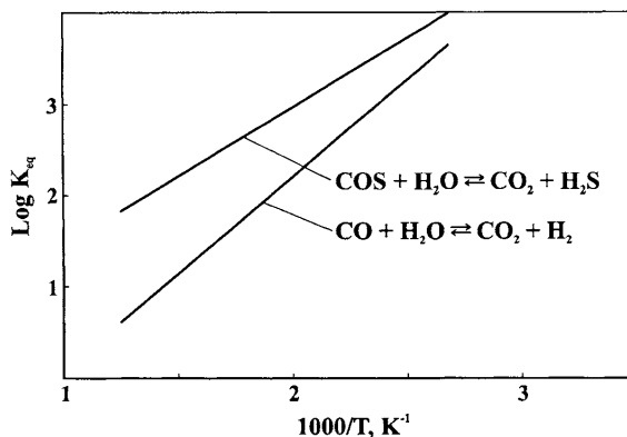
Figure 3 Equilibrium constants for COS hydrolysis and the shift reaction
