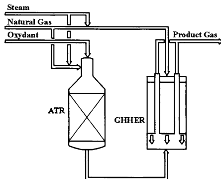
Figure 36 Autothermal Reformer (ATR) and Gas Heated Reformer ('two-in, one-out', GHER) in parallel arrangement
