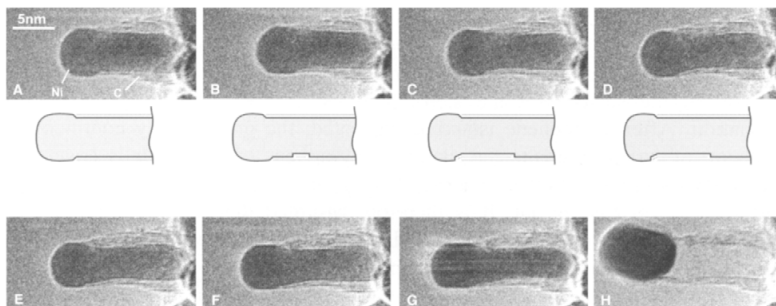
Figure 46 Image sequence of the initial carbon formation on a Ni/MgAl 2 O 4 catalyst. Drawings are included to guide the eye in locating the positions of mono-atomic Ni step edges at the C-Ni interface. The images are acquired in situ with CH 4 :H 2 = 1:1 at a total pressure of 2.1mbar with the sample heated to 536°C.
