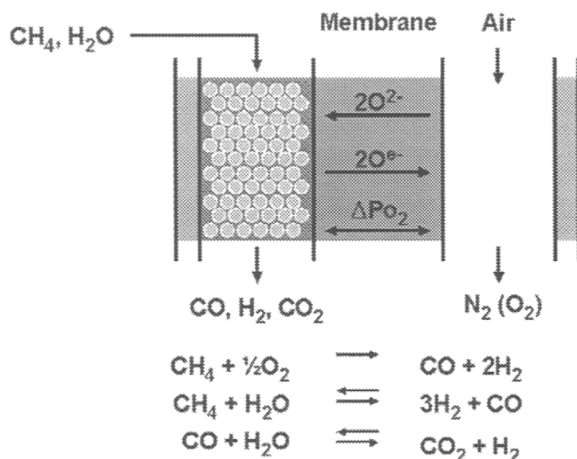
Figure 64 Principle of oxygen membrane reforming
