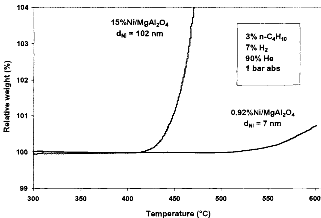
Figure 41 Relative weight increase as a function of the temperature for two catalysts with different nickel crystal size but the same nickel surface area and reforming activity
