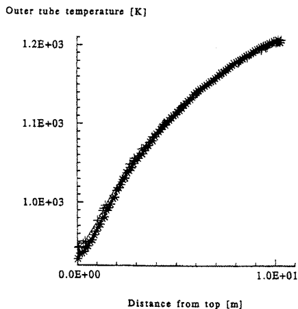
Figure 25 Calculated and measured outer tube wall temperature Measured Outer Tube Wall Temperature [56]
