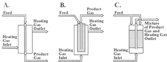
Figure 27 A: Concept with 'straight-through' tubes; B: Concept with bayonet tubes; C: Concept with mixing of heating gas and product gas before heat exchange.
