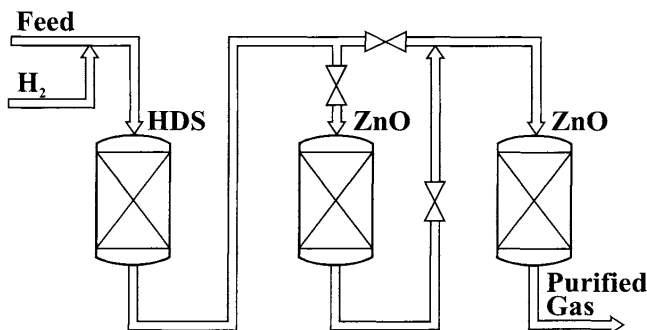
Figure 1 Typical process flow diagram for desulphurisation of natural gas
