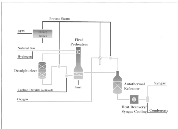
Figure 59 Process layout of ATR Process Demonstration Unit
