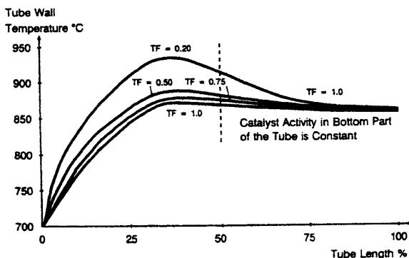
Figure 24 Tube wall temperatures in top fired reformer at various catalyst activity levels (TF) in the upper 50% of the tube.
