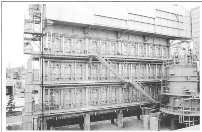
Figure 17 Photo of Topsøe Reformer [34]
