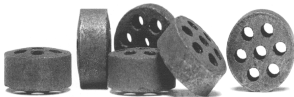
Figure 23 Steam reforming catalyst. Topsøe R-67 R-7H.
