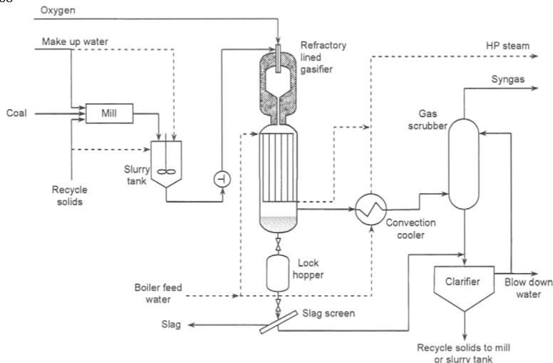
Figure 74 Texaco gasifier with quench cooling[1]
