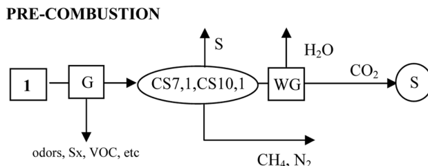
Figure 18. Pre-combustion approach for capture and concentration of CO 2 in the natural, coal and landfill gas industries for stream 1 defined in Figs. 7 and 10. The short-hand notation used here appears as CS#, # or CS#-#, #. CS stands for a CO 2 separation step. The first number (#) corresponds to a figure number (or figure numbers as indicated by #-#). This number (or numbers) corresponds to one (or more) of the CO 2 producing flowsheets depicted in Figs. 1 to 11. The second number (#) after the comma represents the proposed CO 2 separation step that is indicated within the boxed region labeled with the corresponding Roman numeral. G refers to a guard step, WG refers to a guard step particular for water, CS7,1 and CS10,1 refer to a CO 2 separation step appropriate for the process in Figs. 7 and 10, respectively, and S refers to the final CO 2 sequestration step. This final CO 2 stream is H 2 O free but may contain small amounts of N 2 , CH 4 , and H 2 S. At the CO 2 separation step, the stream contains CO 2 , N 2 and H 2 S as main gas components. Depending on the CO 2 and H 2 S concentrations, Fig. 23 provides alternative processes for the CO 2 separation step CS7,1 and CS10,1.
