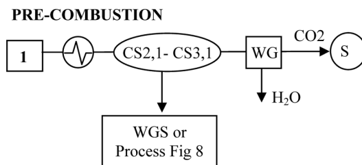
Figure 14. Pre-combustion approaches for the capture and concentration of CO 2 in the coal gasification industry for stream 1 in Figs. 2 and 3. The short-hand notation used here appears as CS#,# or CS#-#,#. CS stands for a CO 2 separation step. The first number (#) corresponds to a figure number (or figure numbers as indicated by #-#). This number (or numbers) corresponds to one (or more) of the CO 2 producing flowsheets depicted in Figs. 1 to 11. The second number (#) after the comma represents the proposed CO 2 separation step that is indicated within the boxed region labeled with the corresponding Roman numeral. WG refers to a guard step particular for water, WGS refers to a water gas shift step, CS2,1 and CS3,1 refer to a CO 2 separation step appropriate for the process in Figs. 5 and 6, respectively, and S refers to the final CO 2 sequestration step. This final CO 2 stream is H 2 O free but may contain small amounts CH 4 , CO and H 2 . At the CO 2 separation steps, boxed flow sheets I and II contain CO 2 , CO, H 2 , and CH 4 as main gas components. Depending on the CO 2 concentration, Fig. 19 provides detailed alternative processes for the CO 2 separation steps CS2,1 and CS3,1.
