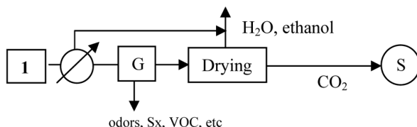
Figure 20. Post-combustion approach for capture and concentration of CO 2 in the ethanol production industry for stream 1 defined in Fig. 11. The short-hand notation used here appears as CS#, # or CS#-#, #. CS stands for a CO 2 separation step. The first number (#) corresponds to a figure number (or figure numbers as indicated by #-#). This number (or numbers) corresponds to one (or more) of the CO 2 producing flowsheets depicted in Figs. 1 to 11. The second number (#) after the comma represents the proposed CO 2 separation step that is indicated within the boxed region labeled with the corresponding Roman numeral. G refers to a guard step and S refers to the final CO 2 sequestration step. This final CO 2 stream is H 2 O free but may contain small amounts of N 2 . No particular action is taken over stream 1 other than a drying step.
