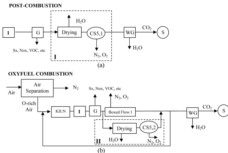
Figure 16. Post-combustion and oxyfuel-combustion approaches for capture and concentration of CO 2 in the cement and lime industry for stream 1 defined in Fig. 5. The short-hand notation used here appears as CS#,# or CS#-#,#. CS stands for a CO 2 separation step. The first number (#) corresponds to a figure number (or figure numbers as indicated by #-#). This number (or numbers) corresponds to one (or more) of the CO 2 producing flowsheets depicted in Figs. 1 to 11. The second number (#) after the comma represents the proposed CO 2 separation step that is indicated within the boxed region labeled with the corresponding Roman numeral. G refers to a guard step, WG refers to a guard step particular for water, CS5,1 and CS5,2 refer to CO 2 separation steps appropriate to boxed flow sheets I and II, respectively, and S refers to the final CO 2 sequestration step. This final CO 2 stream is H 2 O free but may contain small amounts of N 2 , CH 4 , H 2 S, O 2 , and SO 2 . At the CO 2 separation steps, boxed flow sheets I and II contain CO 2 and N 2 as main gas components. Boxed flow sheet I is rich in N 2 , while boxed flow sheet II is lean in this gas species. Depending on the CO 2 concentration, Fig. 21 provides alternative processes for the CO 2 separation steps CS5,1 and CS5,2.
