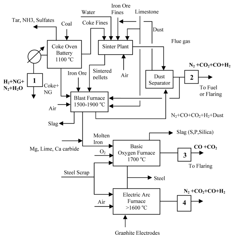
Figure 4. Flow sheet of a typical, state-of-the-art, stainless steel production plant consisting of a coke oven, sinter plant, blast furnace, basic oxygen furnace (BOF) and electric arc furnace (EAF). \text{CO}_2 and \text{CO} are produced out of the burning of methane, coal-coke and carbon removal from pig iron through all steps. The compositions of the numbered streams are shown in Table 12.
