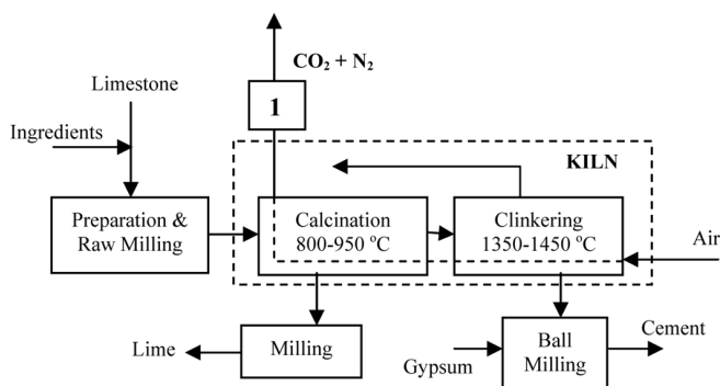
Figure 5. Flow sheet of a typical, state-of-the-art, process for the manufacture of lime and cement. After a preparation and raw milling step, lime is produced through calcination within a kiln. Cement is produced in a further clinkering step and much more elevated temperatures. CO 2 is produced from the decomposition of carbonates and burning of kiln fuel. Final products are obtained following fine milling steps. The composition of the numbered stream is shown in Table 12.
