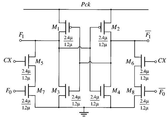
Fig. 1. CAL inverter.
