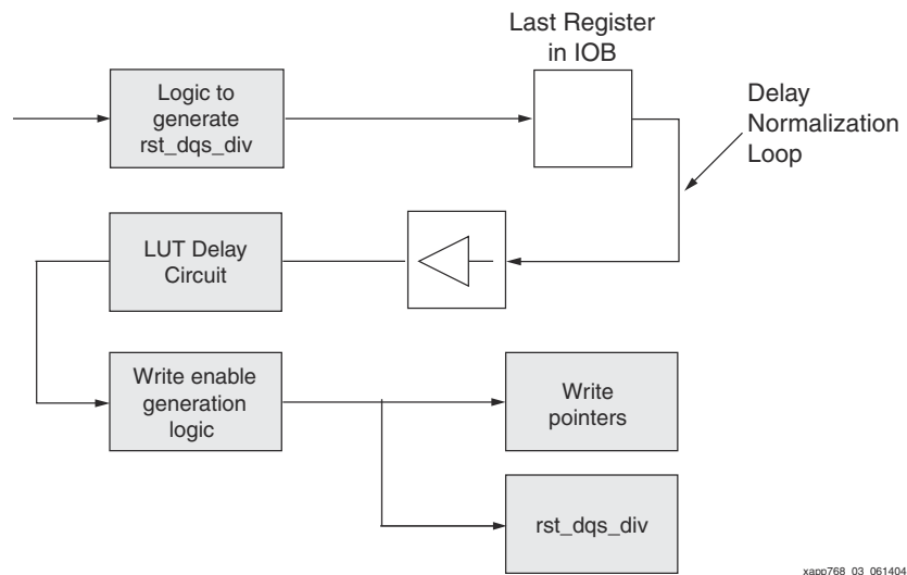
Figure 3: Rst_dqs_div Circuit
