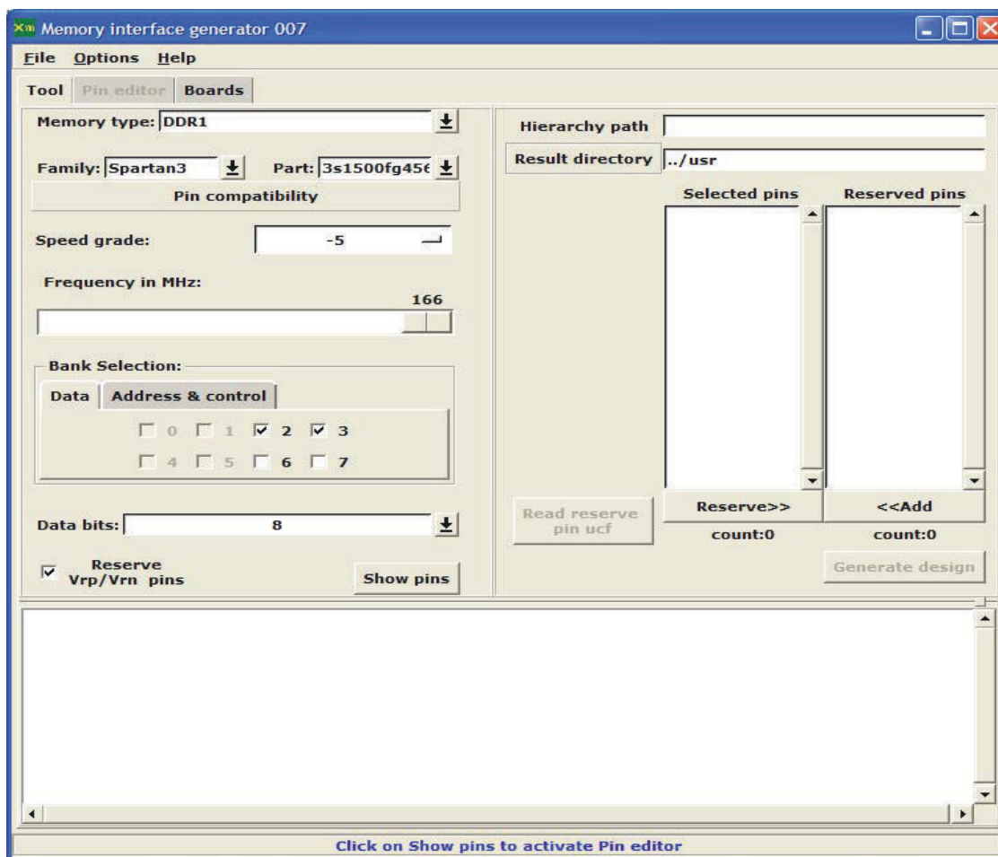
Figure 9: MIG 007 Tool
