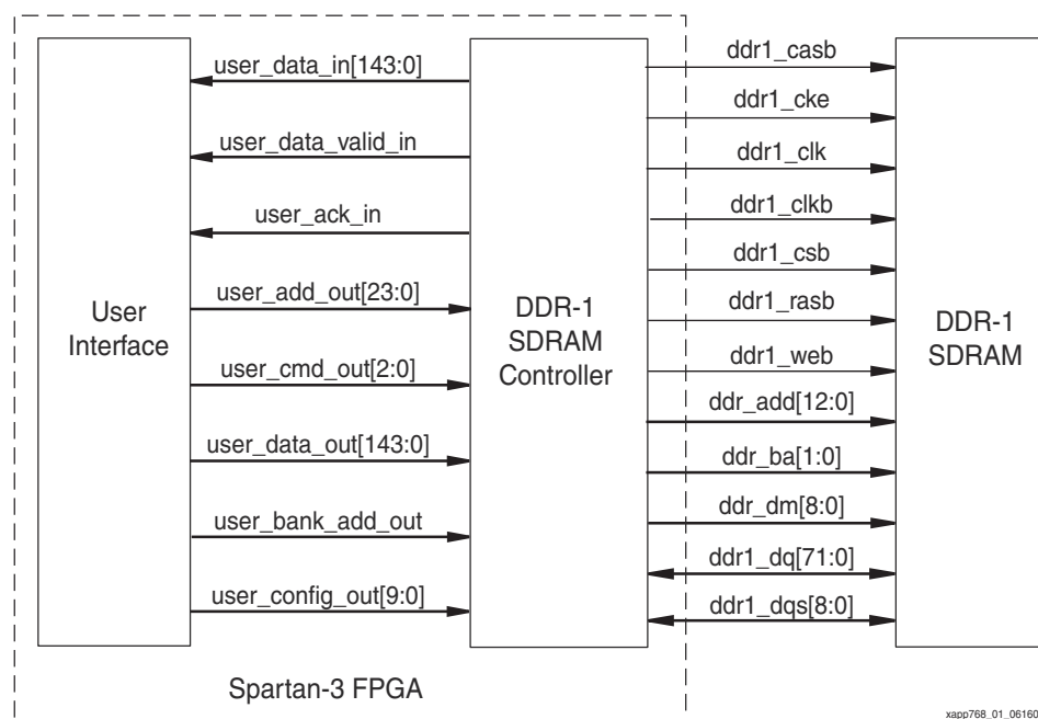
Figure 1: System Diagram
