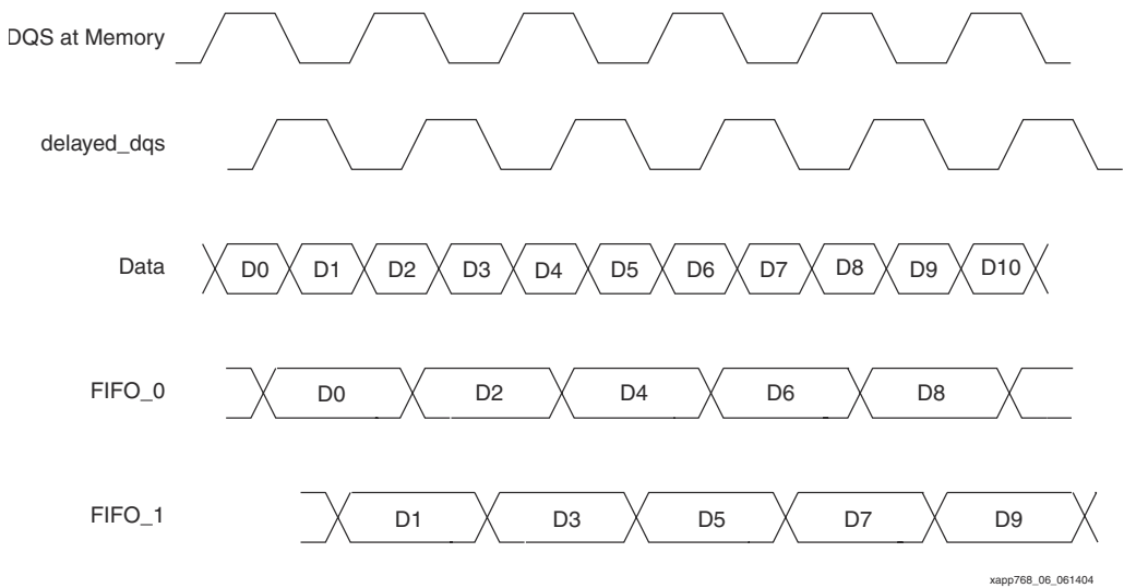
Figure 6: Read Data Timing Diagram
