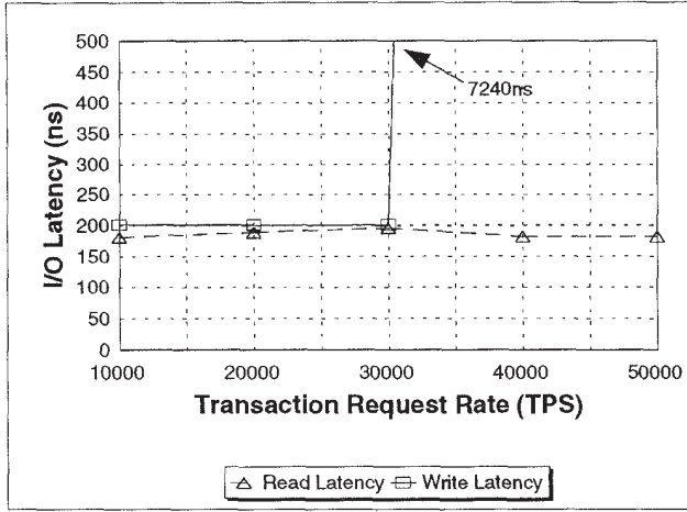
Figure 15: I/O Latency for Increasing Request Rates
