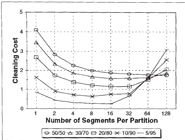
Figure 9: Cleaning Costs vs. Partition Size
