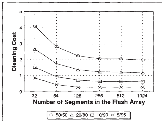
Figure 10: Cleaning Costs vs. Number of Segments
