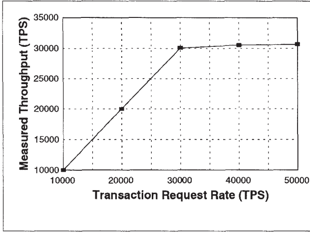
Figure 13: Throughput for Increasing Request Rates
