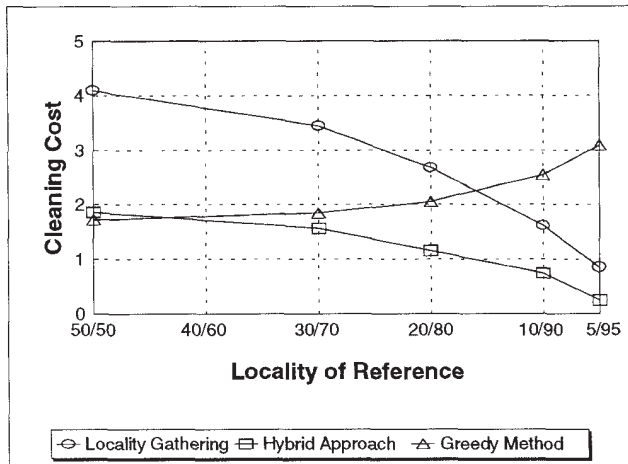
Figure 8: Comparison of Cleaning Algorithms
